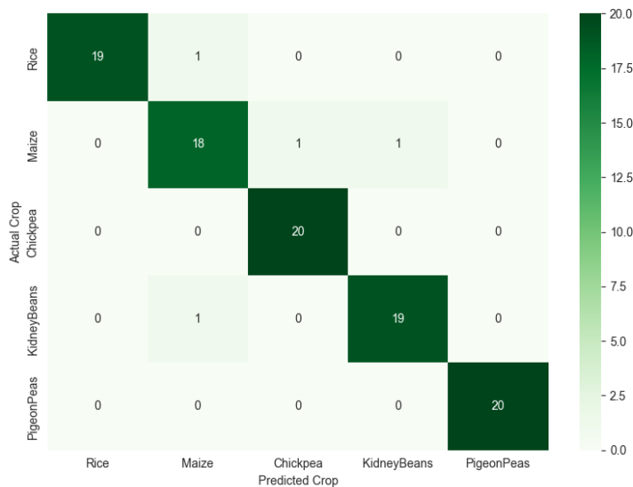
Figure 4. Confusion Matrix (Model Performance)
