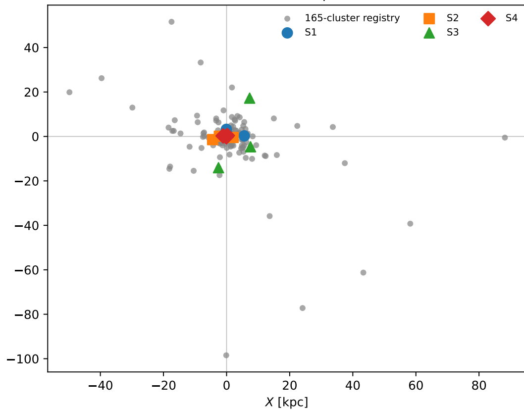
Galactocentric plane
