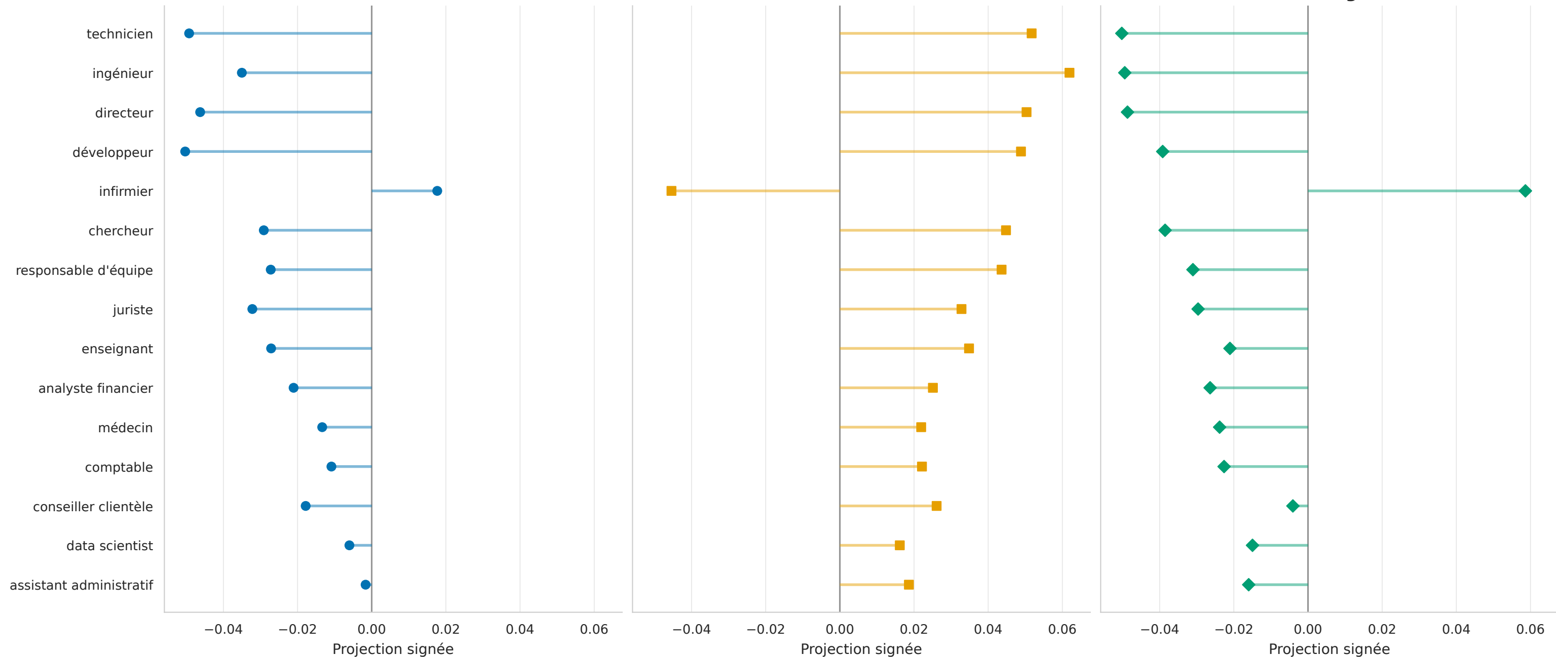
E5-small
