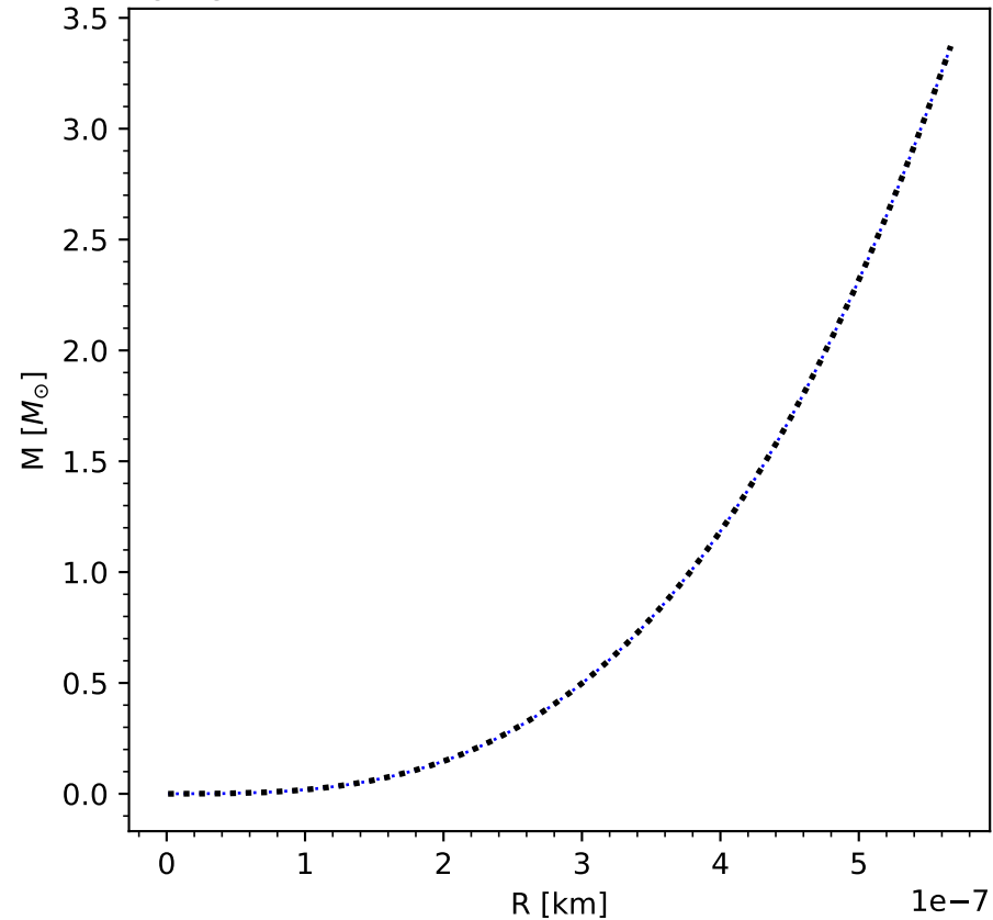
Mass-Radius of a pure neutron star
