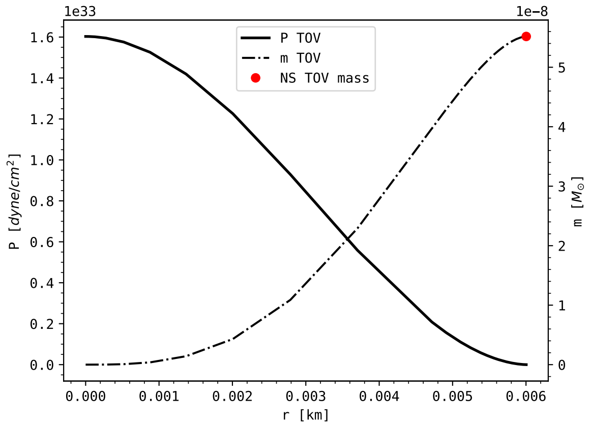
P(r) & m(r) of a pure neutron star in the non-relativistic case ( \gamma=2.5 )
