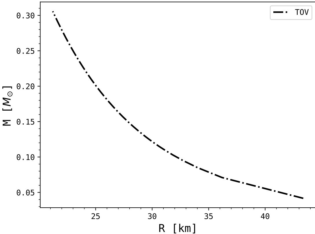
Mass-Radius of a pure non relativistic NS
