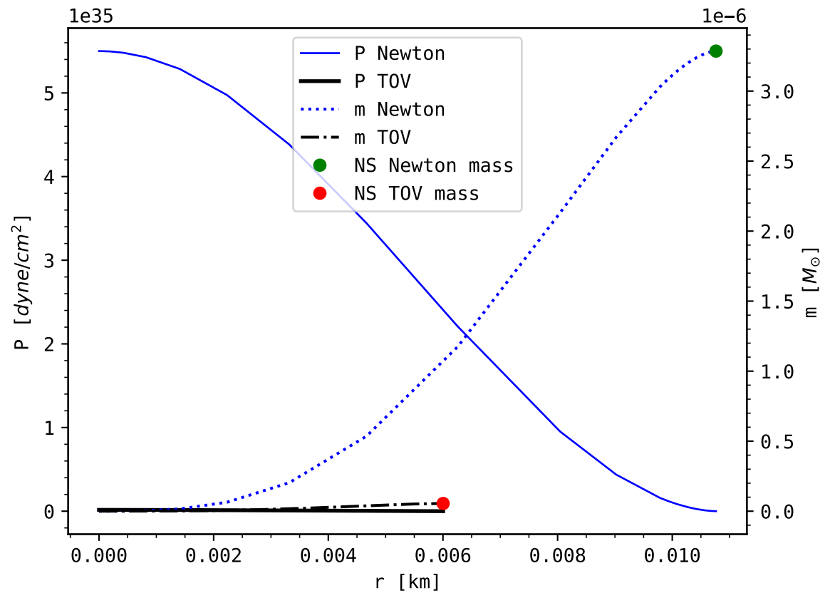
P(r) & m(r) of a pure neutron star in the full relativistic case (gamma=2.0)
