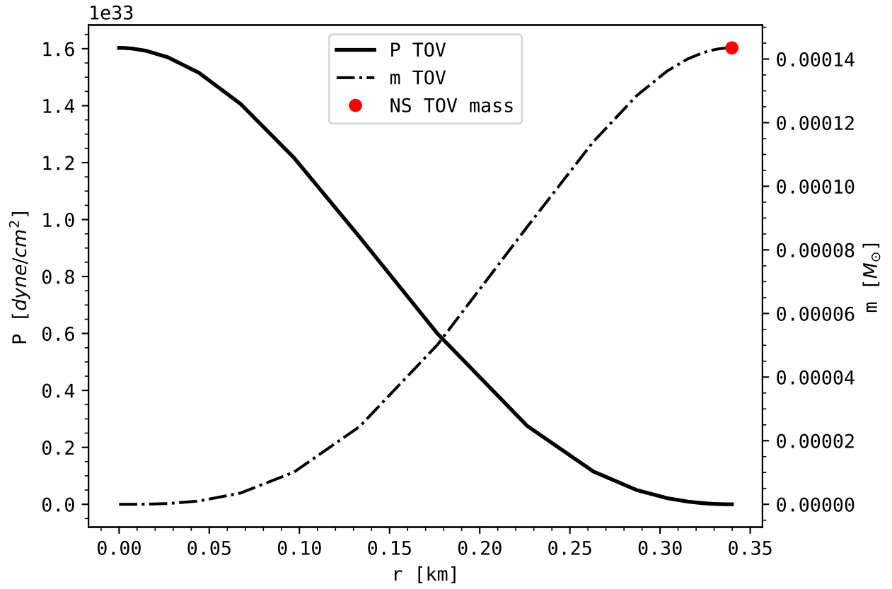
P(r) & m(r) of a pure neutron star in the non-relativistic case ( \gamma=2.0 )
