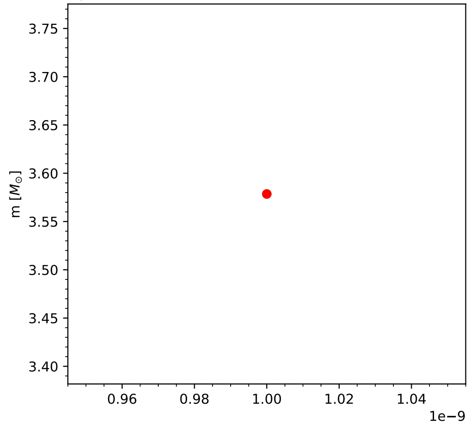
m(r) of a pure neutron star
