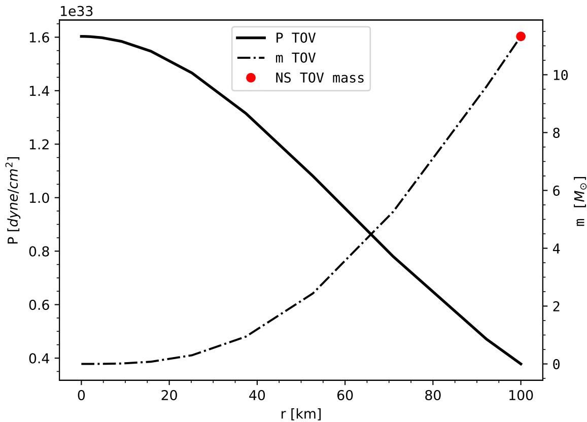
P(r) & m(r) of a pure neutron star in the non-relativistic case ( \gamma=1.5 )
