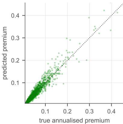
(c) R^2 0.91
