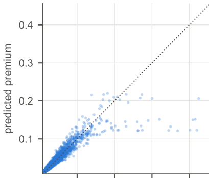
(a) R^2 0.74
