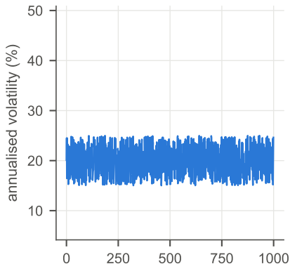
(a) i.i.d. sigma
