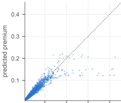
(a) R^2 0.74
