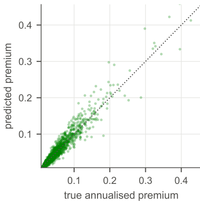
(c) R^2 0.91
