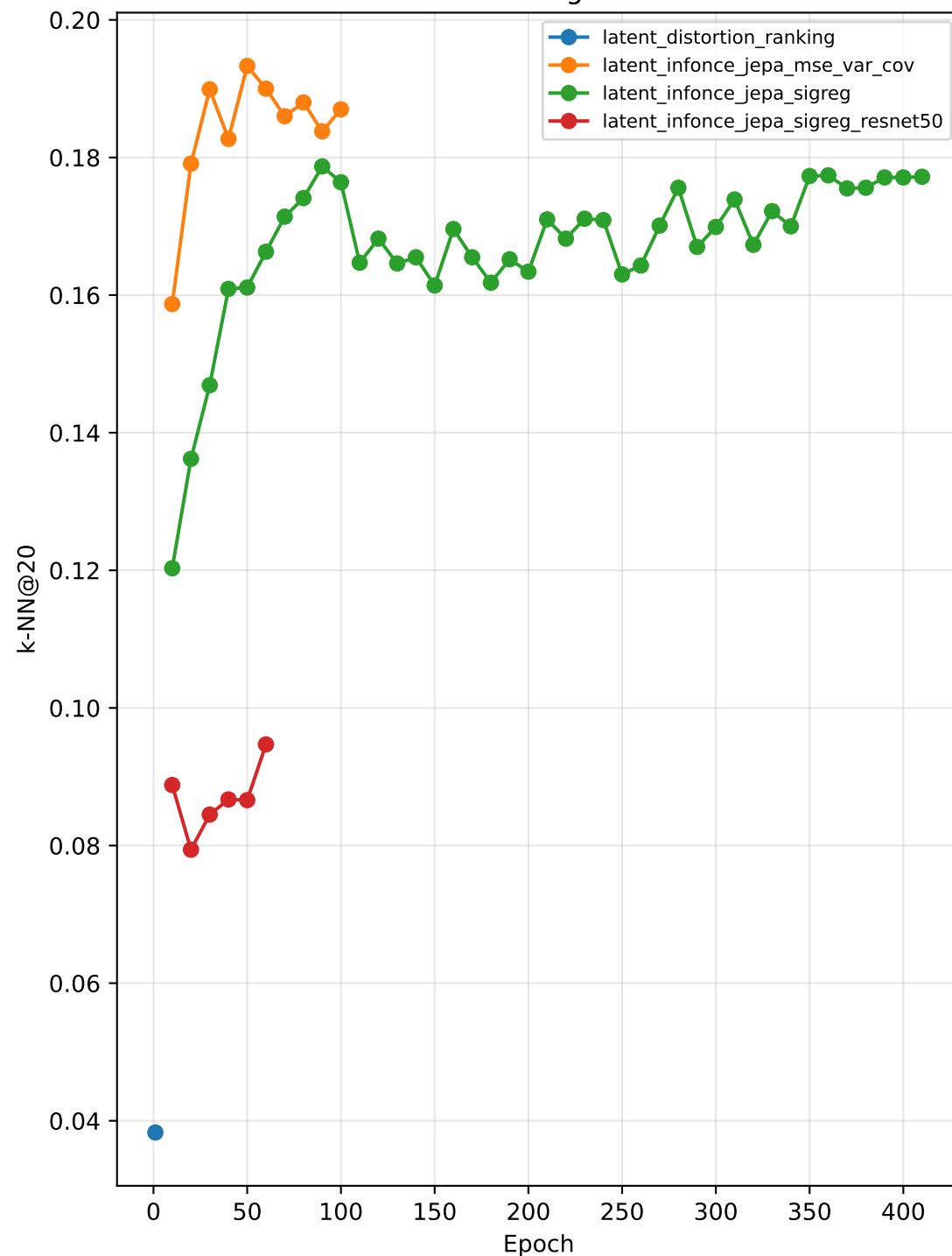
k-NN learning curves
