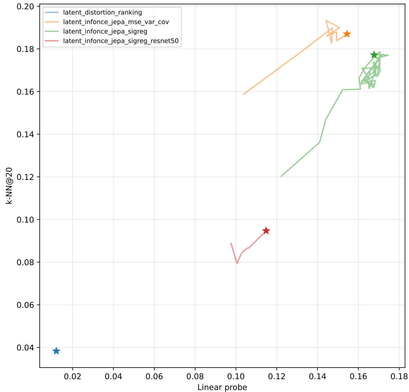
k-NN vs Linear trade-off
