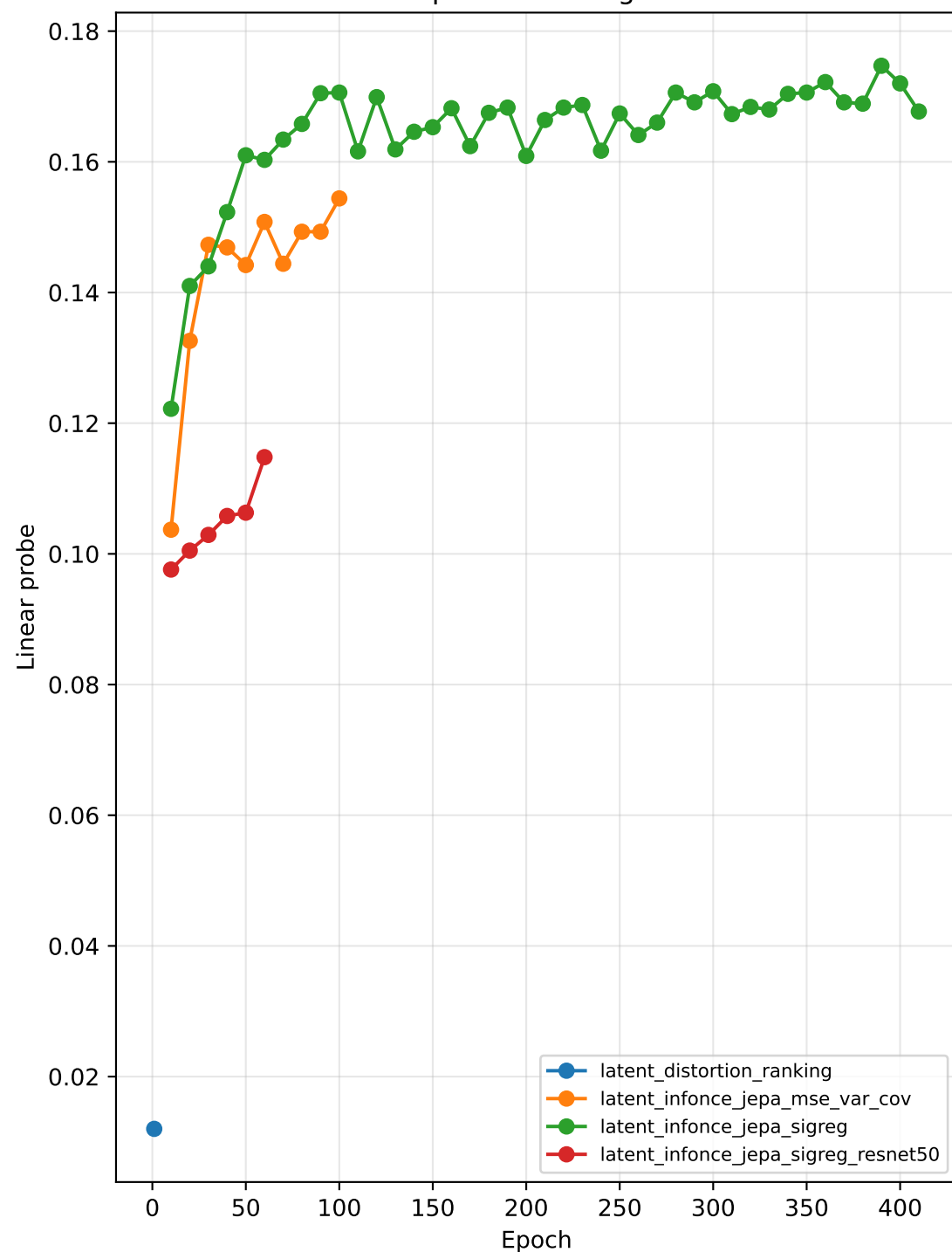
Linear probe learning curves
