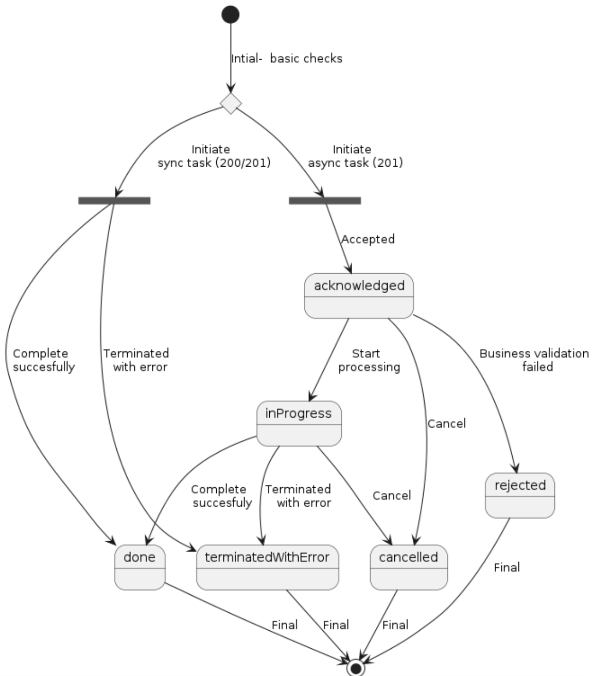
TMF Task Lifecycle
