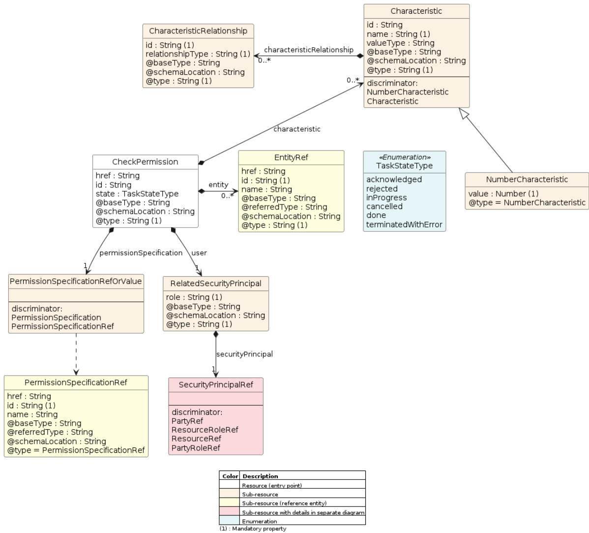
Figure 8 - CheckPermission
