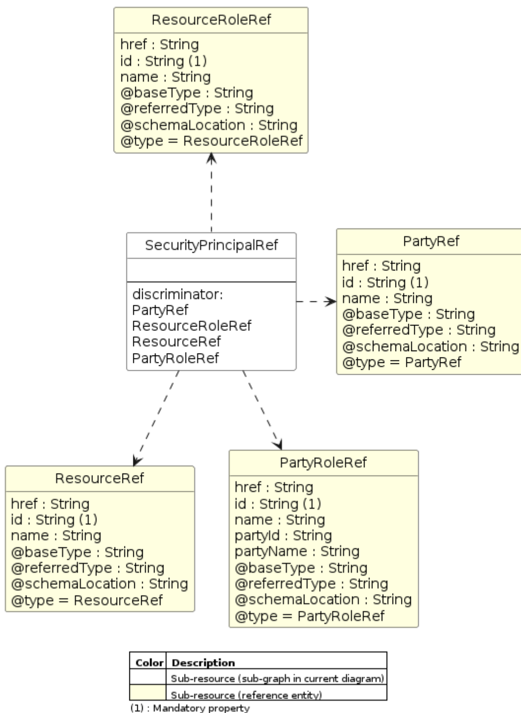
Figure 3 - SecurityPrincipalRef
