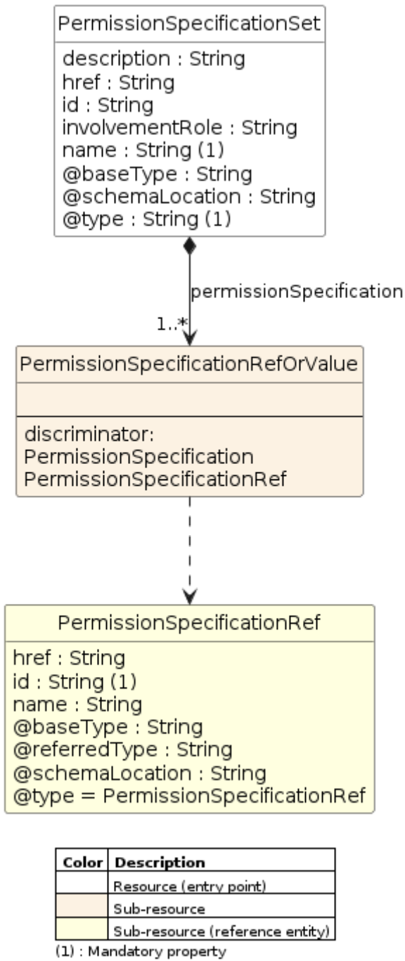
Figure 5 - PermissionSpecificationSet
