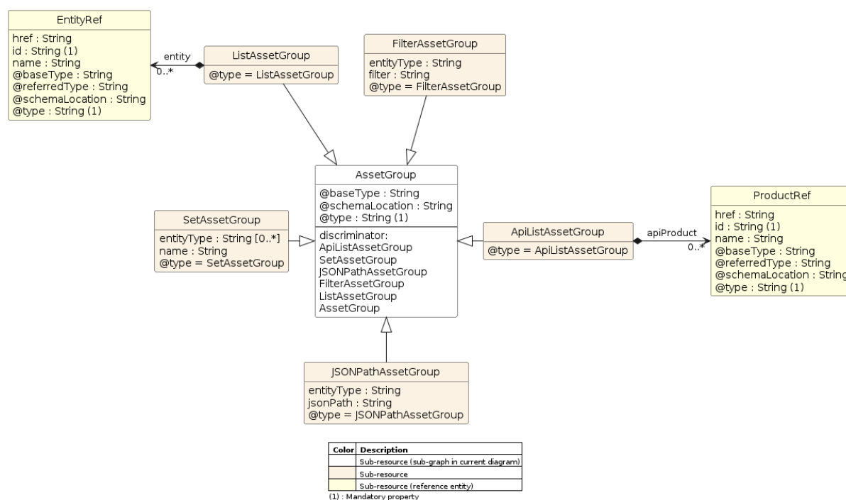
Figure 4 - AssetGroup
