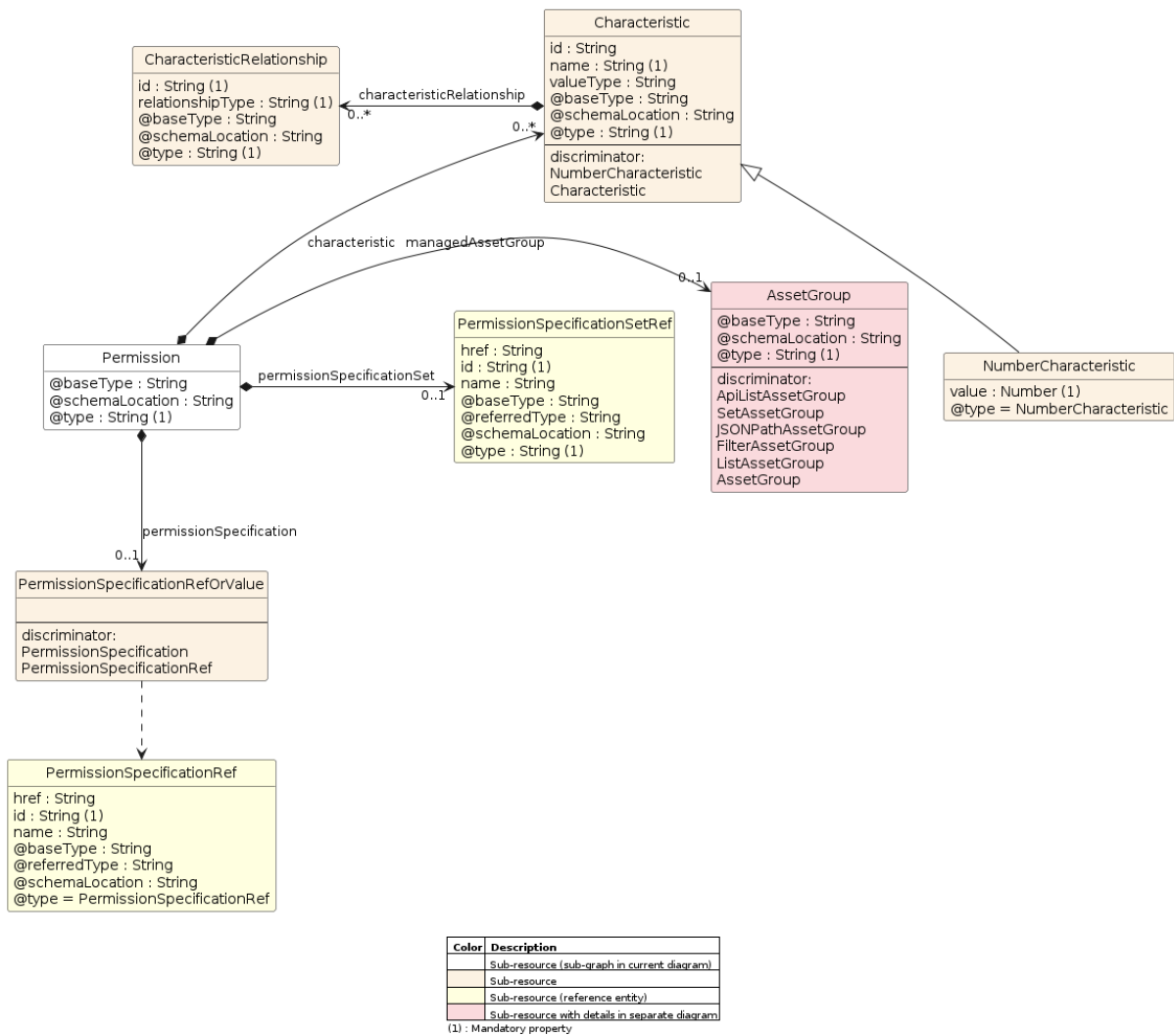
Figure 2 - Permission
