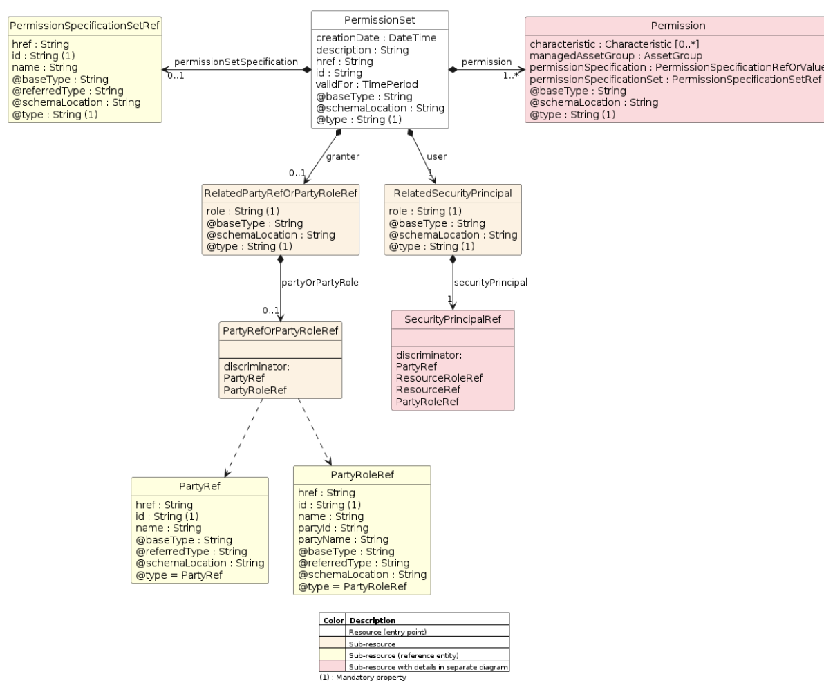
Figure 1 - PermissionSet
