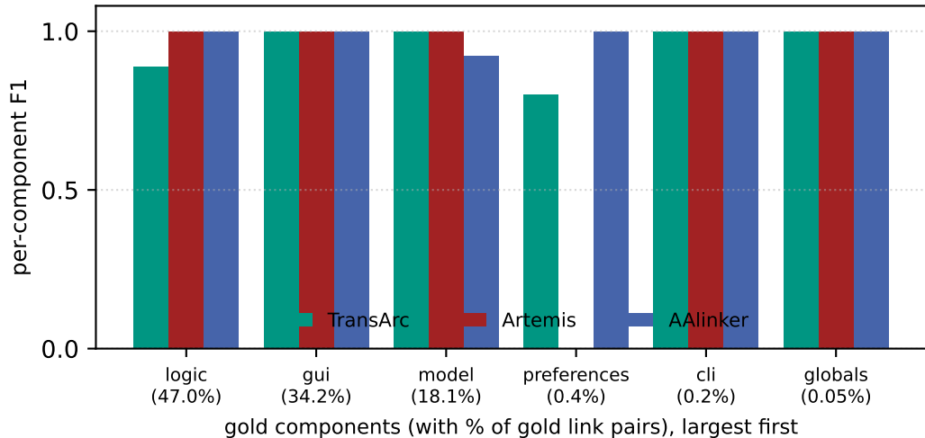
JabRef doc-to-code: per-component F1 across all 6 components (AAlinker = s20 union, mean of 1 run)
