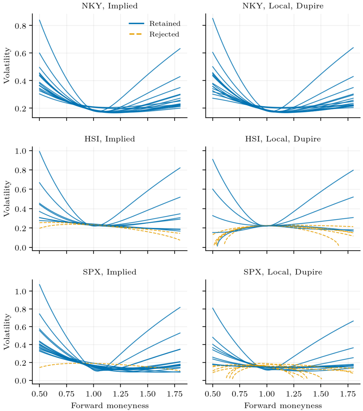
Figure 2: Fitted implied and local volatility curves across forward moneyness.
