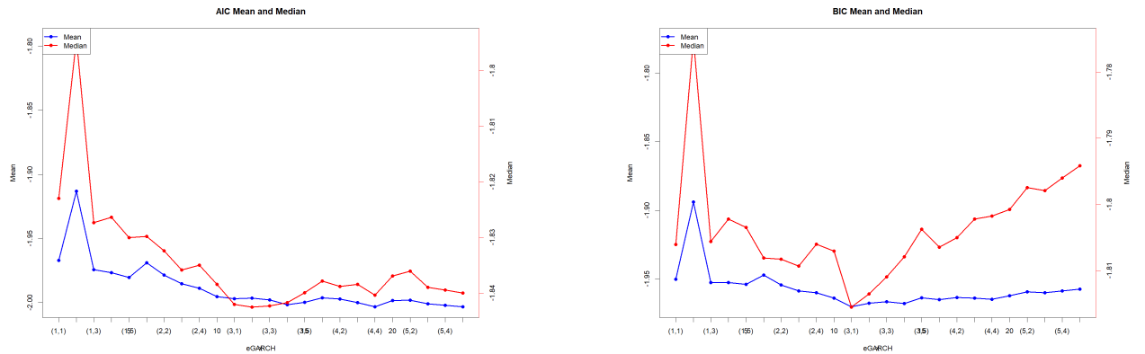
Figure 2: Akaike and Bayesian information criterion by eGARCH order.
