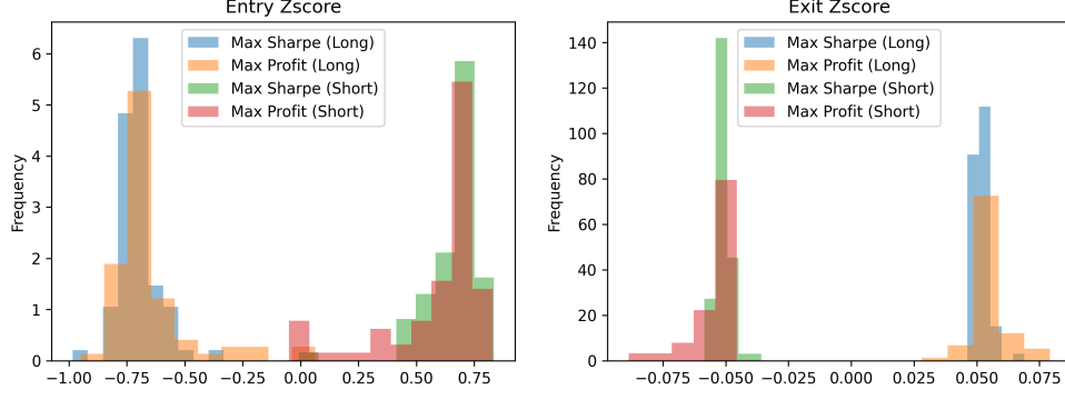
Figure 3: Distribution of the optimized entry and exit thresholds.
