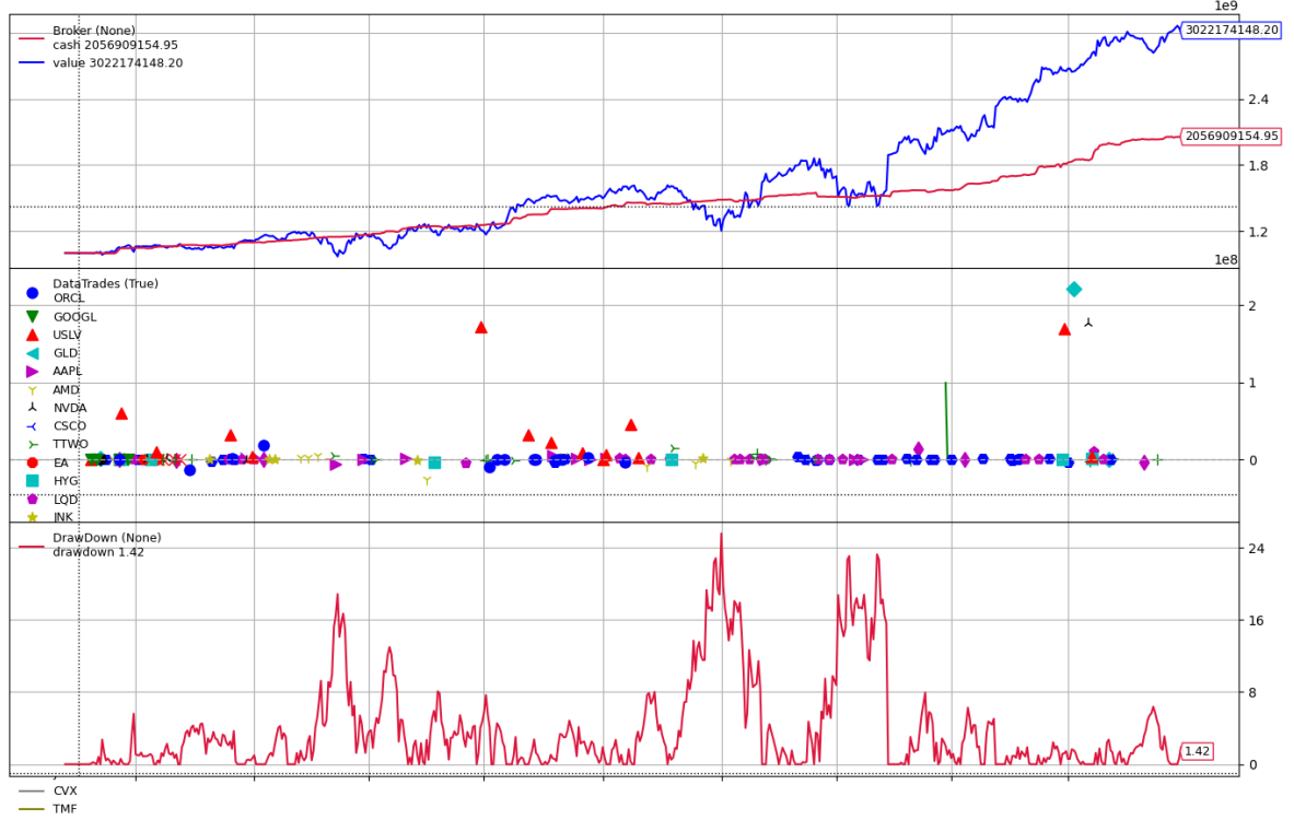
Figure 6: Backtest paths for OW-OE.
