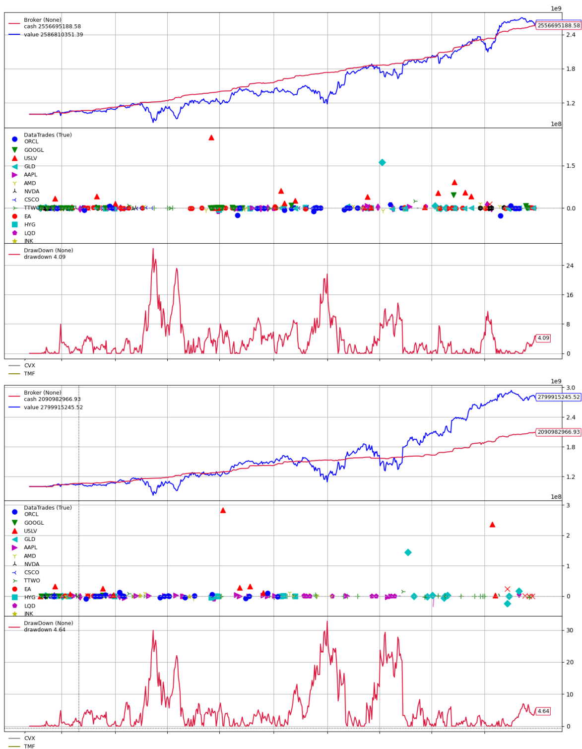
Figure 5: Backtest paths for EW-FE, upper, and EW-OE, lower. Each panel reports portfolio value, cash, per-trade profit and loss and drawdown.
