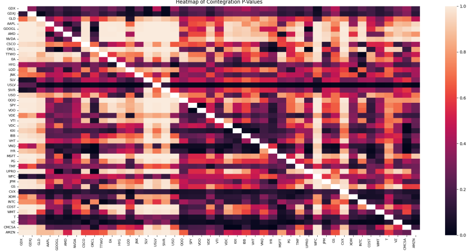
Figure 1: Engle-Granger p-values for every candidate pair on the training sample. Darker cells indicate stronger evidence of cointegration.
