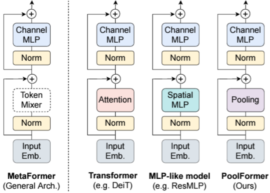
Figure 19: The MetaFormer block, reproduced from Yu et al. (2022). The token mixer on the left is a slot rather than a fixed choice, and the three instances to its right are attention, a spatial multi-layer perceptron and pooling. Fast-ViT places a depthwise convolution in that slot.
