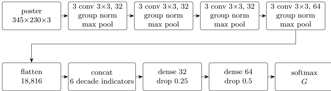
Figure 14: The convolutional network built from scratch of Section 3.
