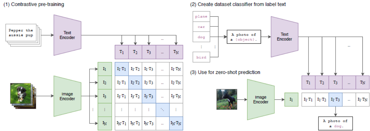
Figure 17: CLIP, reproduced from Radford et al. (2021). Panel one is the contrastive pre-training of Equation (3) and panel three is the zero-shot rule of Equation (4), which is what this report uses.
