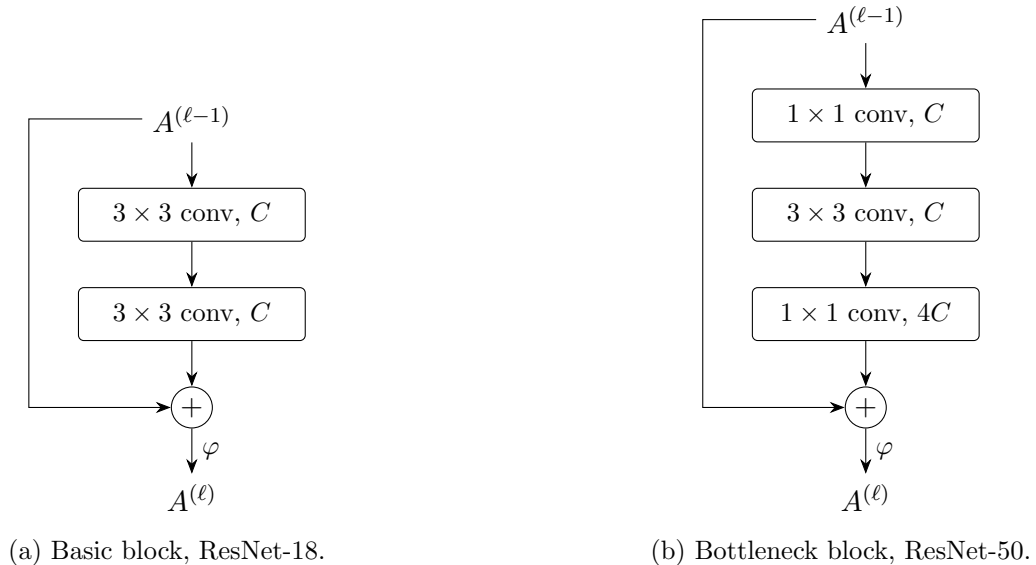
Figure 8: The two residual blocks of Equation (1).
