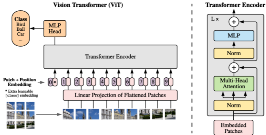
Figure 18: The vision transformer, reproduced from Dosovitskiy et al. (2021). Two of the four CLIP image encoders are this architecture at patch sizes 32 and 16.
