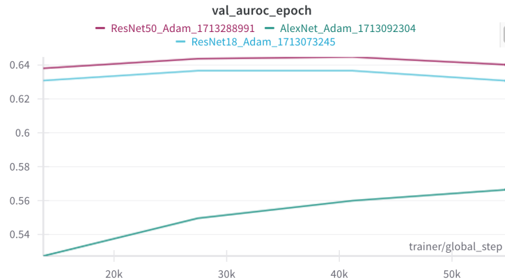
Figure 10: Validation AUROC by epoch for AlexNet and ResNets under Adam.
