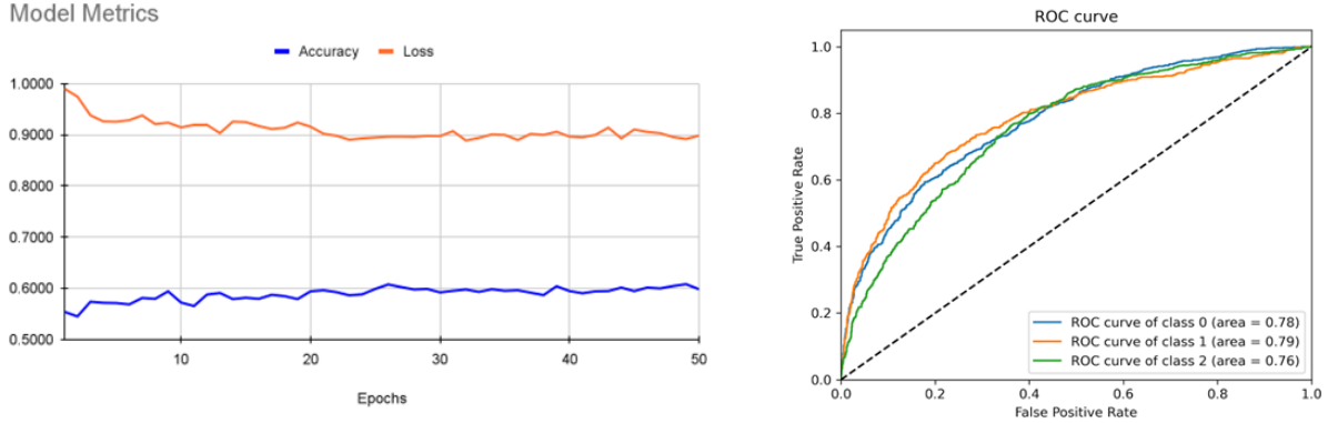
Figure 5: Fit and discrimination of the VGG16 classifier. Validation accuracy and loss by epoch on the left, ROC curves on the held-out sample on the right.
