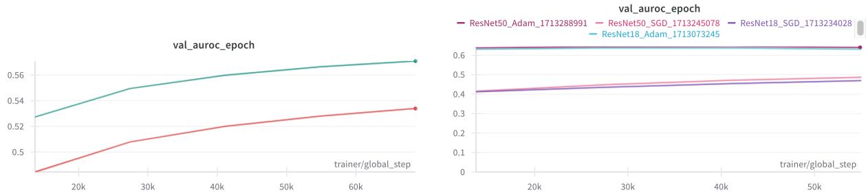
Figure 9: Validation AUROC by epoch under Adam and stochastic gradient descent, for AlexNet (left) and ResNet (right).
