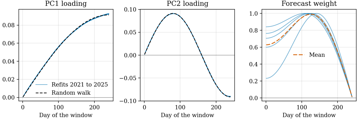
Figure 3. Loadings of the first two principal components at each refit from 2021 to 2025 with the eigenvectors of a random walk, and the forecast weight \eta_g relative to the largest weight.
