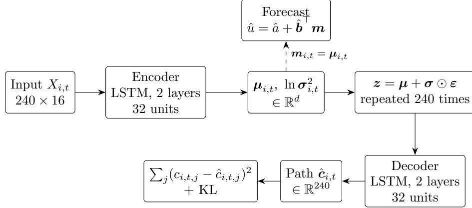
Figure A.1. Architecture of the VAE. The encoder reads 240 days of sixteen features and returns the mean and log variance of the latent, and the decoder receives a draw of the latent at each of 240 steps and rebuilds the cumulative path of standardized returns. The posterior mean \mathbf{m}_{i,t} is the embedding that enters the forecast.
