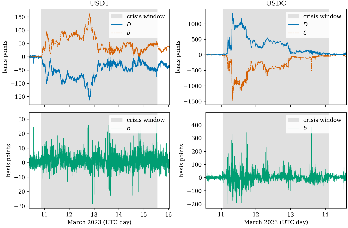
Figure 1: Cross-currency basis D and peg deviation \delta (top), and triangular arbitrage deviation b (bottom) in bps, 1-minute close prices from 12 hours before to 12 hours after each crisis window (shaded), UTC.
