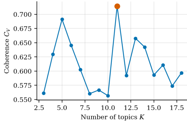
Figure B.1: Coherence C_V of LDA against the number of topics K .
