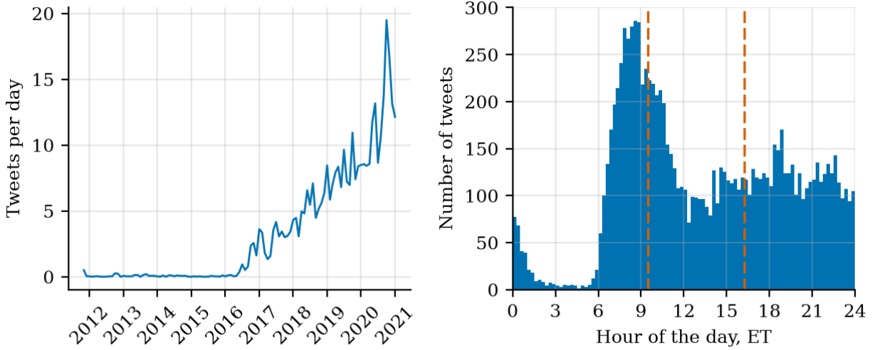
Figure 1: Monthly mean tweets per calendar day (LHS) and time of posting for tweets from 2016 onward (RHS), with the open at 9:30 and the VIX close at 16:15 ET marked.
