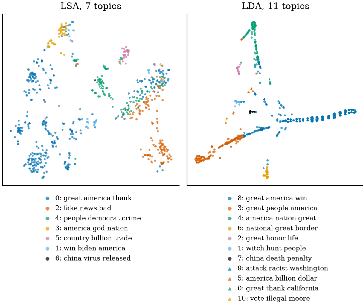
Figure B.2: t-SNE maps of the LSA weights with seven topics (left) and the LDA weights with eleven topics (right).
