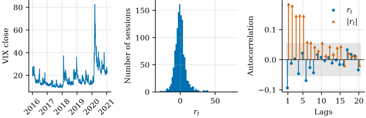
Figure 2: VIX close V_t (left), histogram of the daily log change r_t (middle), and autocorrelations of r_t and |r_t| up to 20 lags (right).
