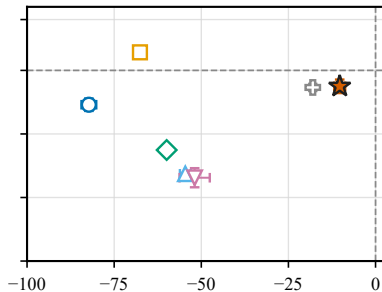
(b) Banking77
