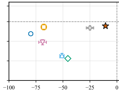
(c) FewRel
