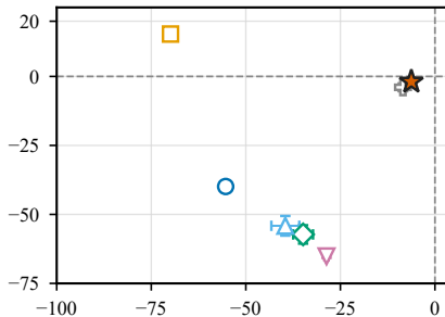
(a) CLINC150
