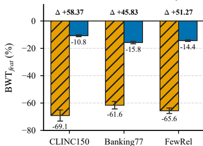
(b) Expanding head: BWT feat
