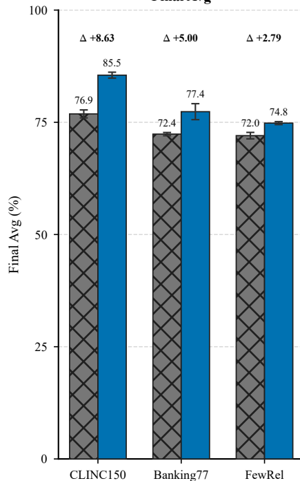
(e) Prototype-only readout Final Avg
