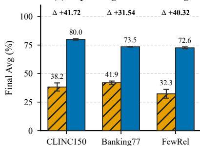
(a) Expanding head: Final Avg
