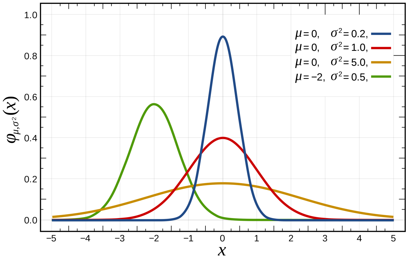
Figure 2: Normal distribution
