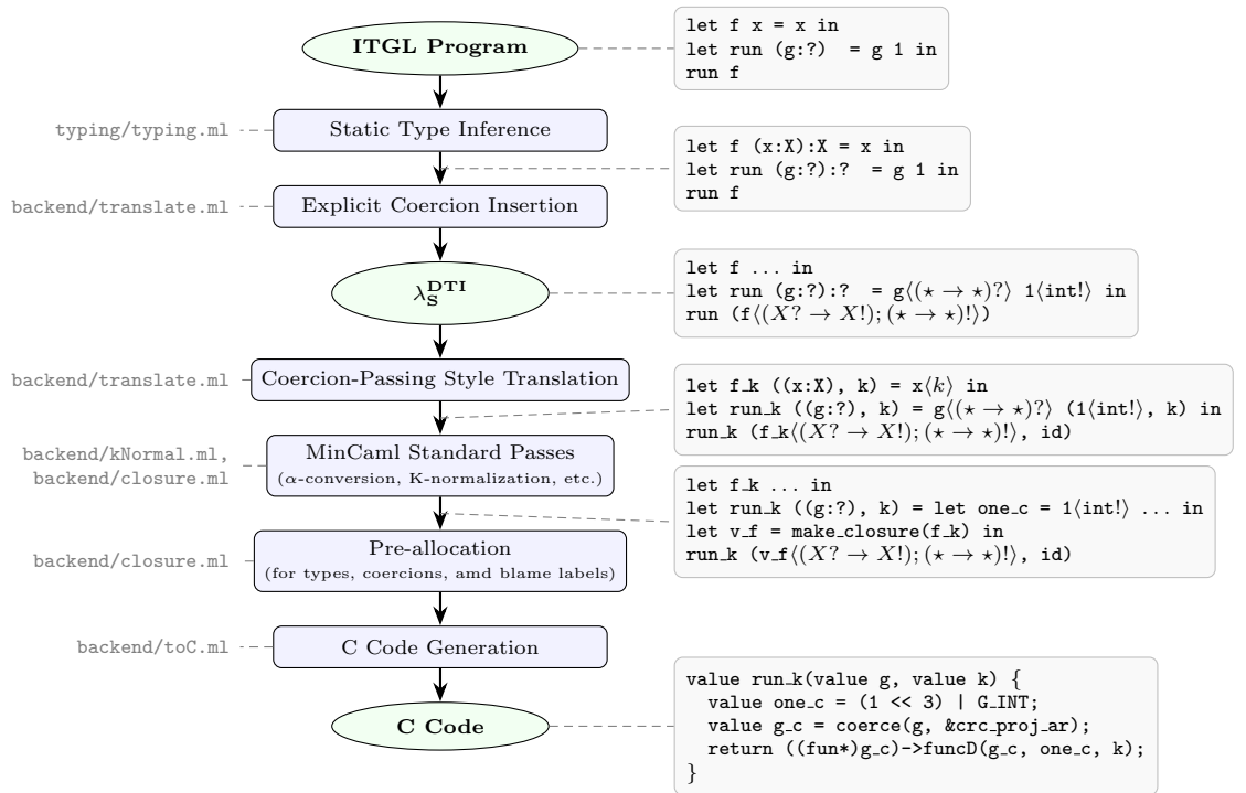
Figure 1: Overall flow of the compilation process.
