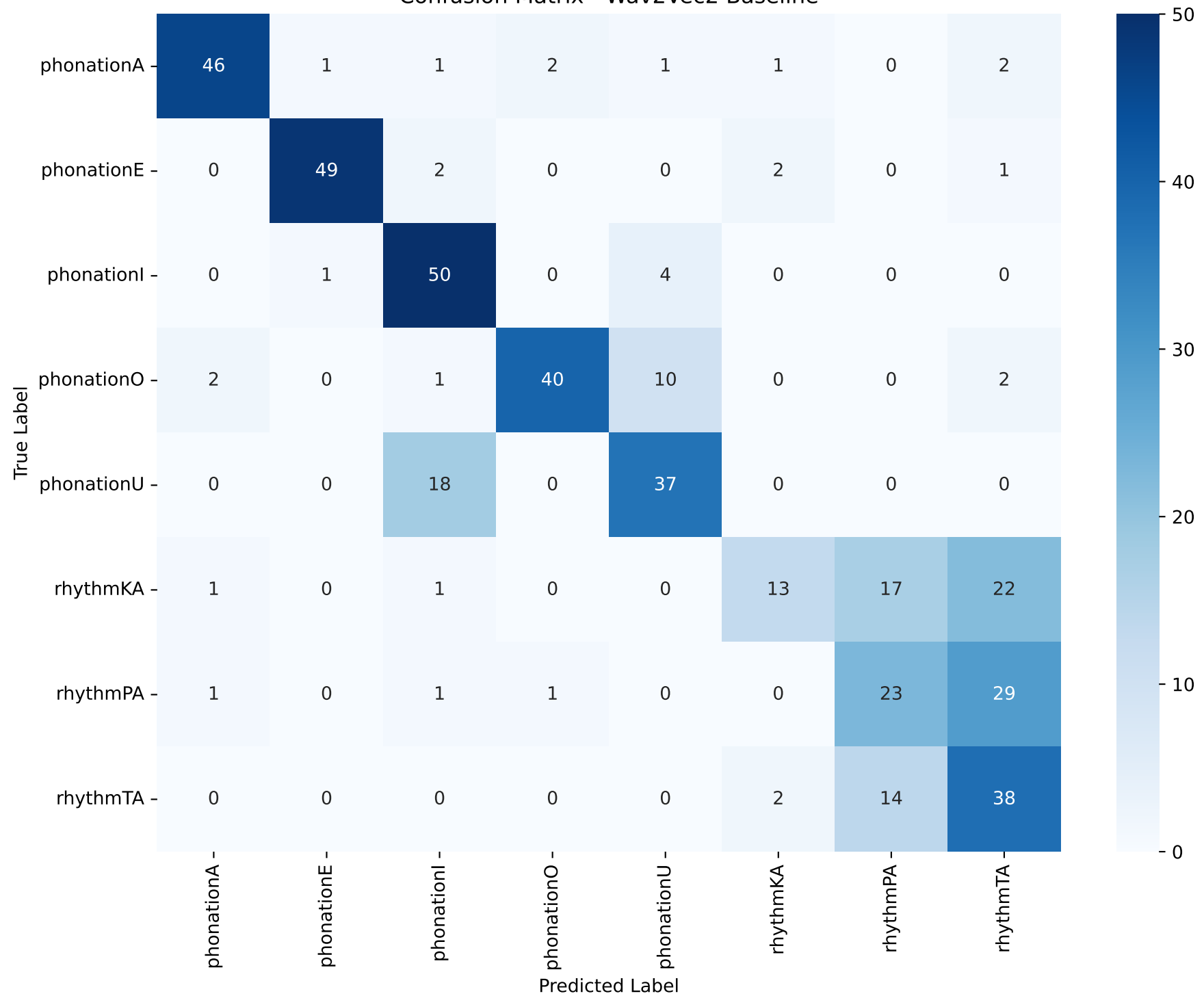
Confusion Matrix - Wav2Vec2 Baseline
