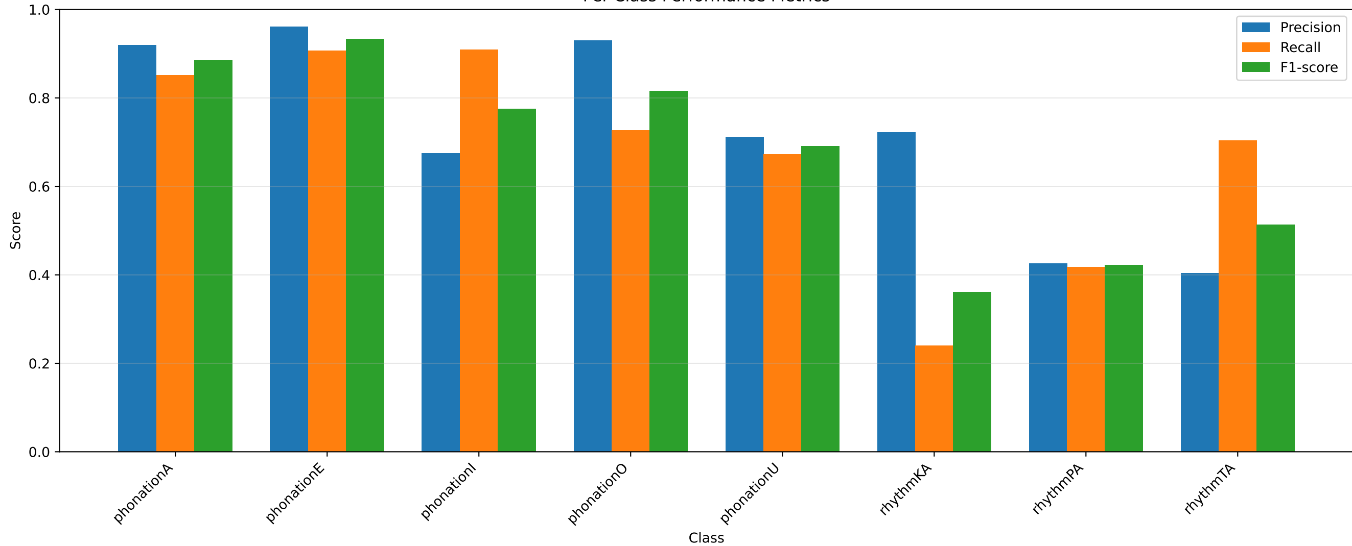
Per-Class Performance Metrics
