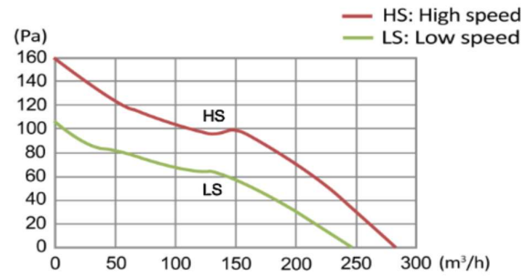
Model HS-125P
