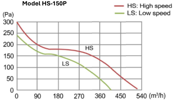
Model HS-150P
