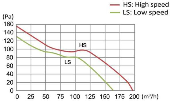
Model HS-100P
