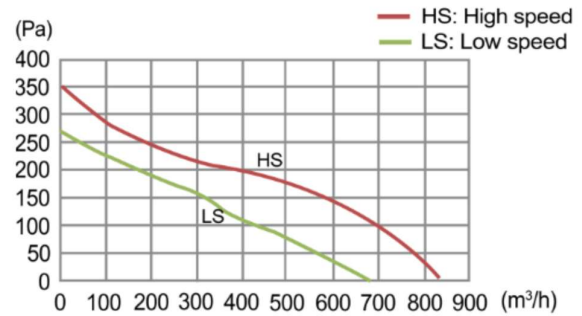
Model HS-200P
