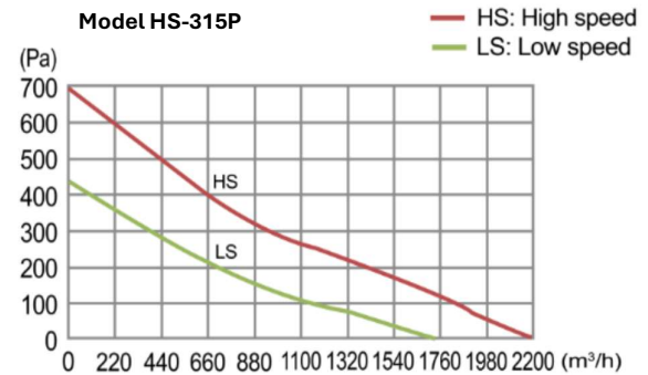
Model HS-315P
