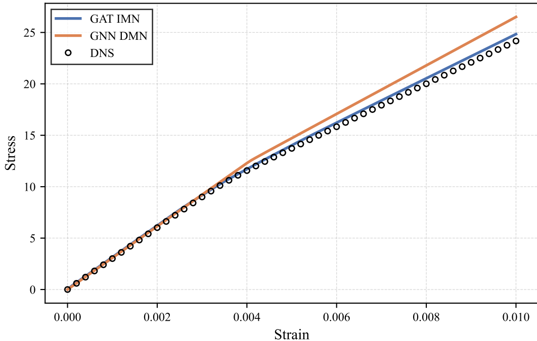
Load Case 3
