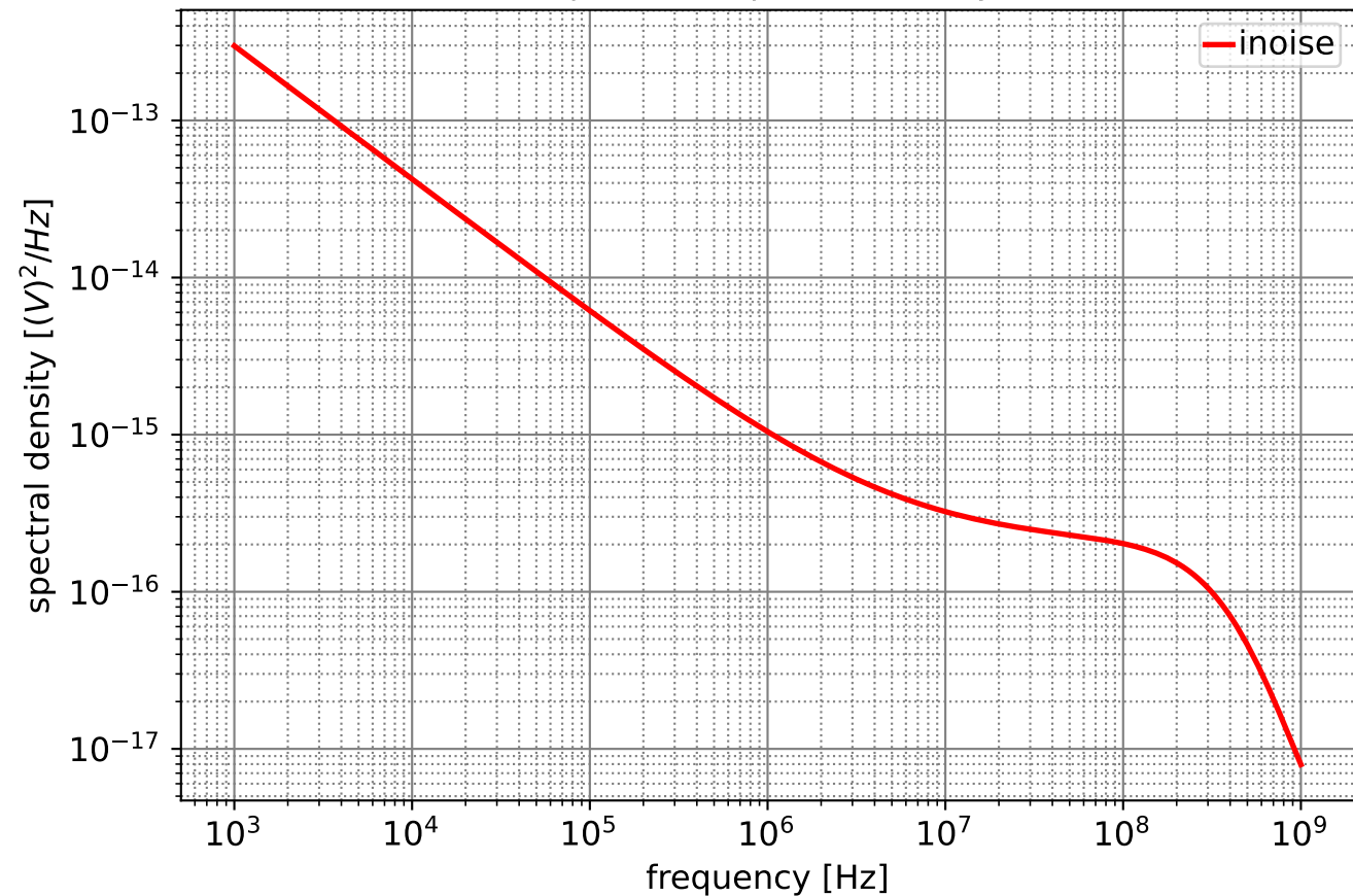
input noise spectral density
