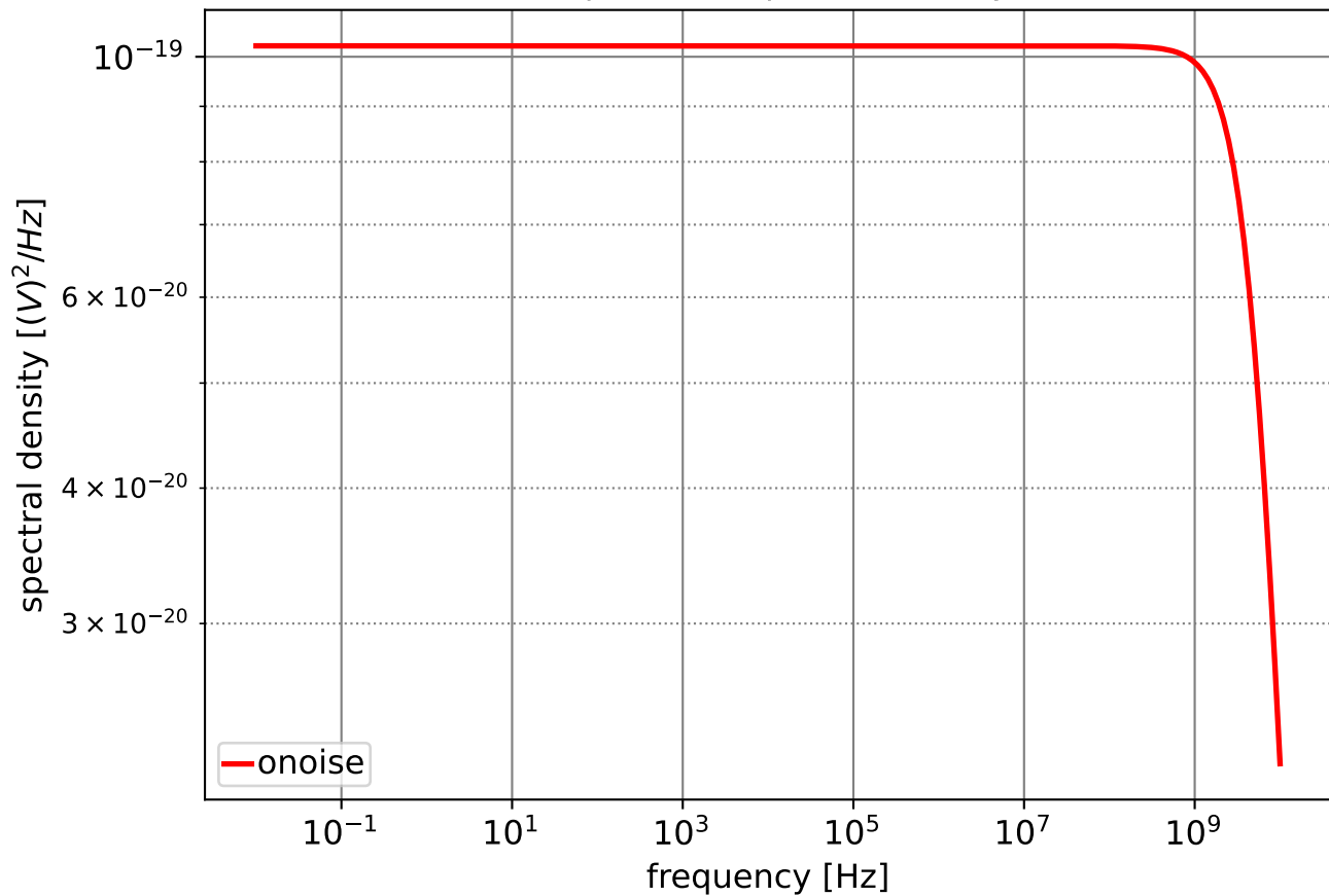
Output noise spectral density
