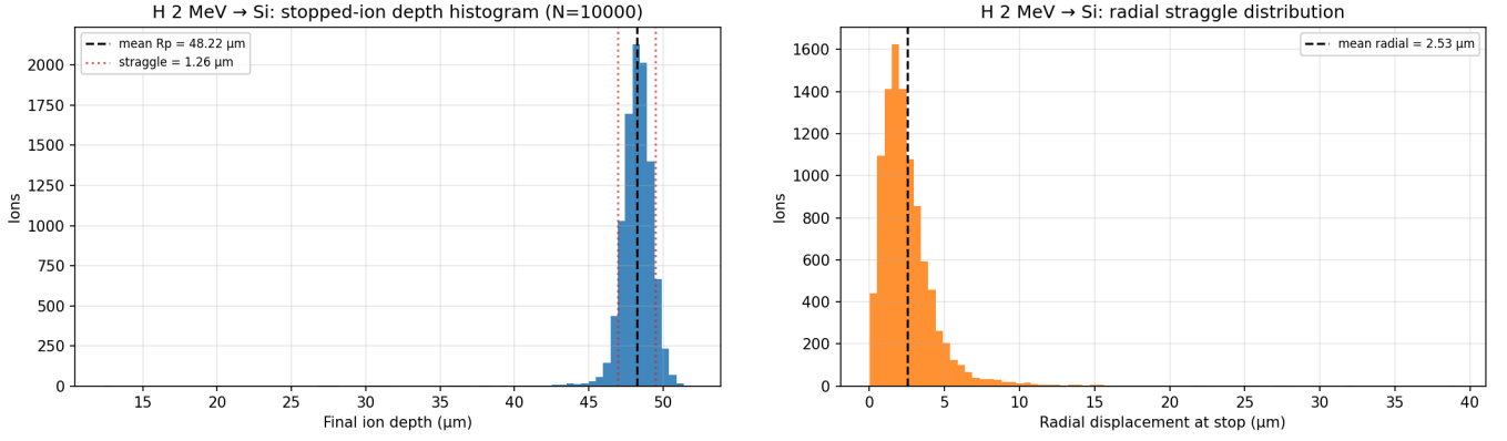
Figure A.6: 2 MeV H in Si. (a) Stopped-ion depth distribution; mean range 48.22 μm with 1.255 μm straggling, a depth resolution of 2.6%. (b) Radial displacement at the stopping point; radial straggling 2.023 μm, which gives IBIC its spatial resolution on buried structures.
