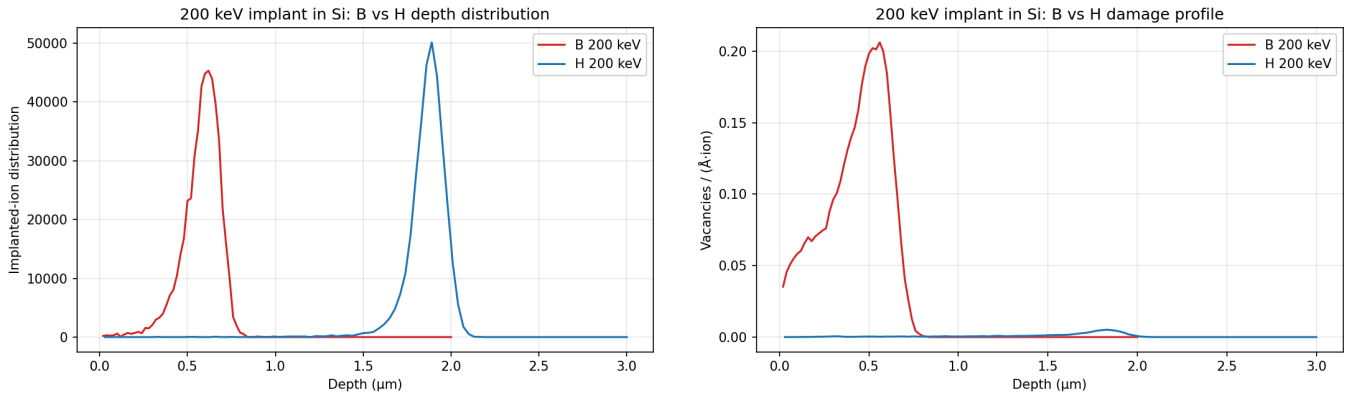
Figure A.8: 200 keV implants in Si: B versus H. (a) Implanted-ion depth distributions — boron stops 3.25 \times shallower (0.569 μm) than hydrogen (1.850 μm), with a proportionally much broader, visibly skewed profile. (b) Damage profiles — boron produces 37.4 \times more vacancies per ion (795 against 21.3), concentrated in a thinner, shallower layer peaking at 0.56 μm.
