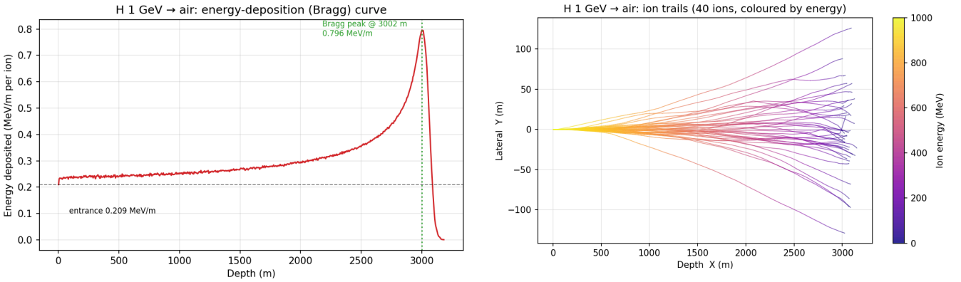
Figure A.2: 1 GeV H in air. (a) Energy-deposition (Bragg) curve: deposition rises slowly across the first three kilometres and peaks sharply at 3002 m, delivering 0.796 MeV/m against 0.209 MeV/m at entry — a factor of 3.8. This is the basis for the answer to Project 1(d). (b) Ion trails coloured by energy, showing tracks essentially straight while the protons are fast (yellow) and fanning out to \pm 100 m as they slow (purple).
