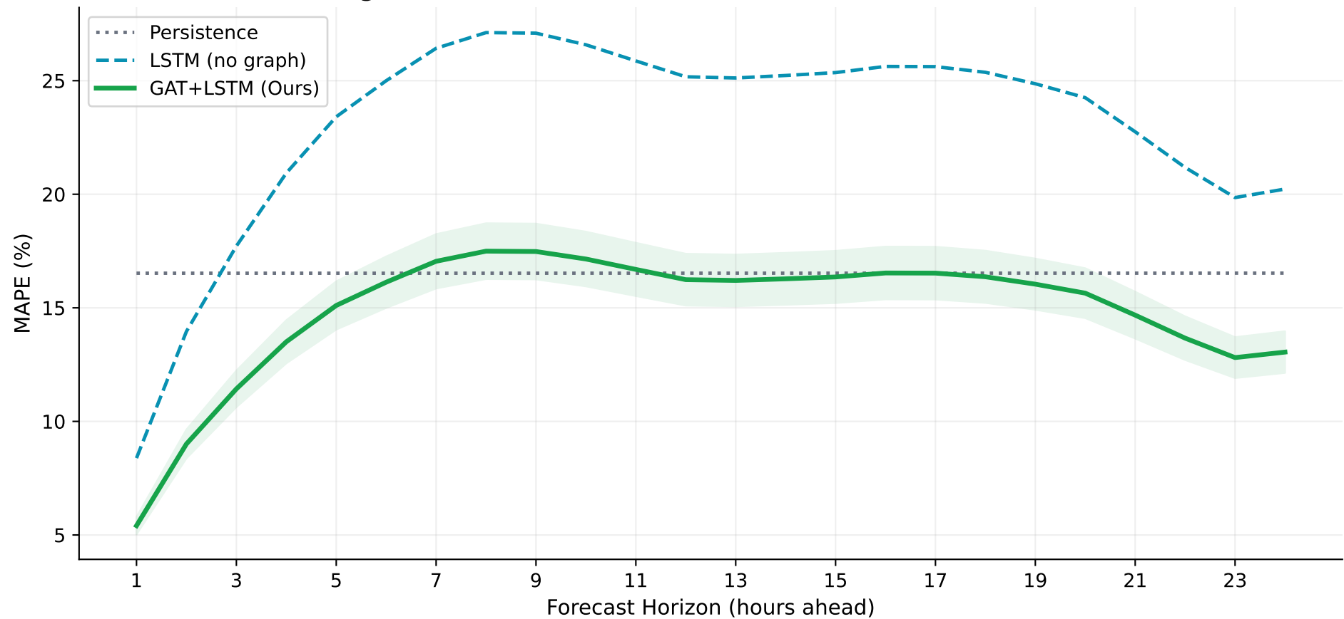
Fig. 12 — MAPE vs Forecast Horizon (1-24h, Real Test Set)
