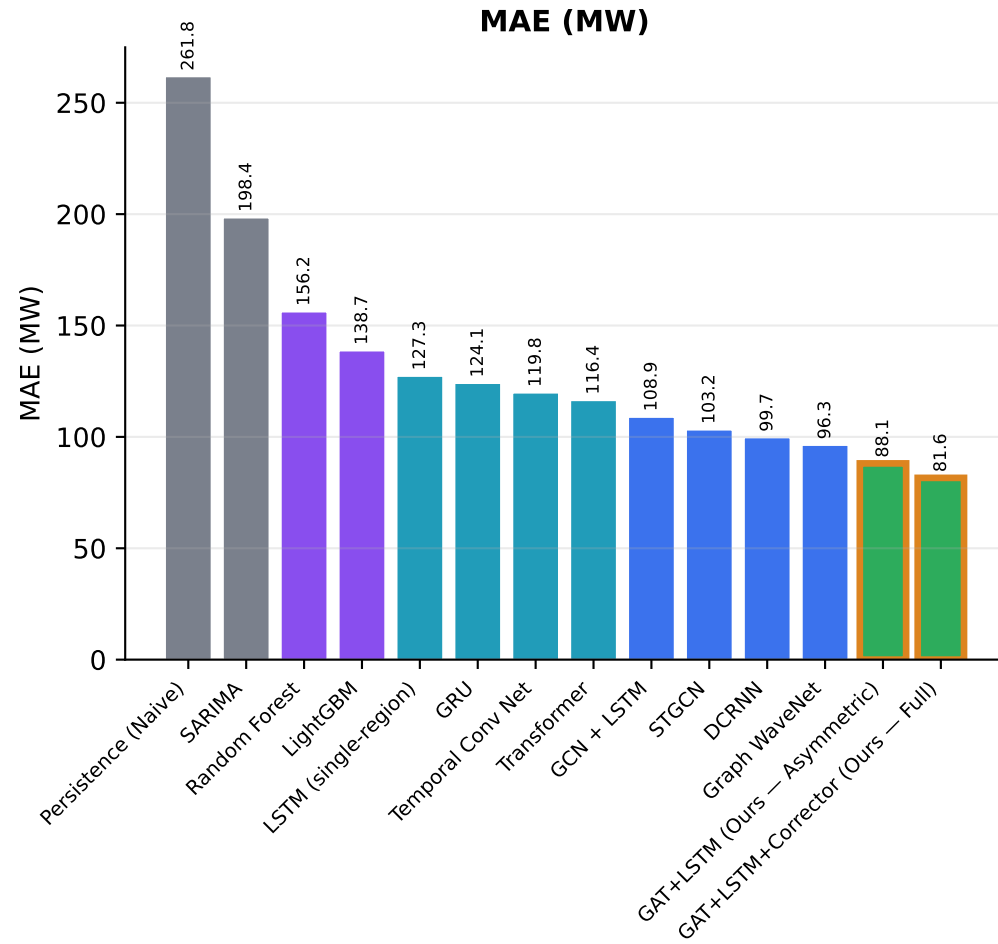
Fig. 4 — Baseline Comparison: Spain Regional Electricity Demand Forecasting (Test Set 2025-2026)
