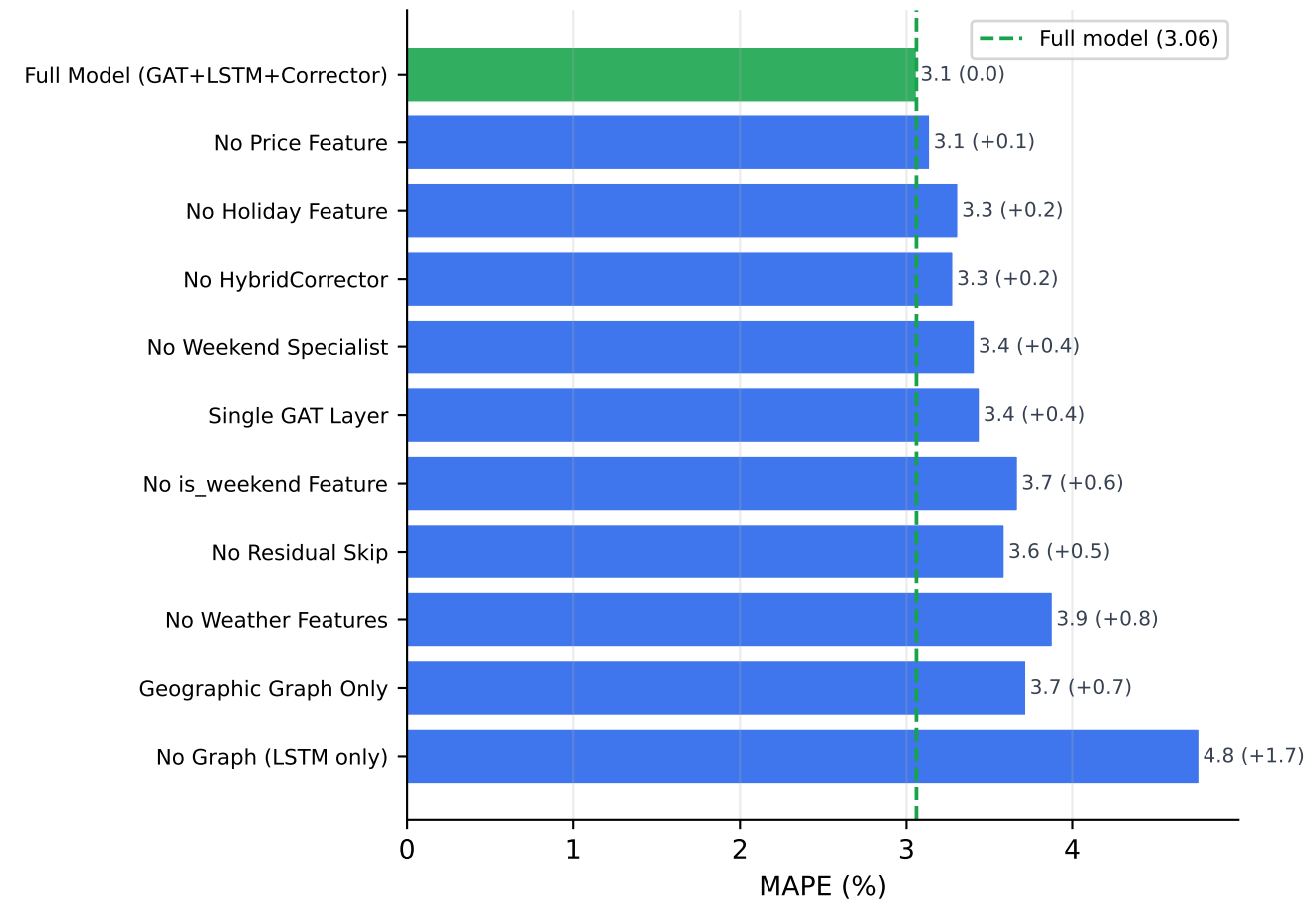
Ablation — MAPE (%)
