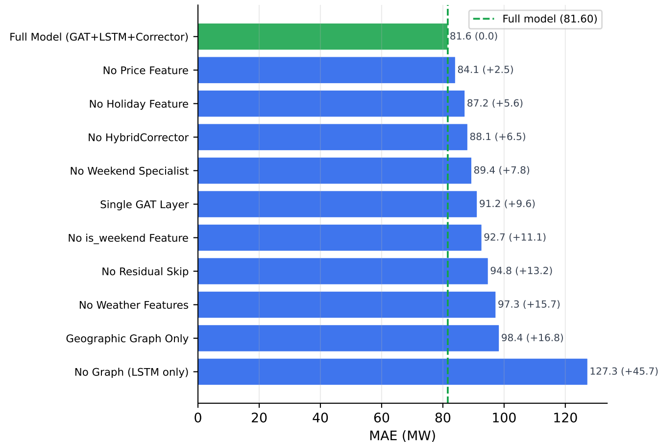
Ablation — MAE (MW)
