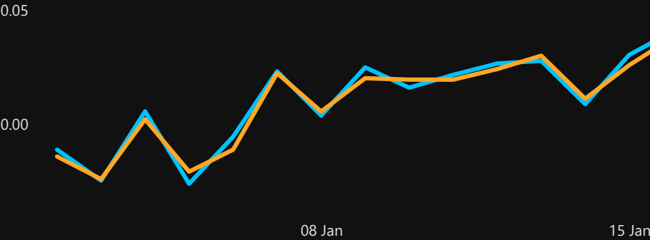
Indicator Summary
