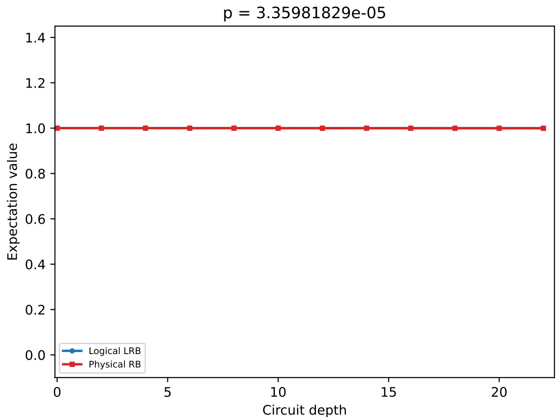
Terminal-Check Logical RB vs Physical RB under Single Qutrit Local Depolarizing Channels
