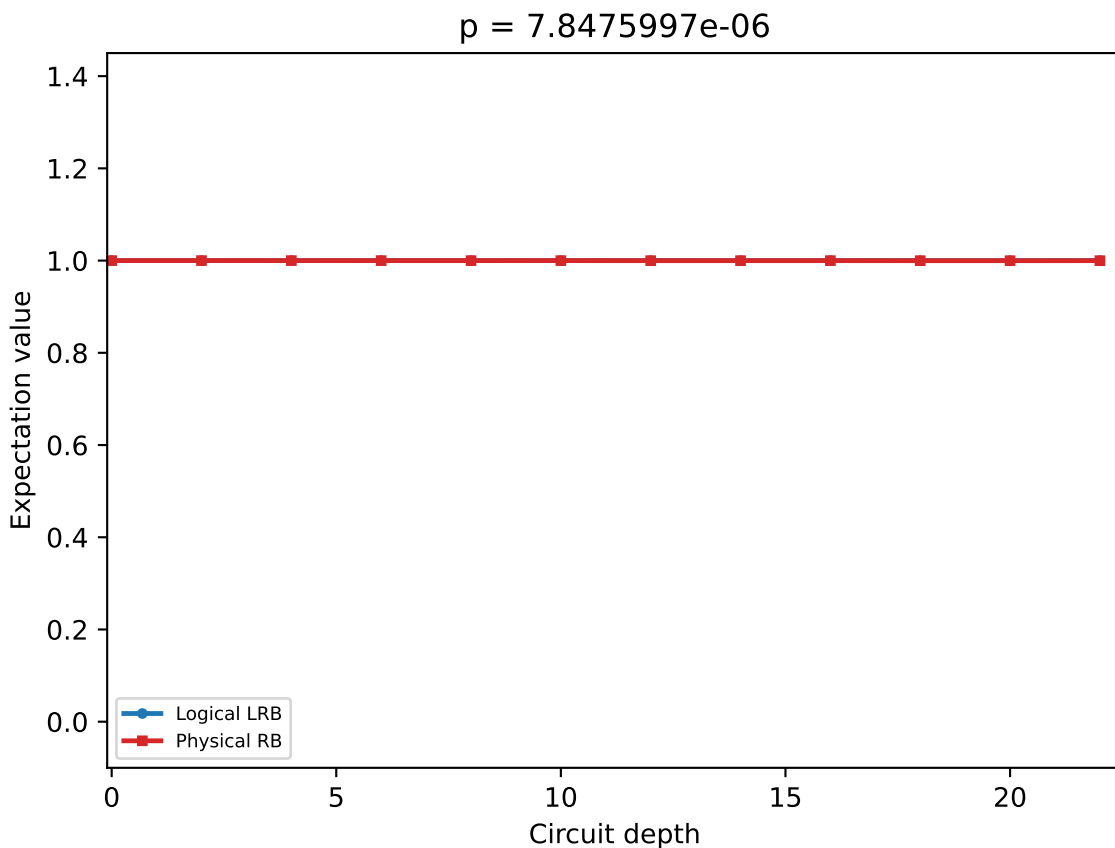
Terminal-Check Logical RB vs Physical RB under Single Qutrit Local Depolarizing Channels
