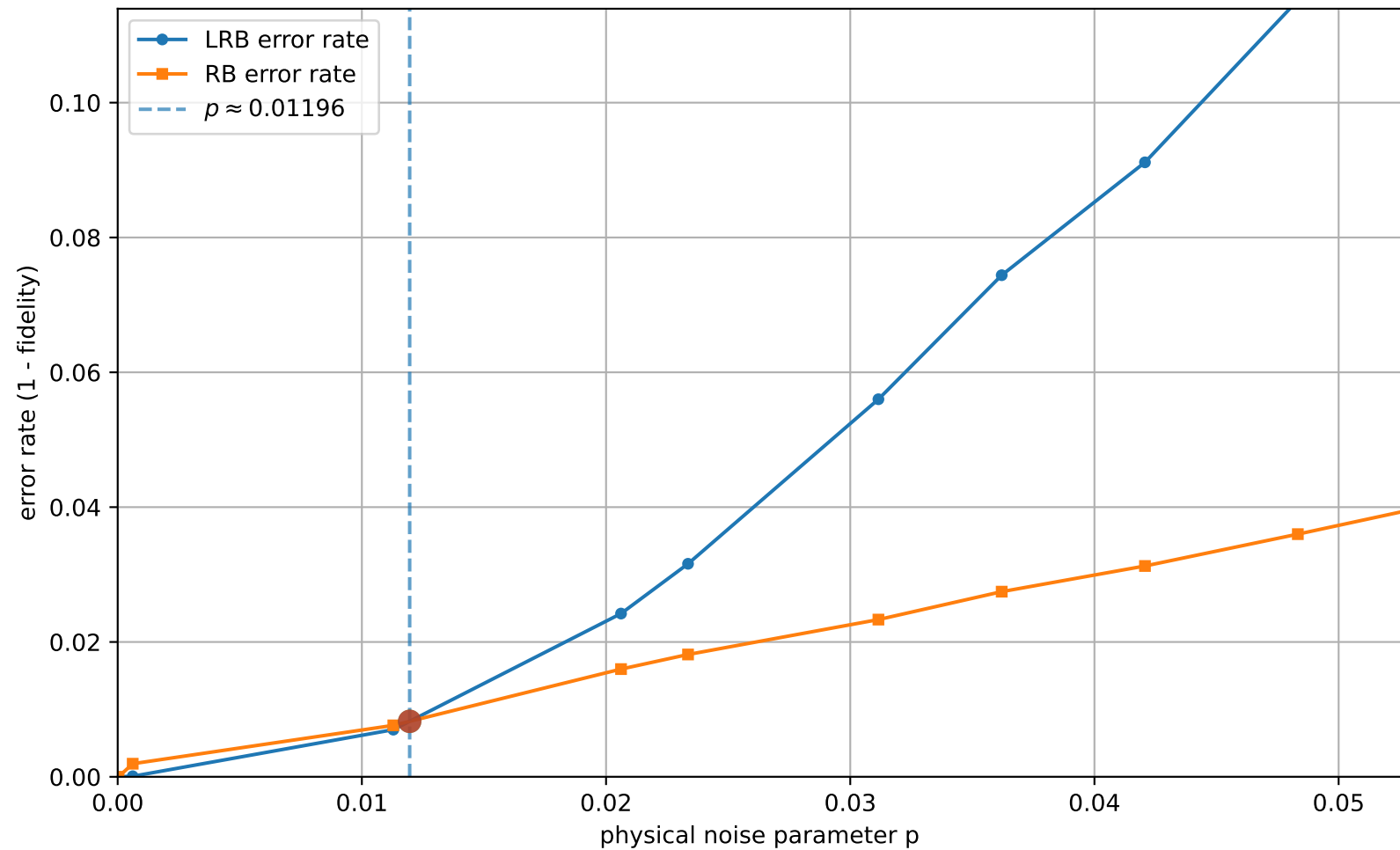
LRB vs RB (uniform interval check = 17, q=3 , [[3, 1, 2]]_3 ): error rates vs p
