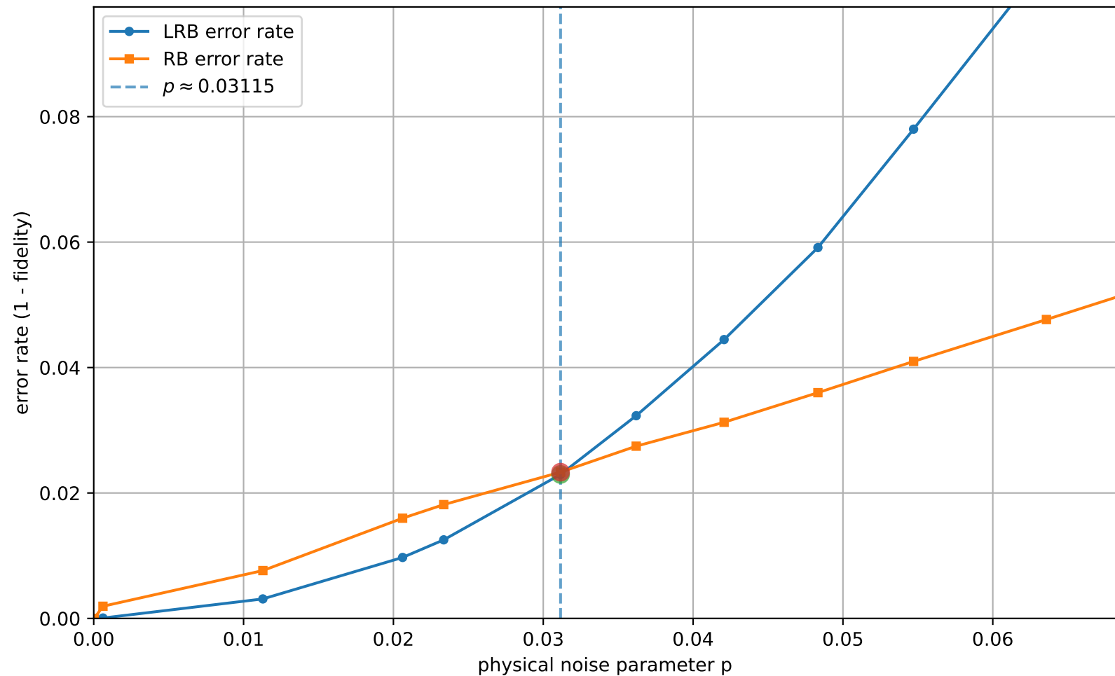
LRB vs RB (uniform interval check = 6, q=3, [[3, 1, 2]]_3 ): error rates vs p
