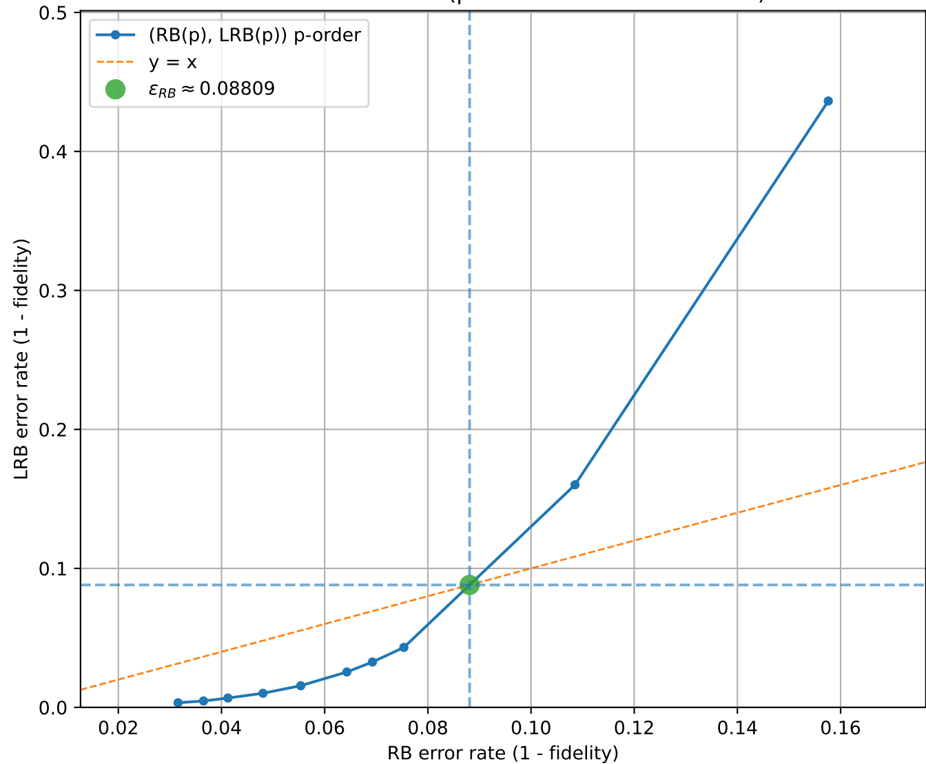
unif=2: LRB vs RB (p-window around threshold)
