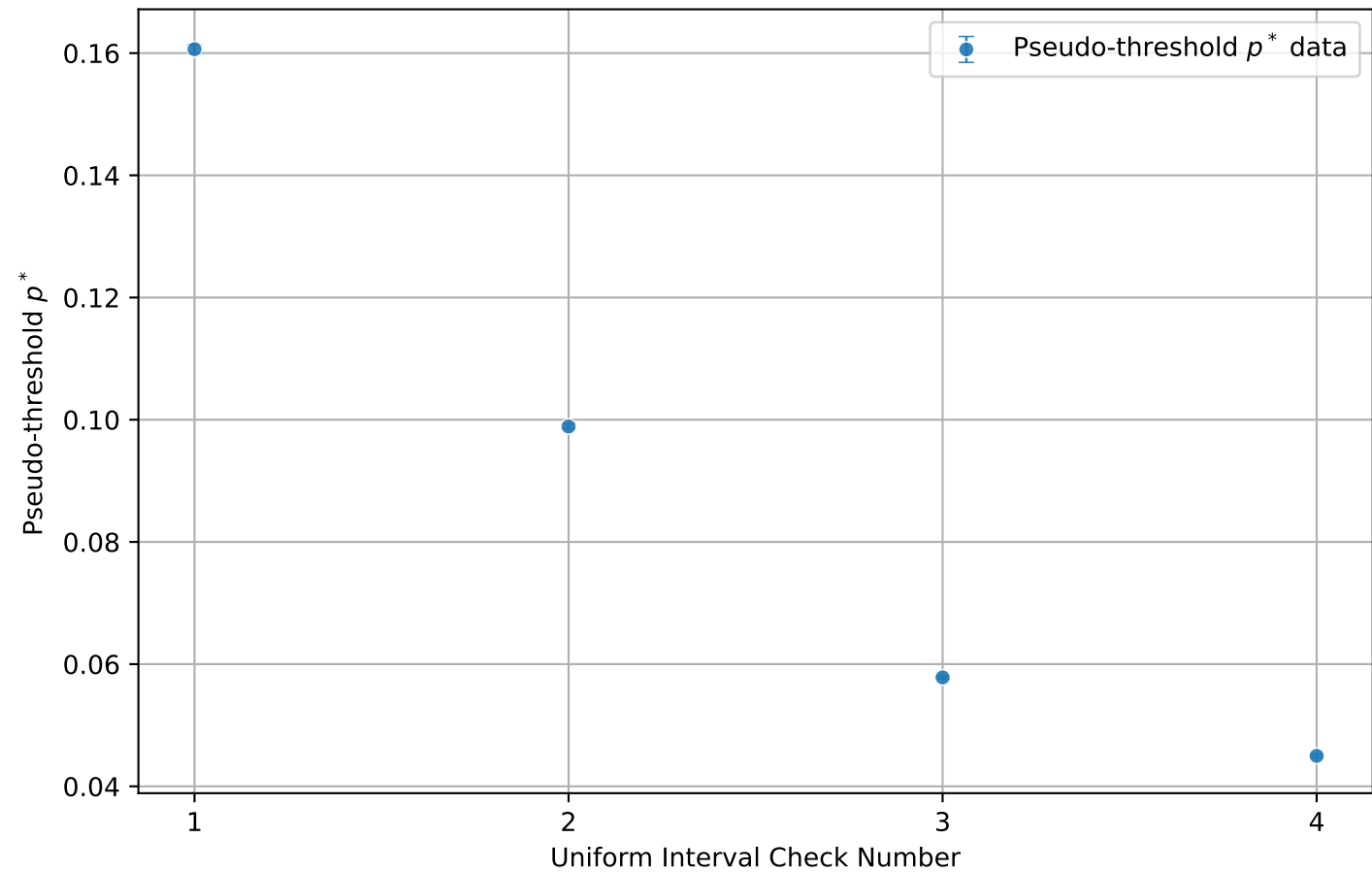
Pseudo-threshold p^* vs Uniform Interval Check (q=3, [[3, 1, 2]]_3 )
