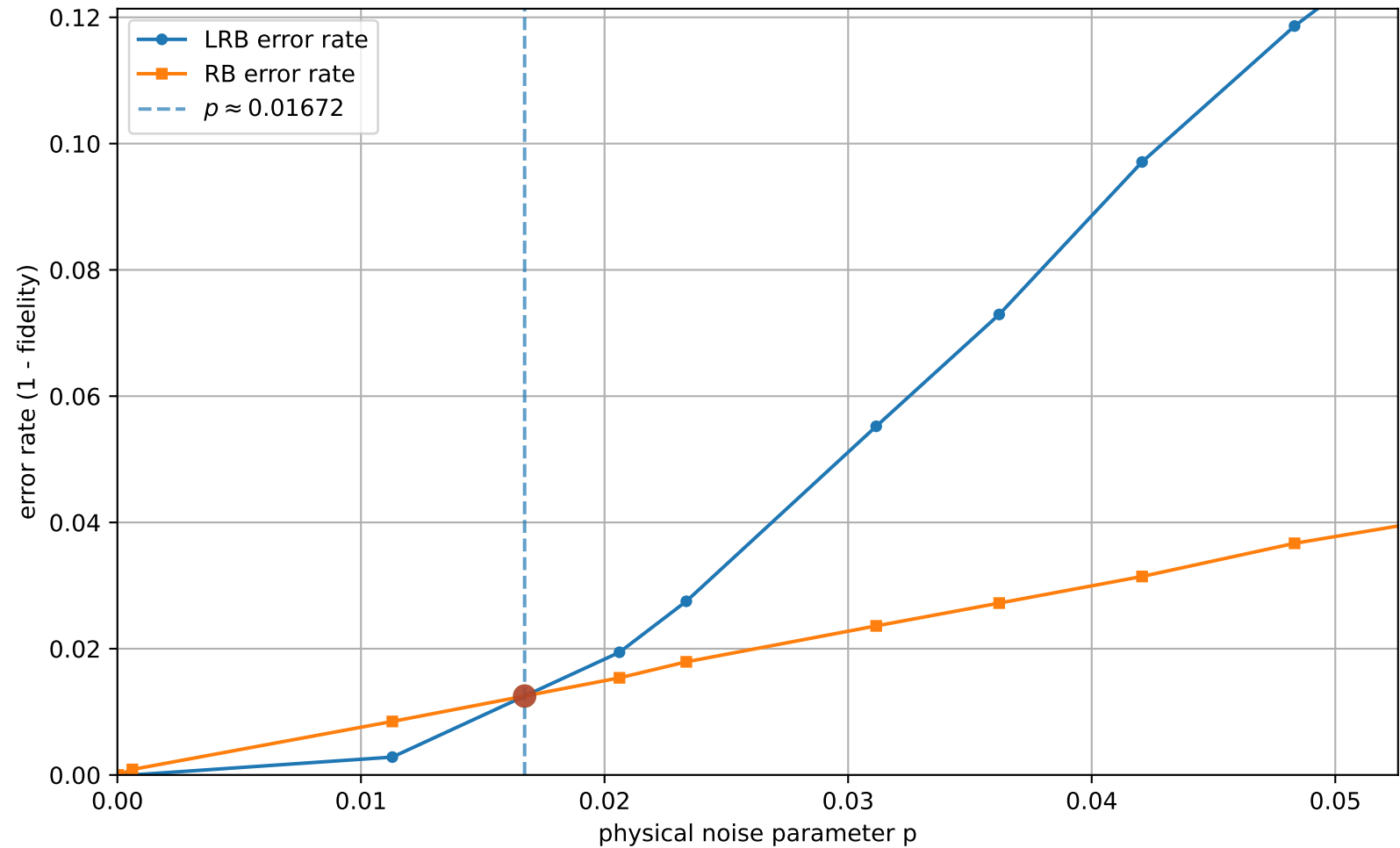
LRB vs RB (uniform interval check = 20, q=3 , [[5, 1, 2]]_3 ): error rates vs p
