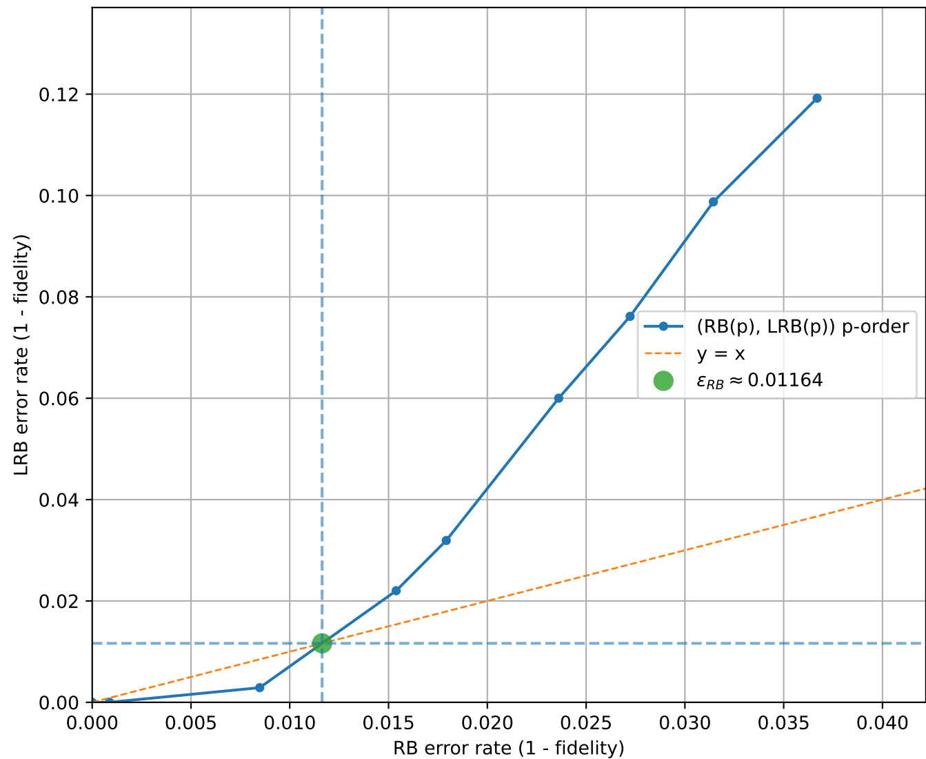
LRB vs RB (uniform interval check = 22, q=3 , [[5, 1, 2]]_3 )
