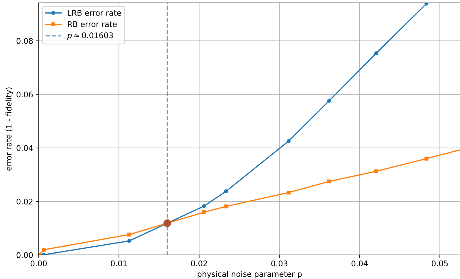
LRB vs RB (uniform interval check = 11, q=3, [[3, 1, 2]]_3 ): error rates vs p
