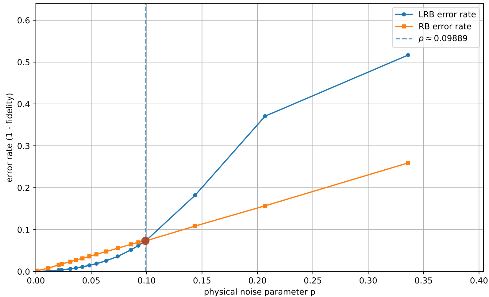
LRB vs RB (uniform interval check = 2, q=3, [[3, 1, 2]]_3 ): error rates vs p (zoom near threshold)
