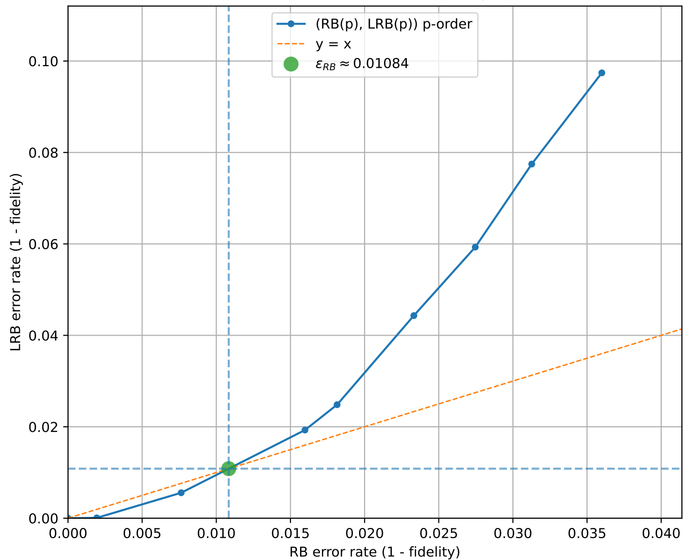
LRB vs RB (uniform interval check = 12, q=3 , [[3, 1, 2]]_3 )
