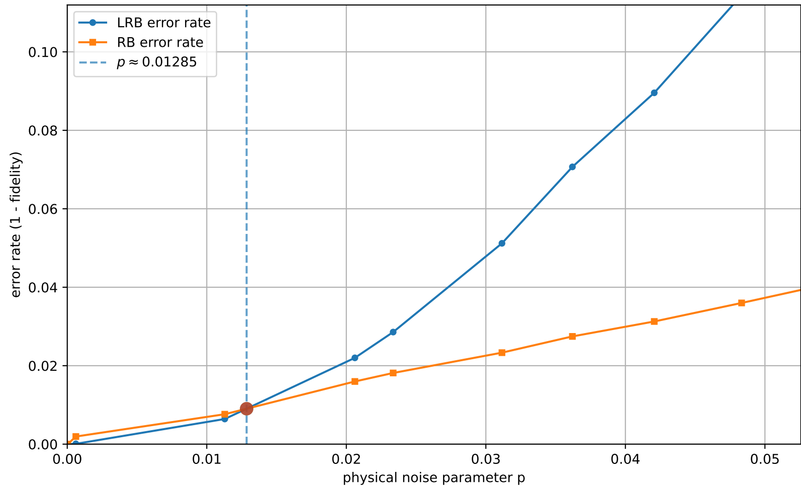
LRB vs RB (uniform interval check = 15, q=3 , [[3, 1, 2]]_3 ): error rates vs p
