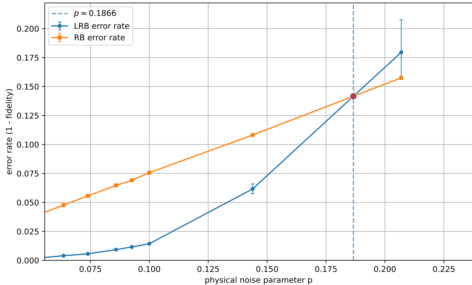
LRB vs RB (uniform interval check = 1, q=3 , [[5, 1, 2]]_3 ): error rates vs p
