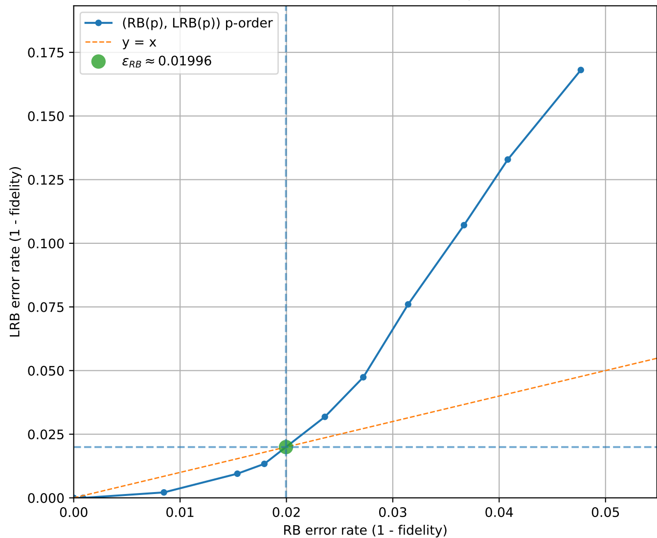
LRB vs RB (uniform interval check = 13, q=3 , [[5, 1, 2]]_3 )
