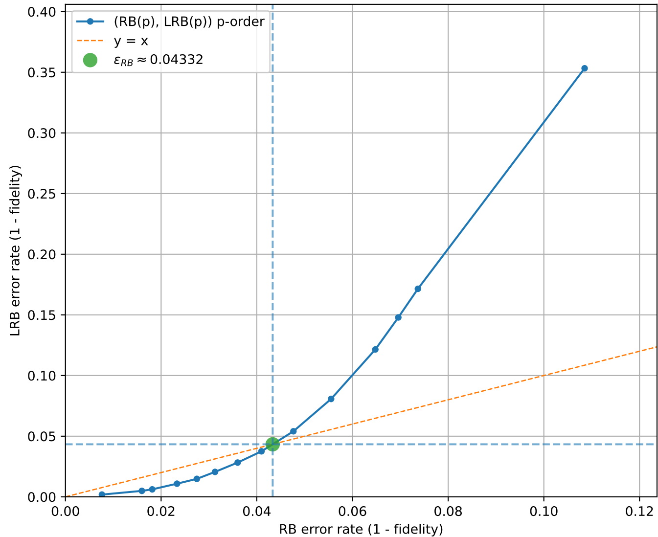
LRB vs RB (uniform interval check = 3, q=3 , [[3, 1, 2]]_3 ): p-window around threshold
