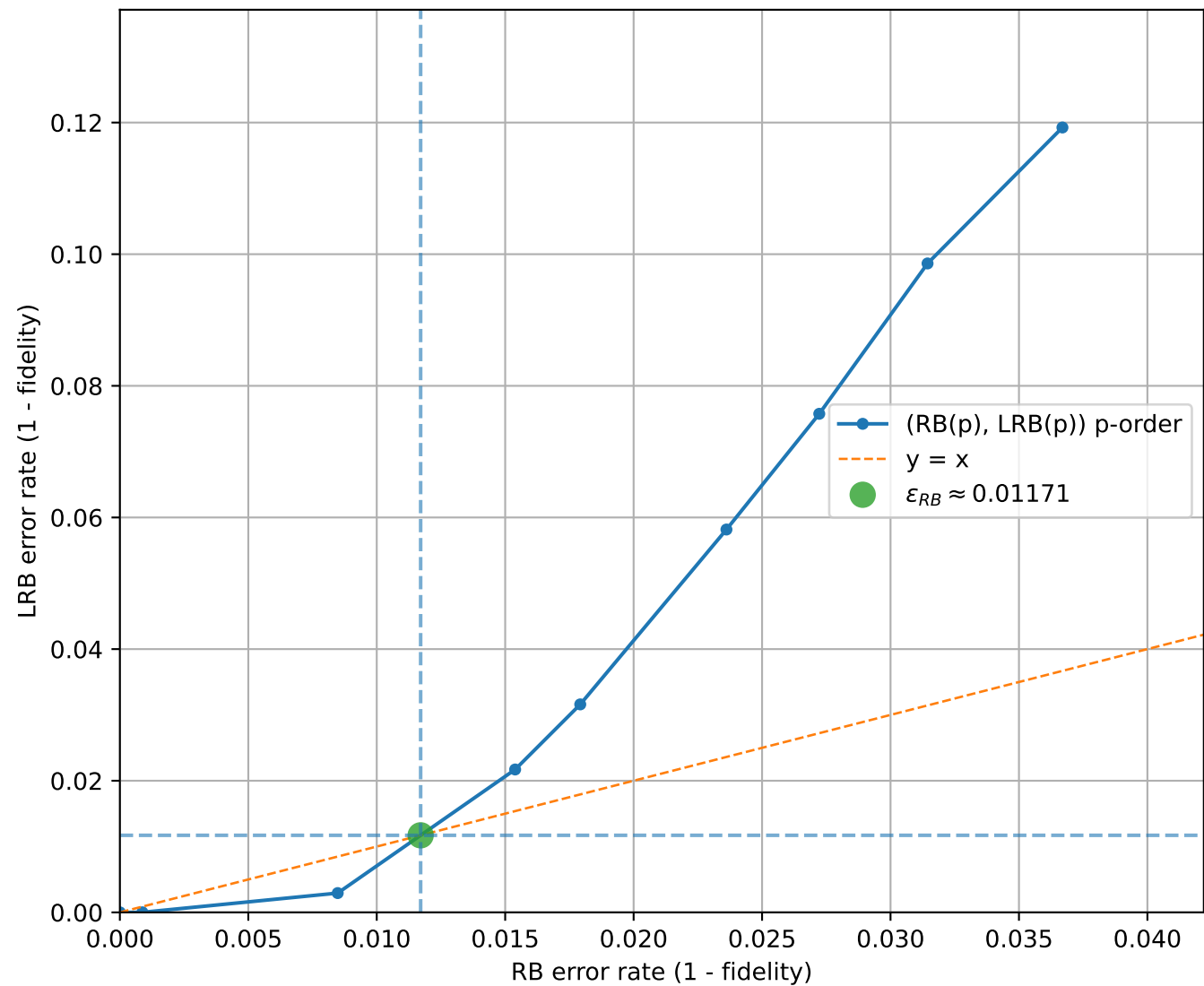
LRB vs RB (uniform interval check = 21, q=3 , [[5, 1, 2]]_3 )
