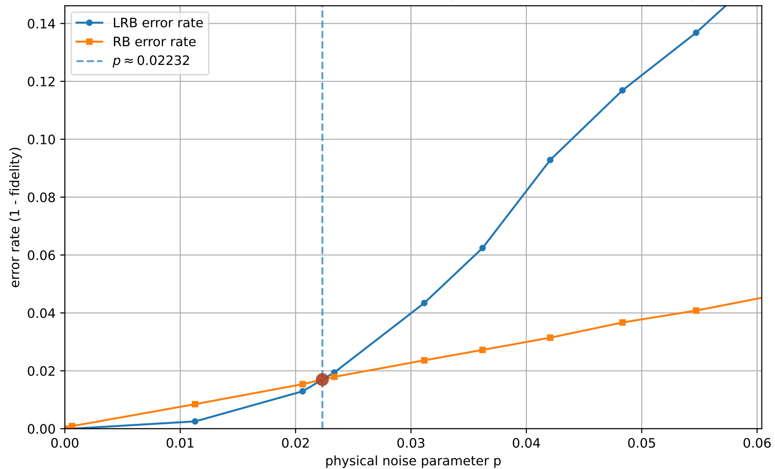
LRB vs RB (uniform interval check = 17, q=3, [[5, 1, 2]]_3 ): error rates vs p
