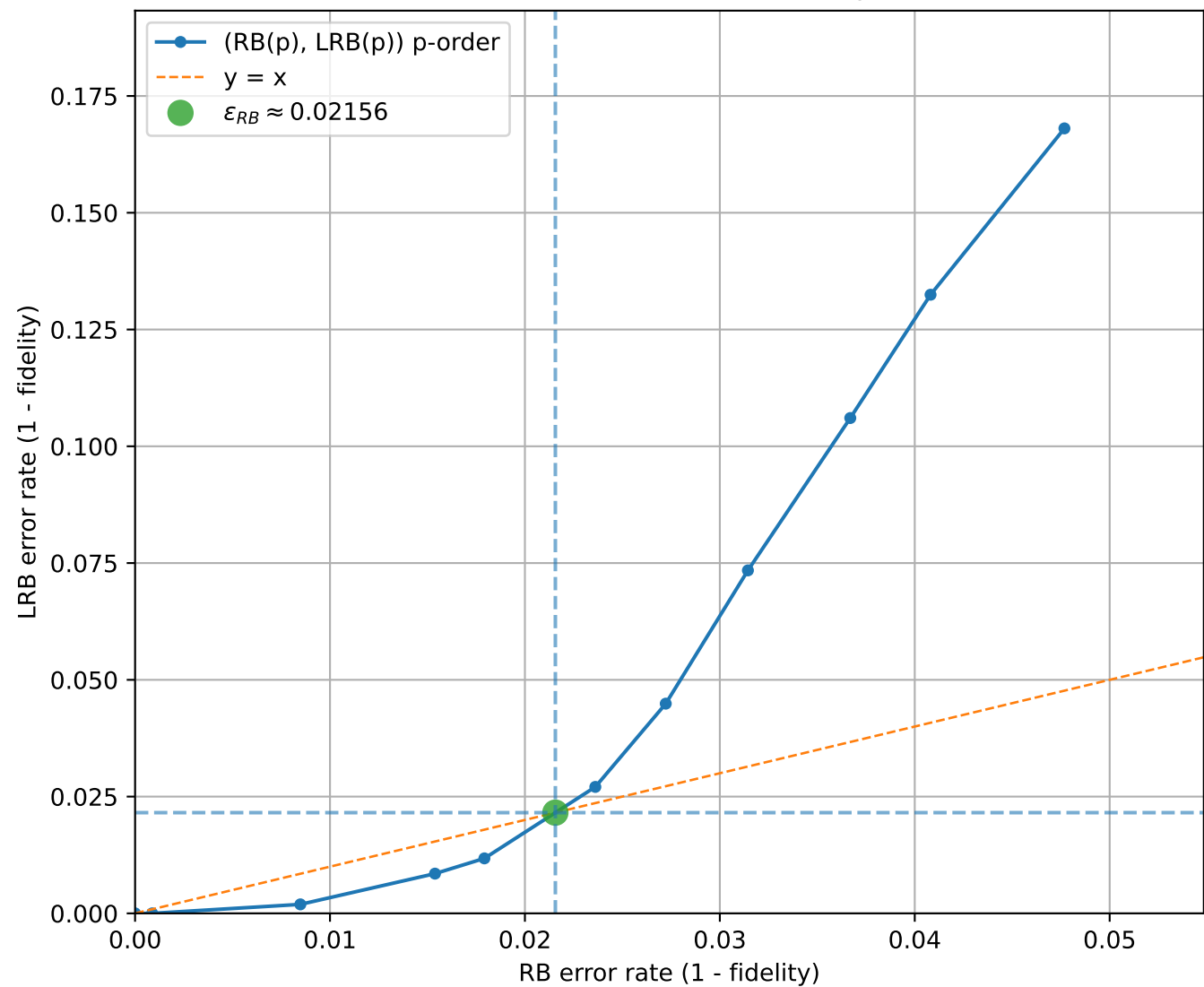
LRB vs RB (uniform interval check = 11, q=3 , [[5, 1, 2]]_3 )
