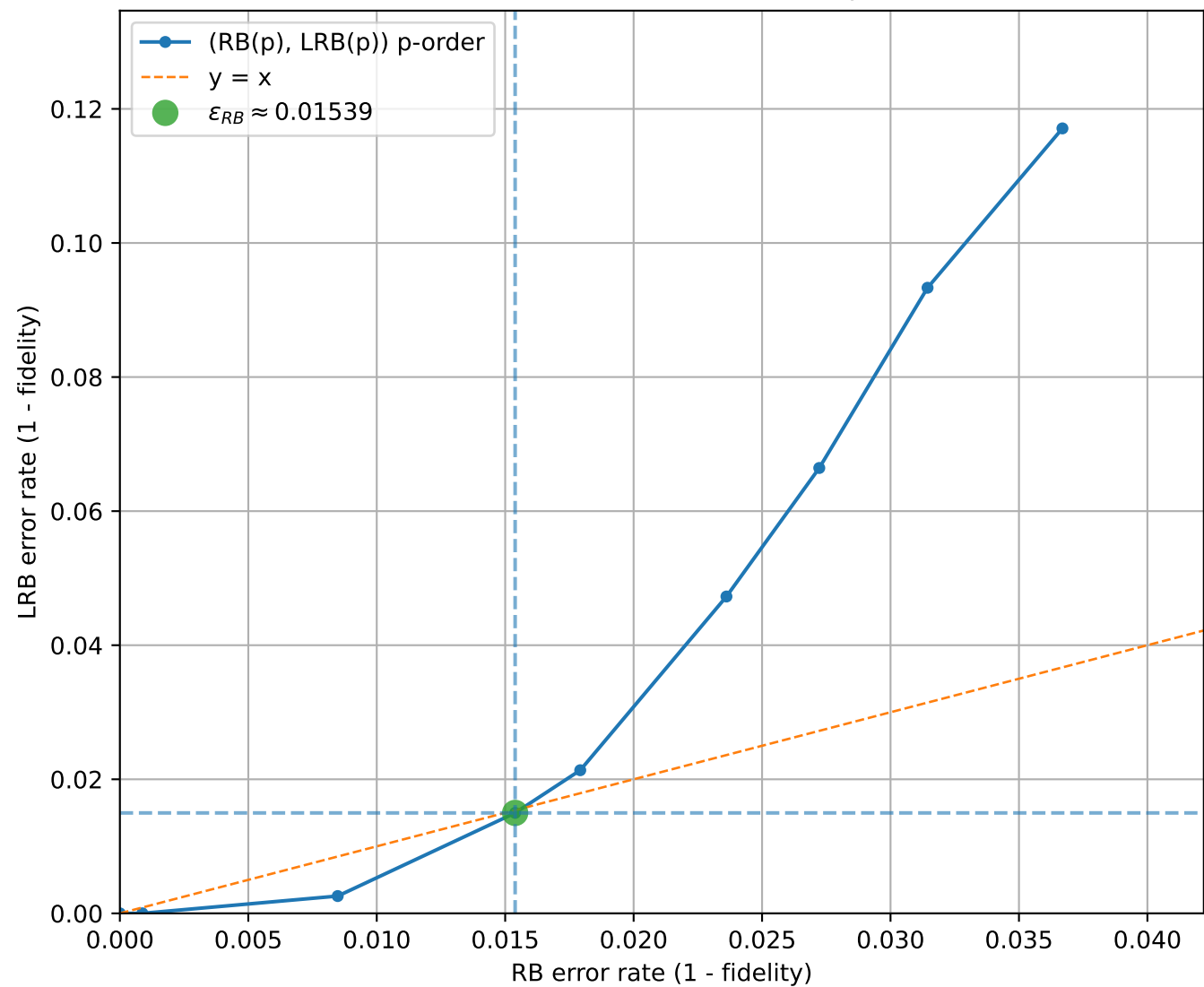
LRB vs RB (uniform interval check = 18, q=3 , [[5, 1, 2]]_3 )
