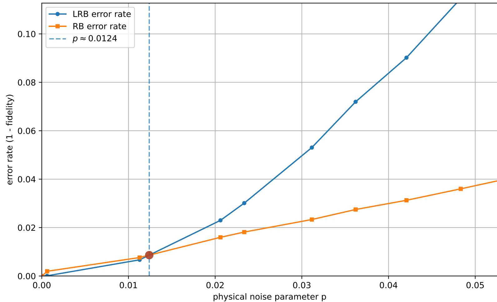
LRB vs RB (uniform interval check = 16, q=3, [[3, 1, 2]]_3 ): error rates vs p
