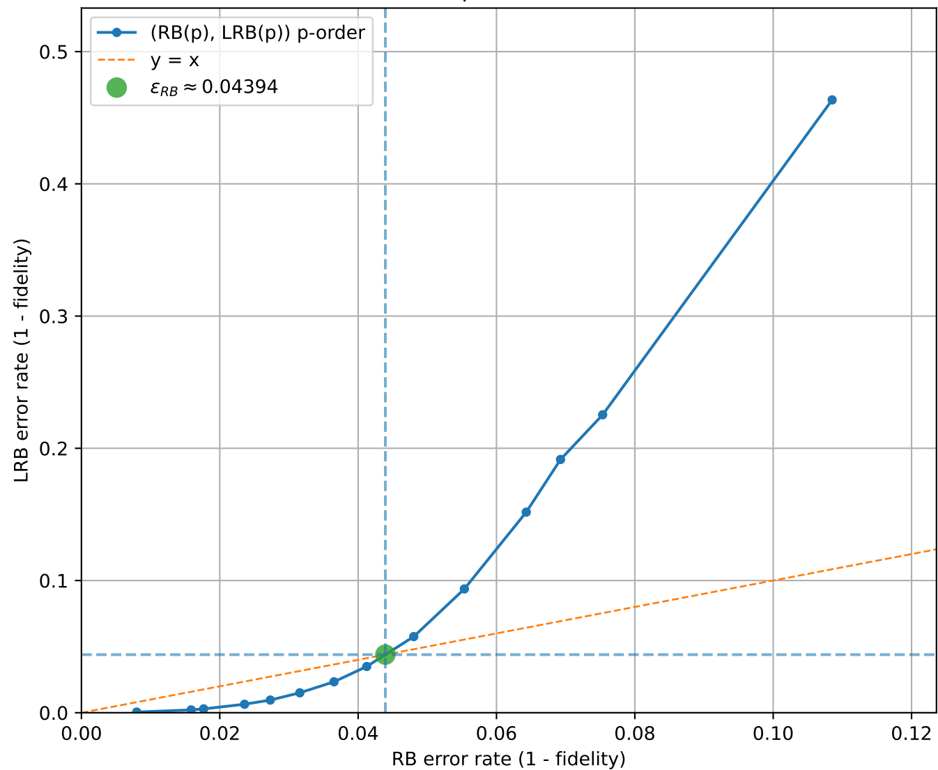
unif=4: LRB vs RB (p-window around threshold)
