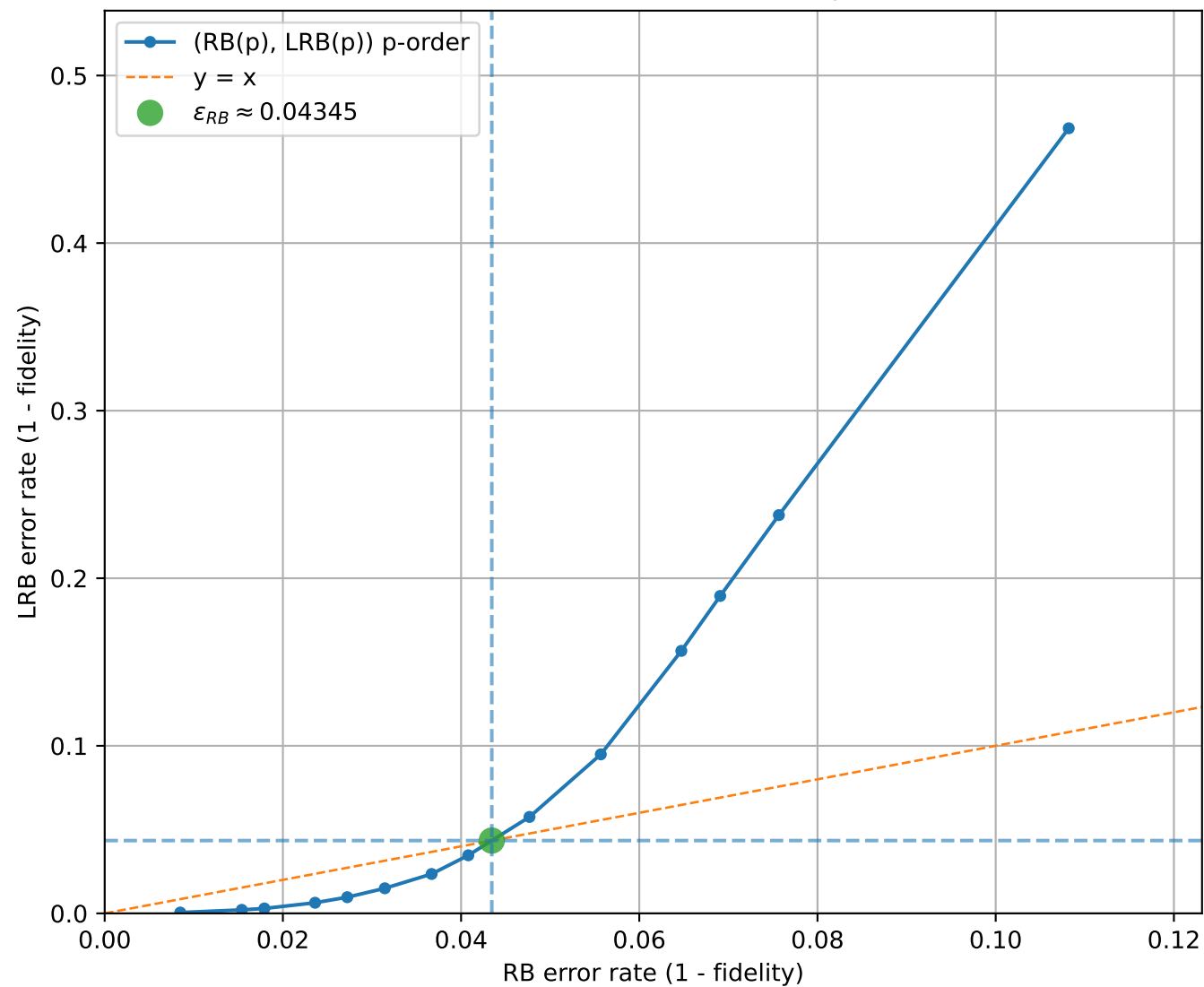
LRB vs RB (uniform interval check = 4, q=3, [[5, 1, 2]]_3 )
