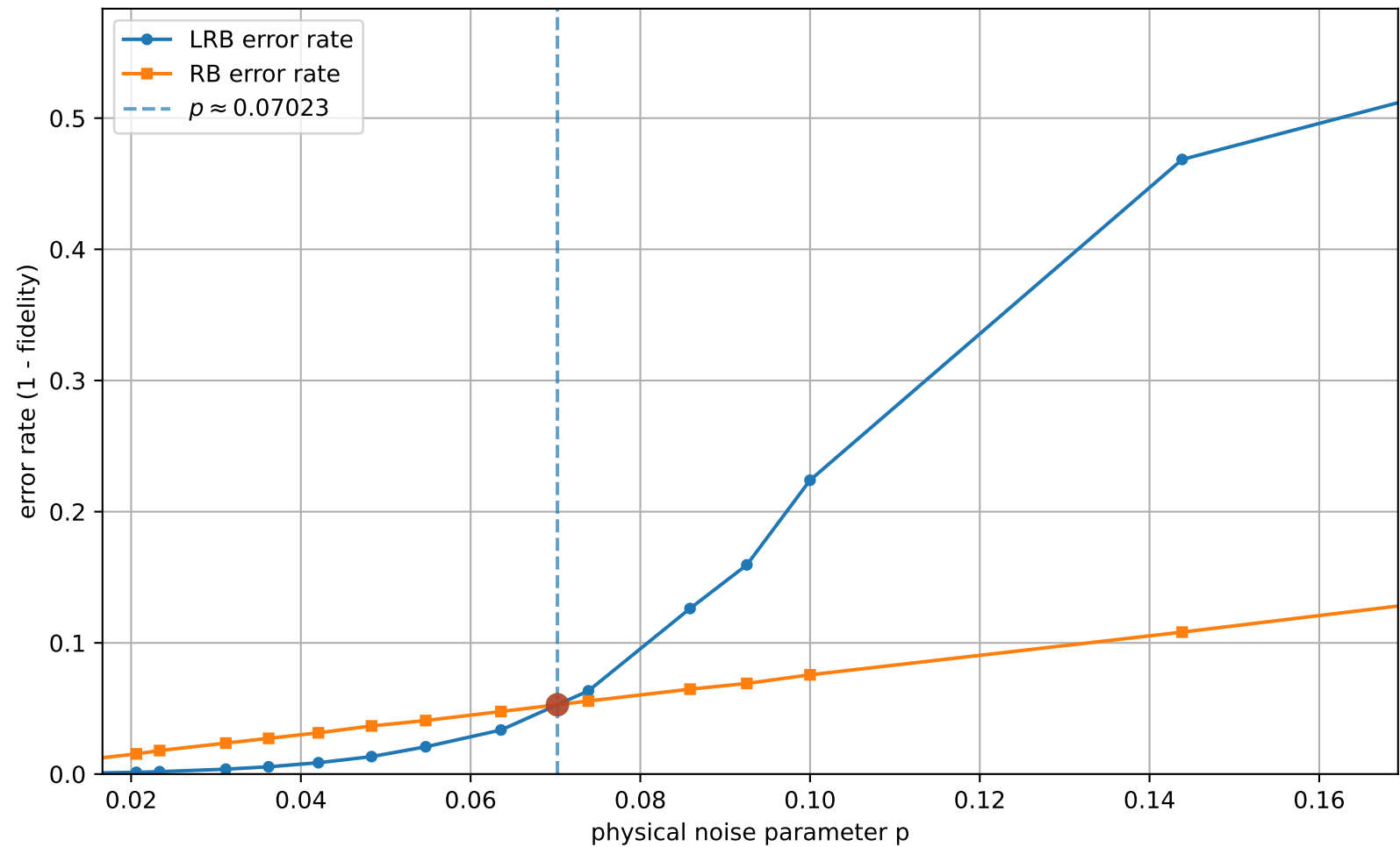
LRB vs RB (uniform interval check = 3, q=3 , [[5, 1, 2]]_3 ): error rates vs p
