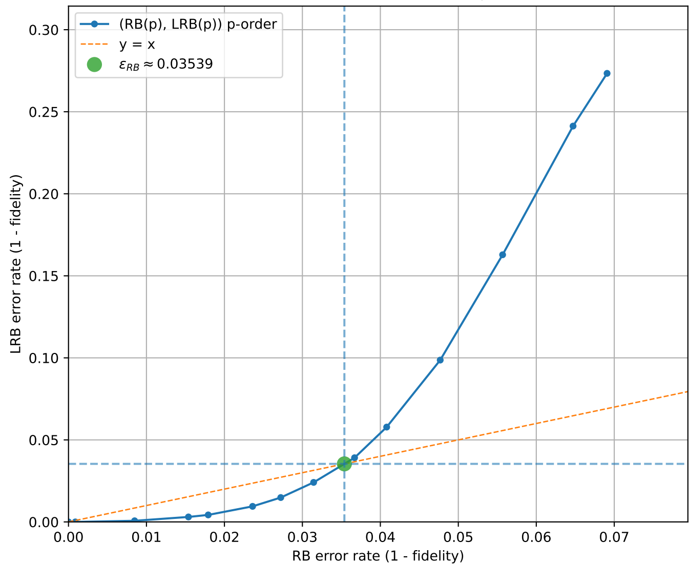
LRB vs RB (uniform interval check = 5, q=3 , [[5, 1, 2]]_3 )
