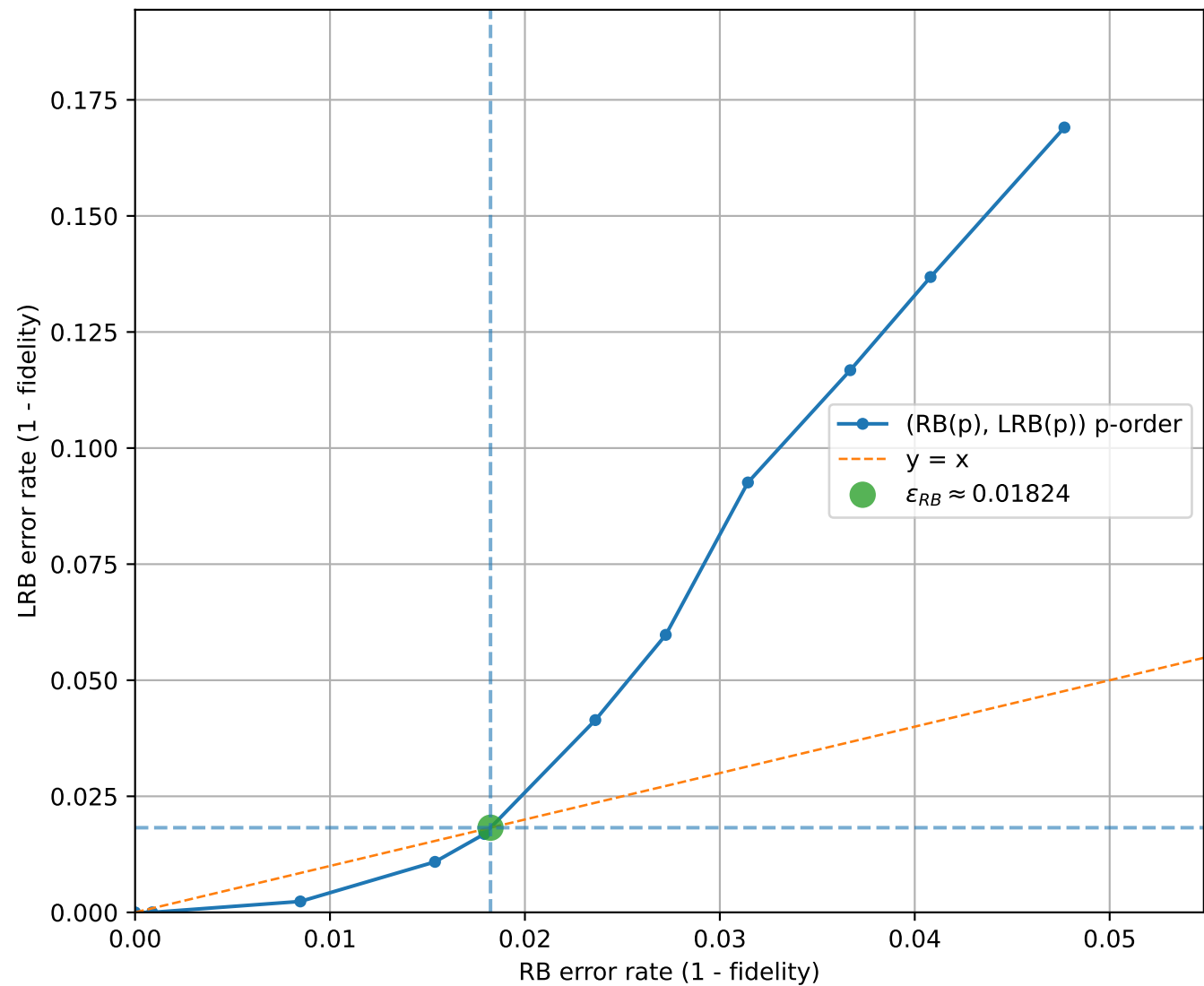
LRB vs RB (uniform interval check = 15, q=3 , [[5, 1, 2]]_3 )
