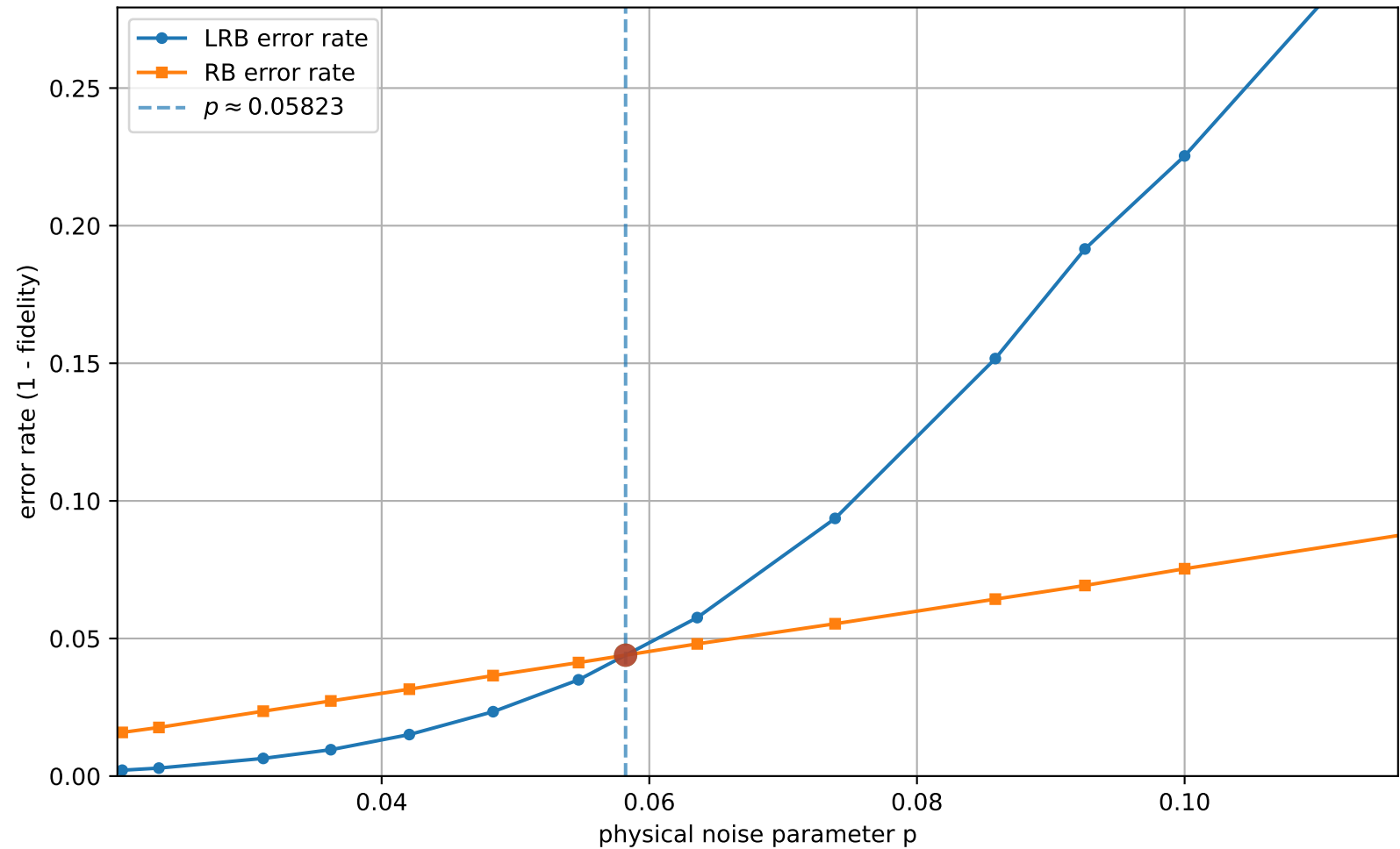
unif=4: error rates vs p (zoom near threshold)
