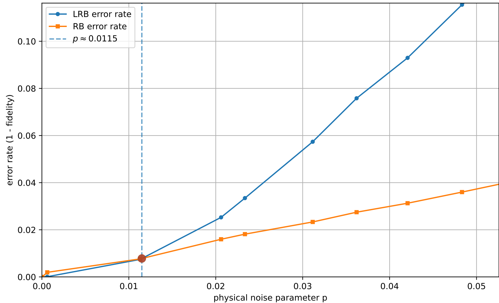
LRB vs RB (uniform interval check = 18, q=3, [[3, 1, 2]]_3 ): error rates vs p
