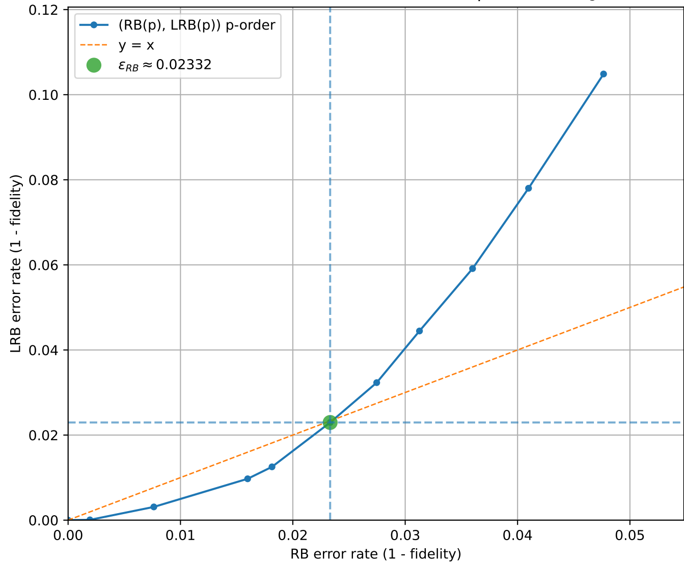
LRB vs RB (uniform interval check = 6, q=3, [[3, 1, 2]]_3 )
