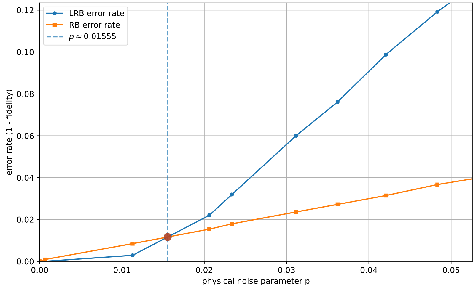
LRB vs RB (uniform interval check = 22, q=3, [[5, 1, 2]]_3 ): error rates vs p
