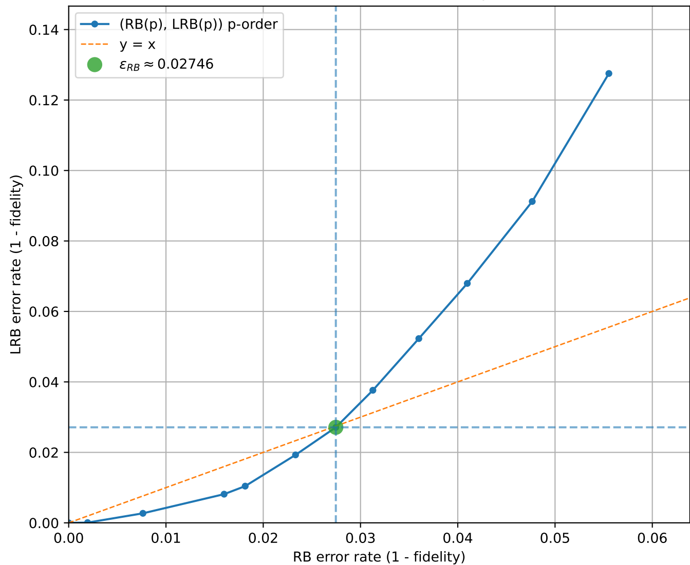
LRB vs RB (uniform interval check = 5, q=3 , [[3, 1, 2]]_3 )
