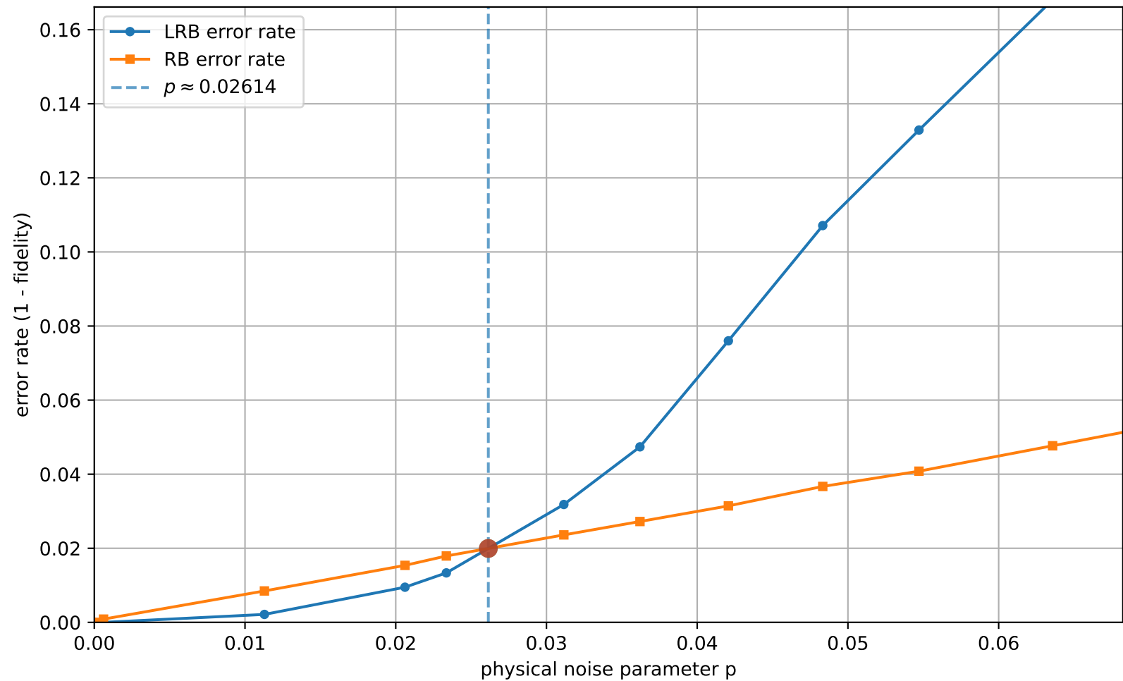
LRB vs RB (uniform interval check = 13, q=3 , [[5, 1, 2]]_3 ): error rates vs p
