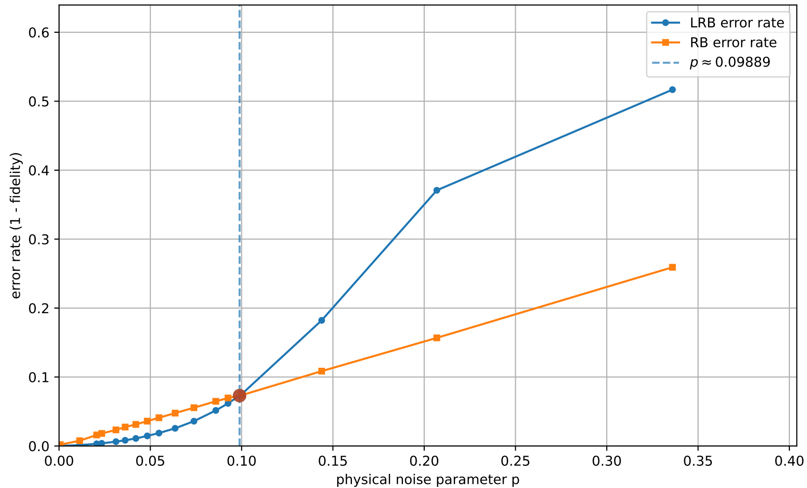
LRB vs RB (uniform interval check = 2, q=3 , [[3, 1, 2]]_3 ): error rates vs p
