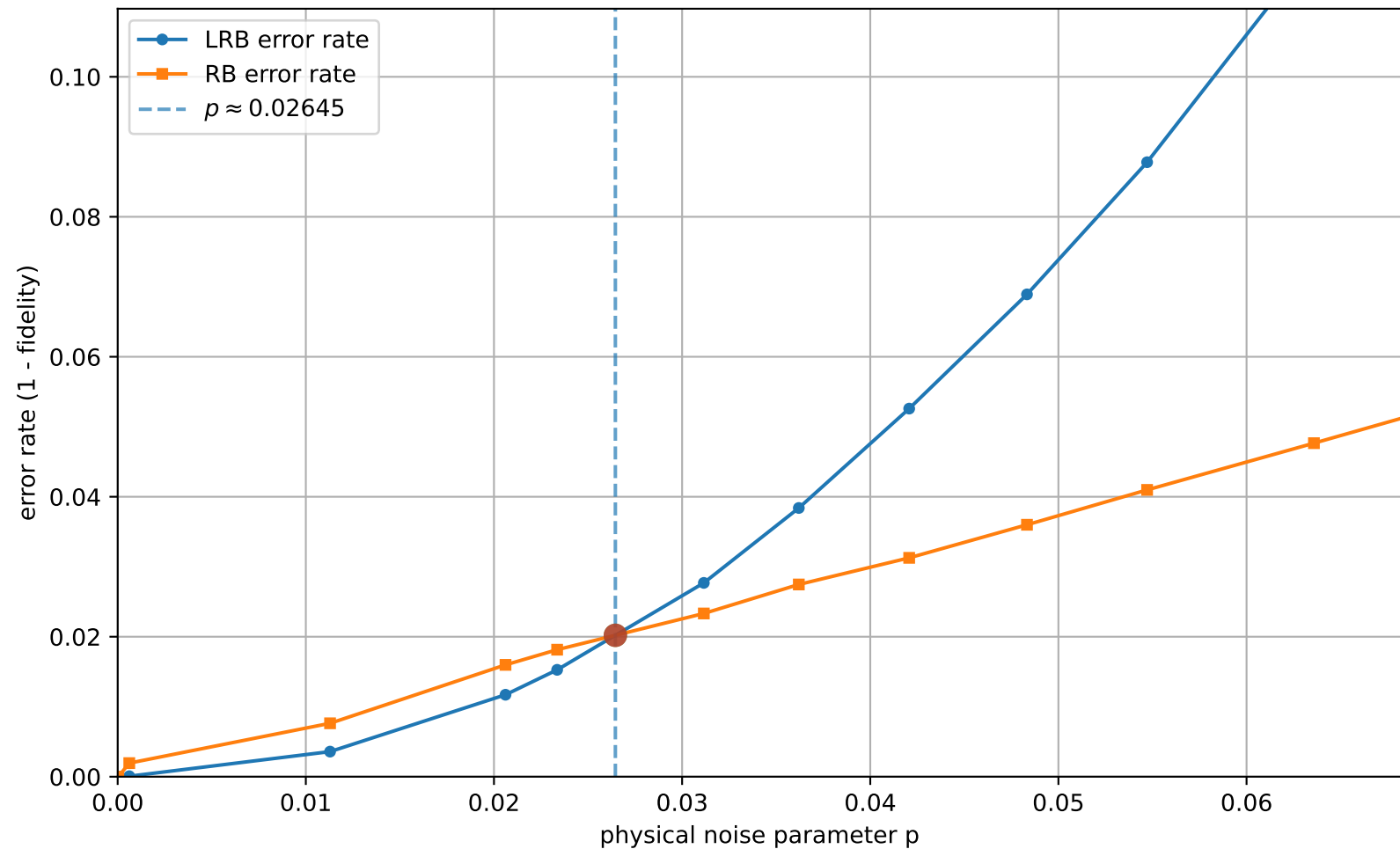
LRB vs RB (uniform interval check = 7, q=3, [[3, 1, 2]]_3 ): error rates vs p
