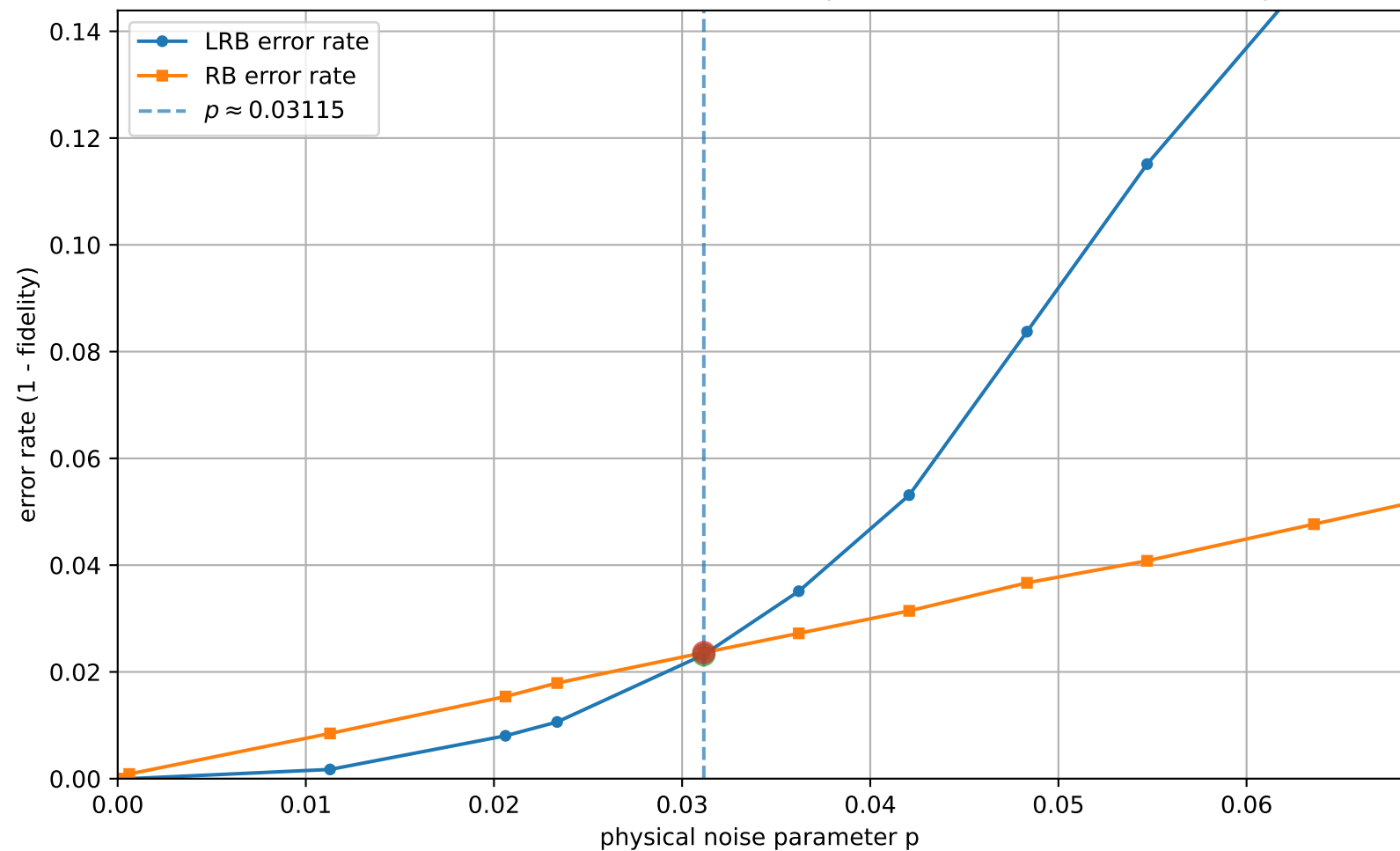
LRB vs RB (uniform interval check = 10, q=3, [[5, 1, 2]]_3 ): error rates vs p
