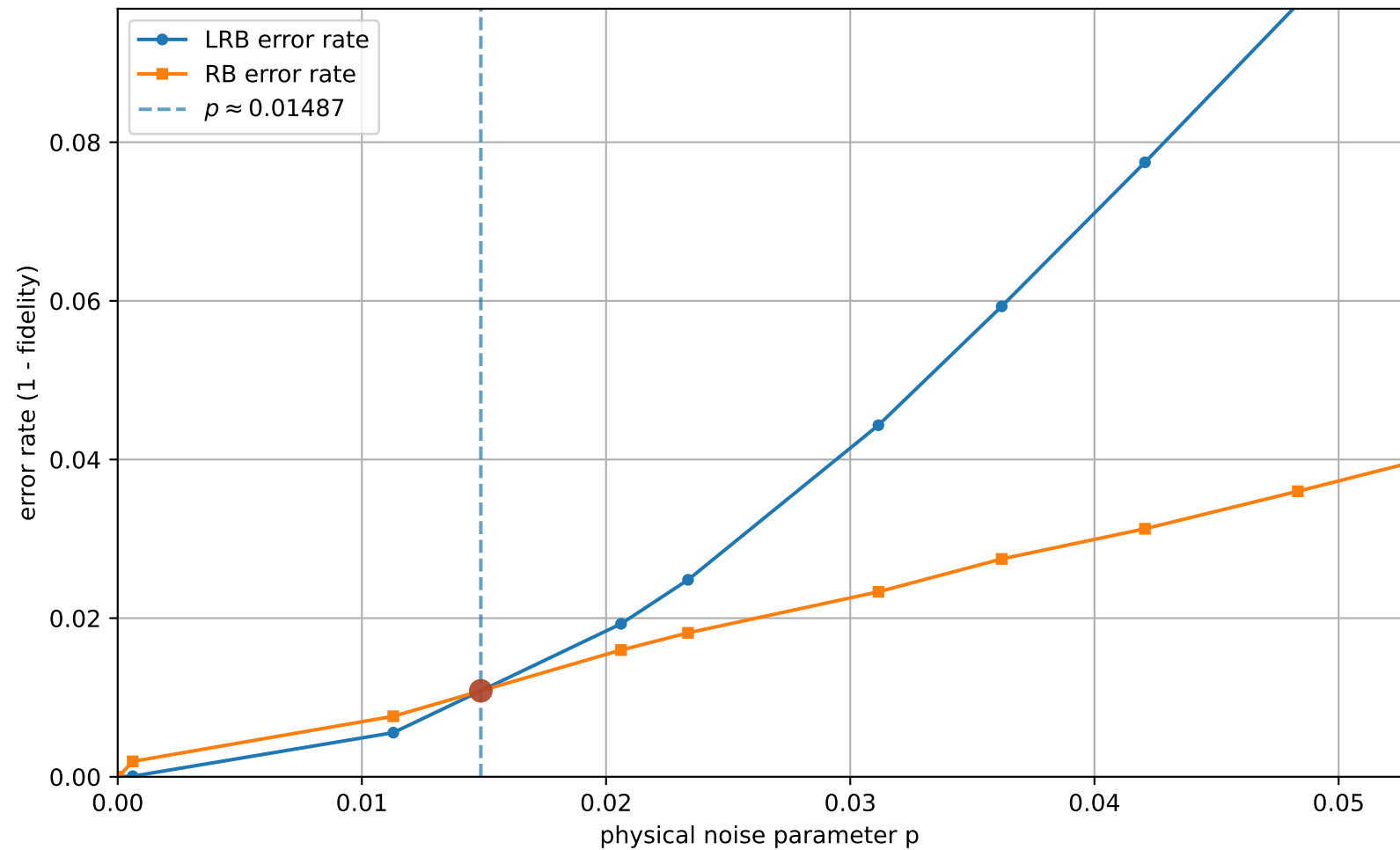
LRB vs RB (uniform interval check = 12, q=3, [[3, 1, 2]]_3 ): error rates vs p
