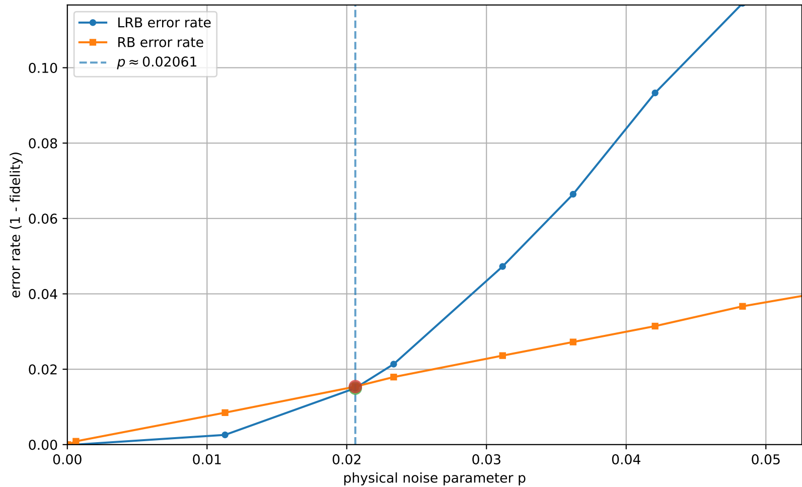
LRB vs RB (uniform interval check = 18, q=3, [[5, 1, 2]]_3 ): error rates vs p
