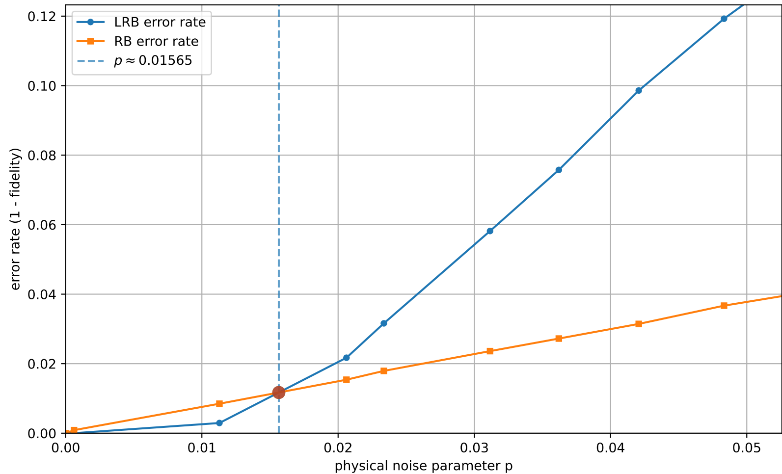
LRB vs RB (uniform interval check = 21, q=3, [[5, 1, 2]]_3 ): error rates vs p
