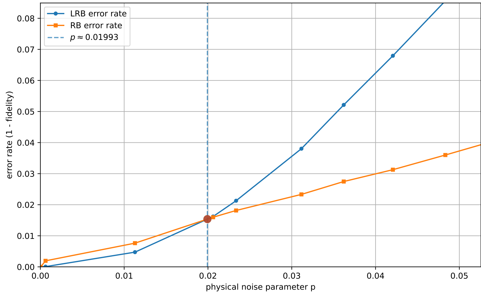
LRB vs RB (uniform interval check = 10, q=3 , [[3, 1, 2]]_3 ): error rates vs p
