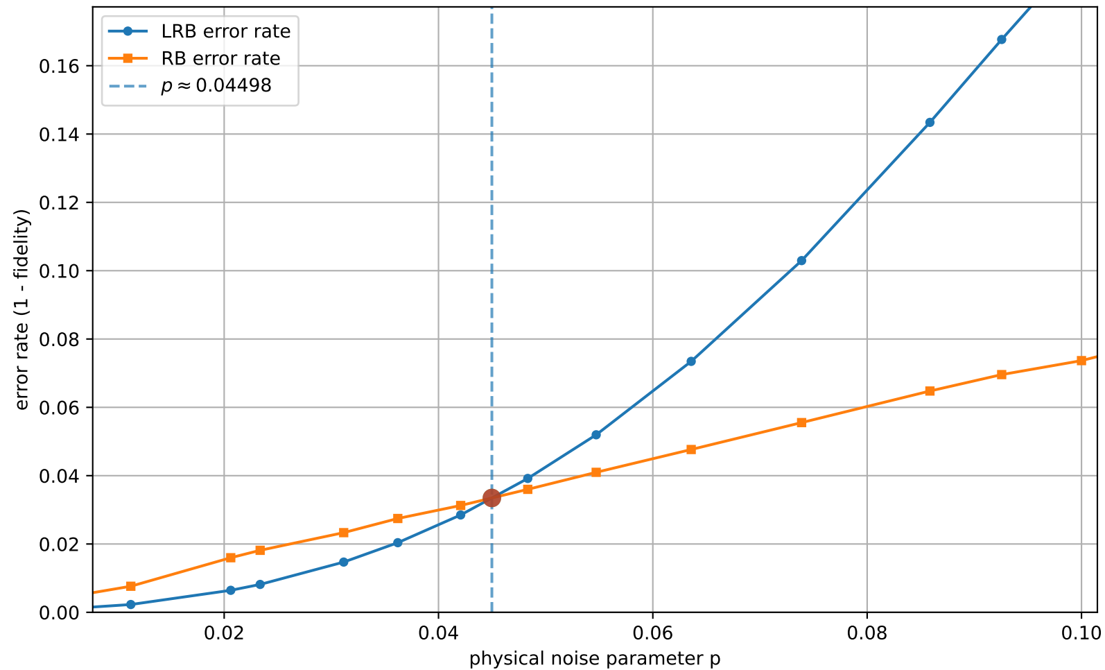
LRB vs RB (uniform interval check = 4, q=3, [[3, 1, 2]]_3 ): error rates vs p
