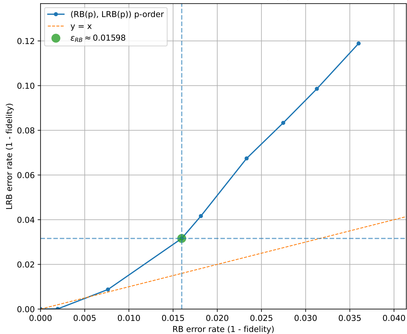
LRB vs RB (uniform interval check = 22, q=3 , [[3, 1, 2]]_3 )
