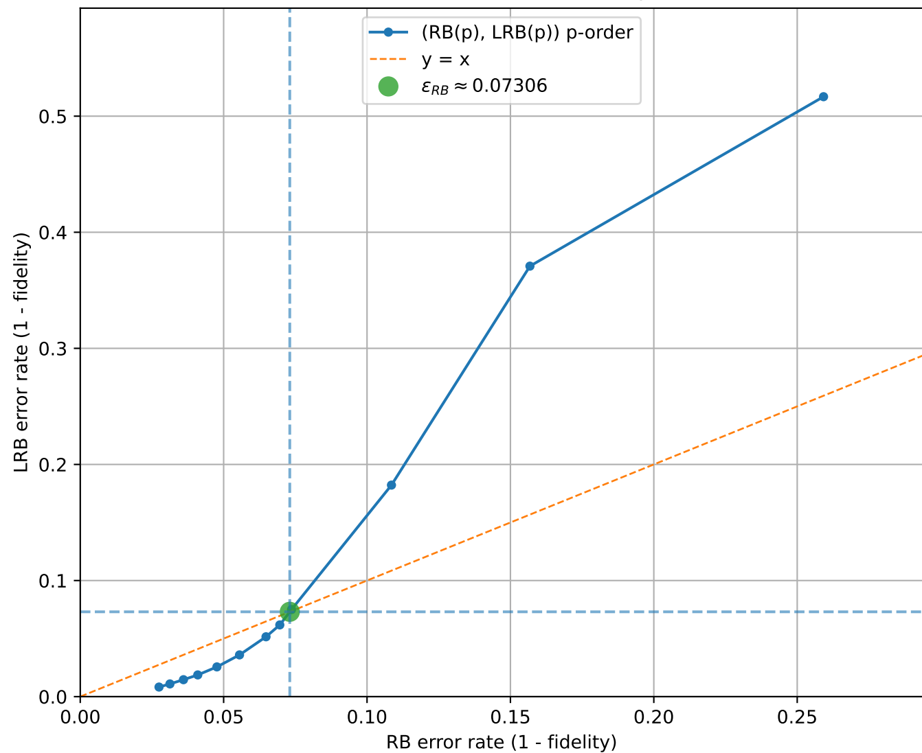
LRB vs RB (uniform interval check = 2, q=3, [[3, 1, 2]]_3 )
