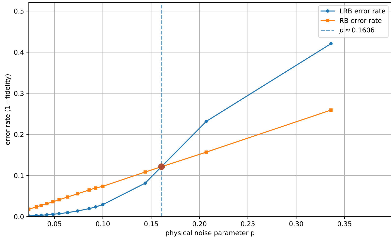
LRB vs RB (uniform interval check = 1, q=3 , [[3, 1, 2]]_3 ): error rates vs p
