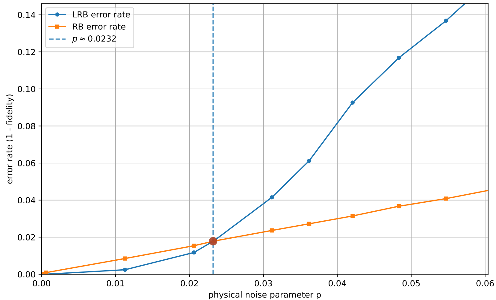
LRB vs RB (uniform interval check = 16, q=3, [[5, 1, 2]]_3 ): error rates vs p
