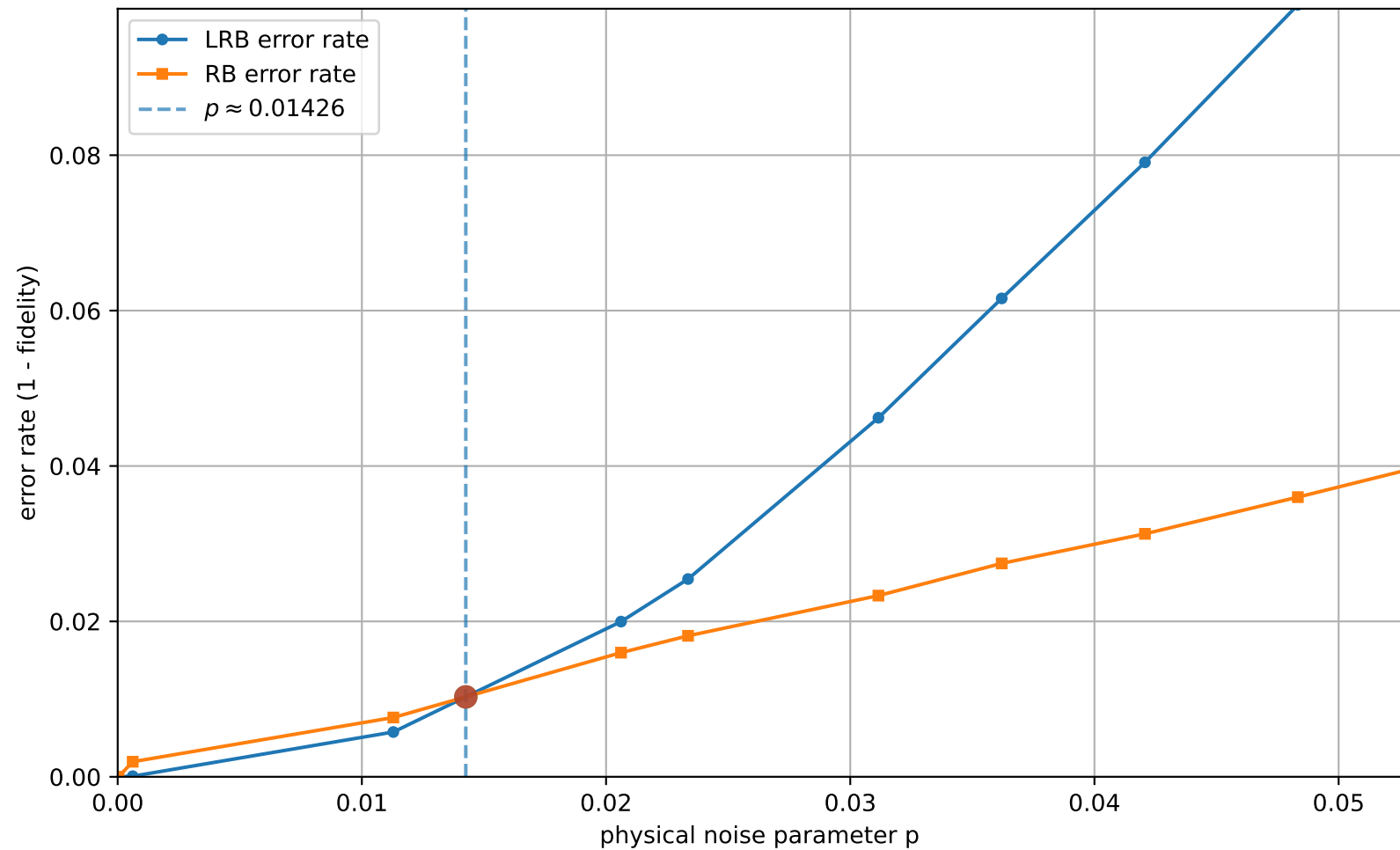
LRB vs RB (uniform interval check = 13, q=3 , [[3, 1, 2]]_3 ): error rates vs p
