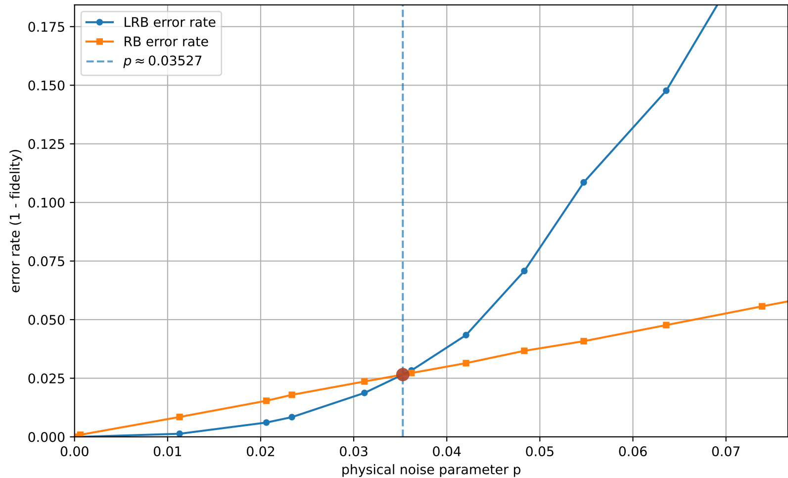
LRB vs RB (uniform interval check = 8, q=3, [[5, 1, 2]]_3 ): error rates vs p
