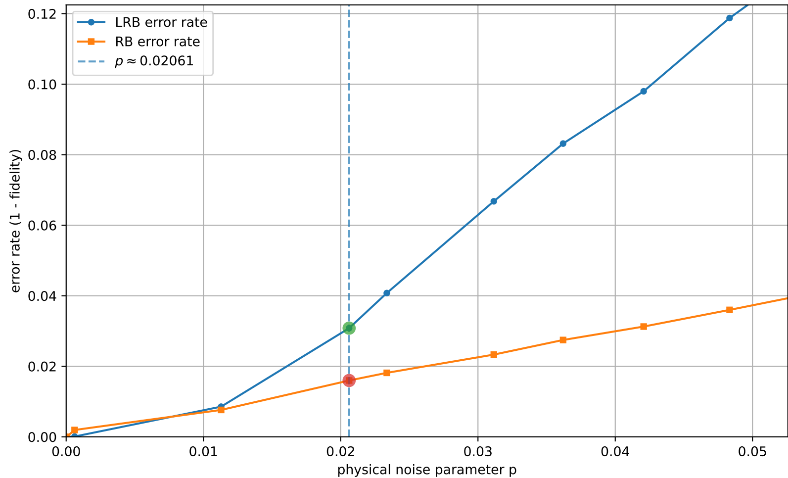
LRB vs RB (uniform interval check = 21, q=3, [[3, 1, 2]]_3 ): error rates vs p
