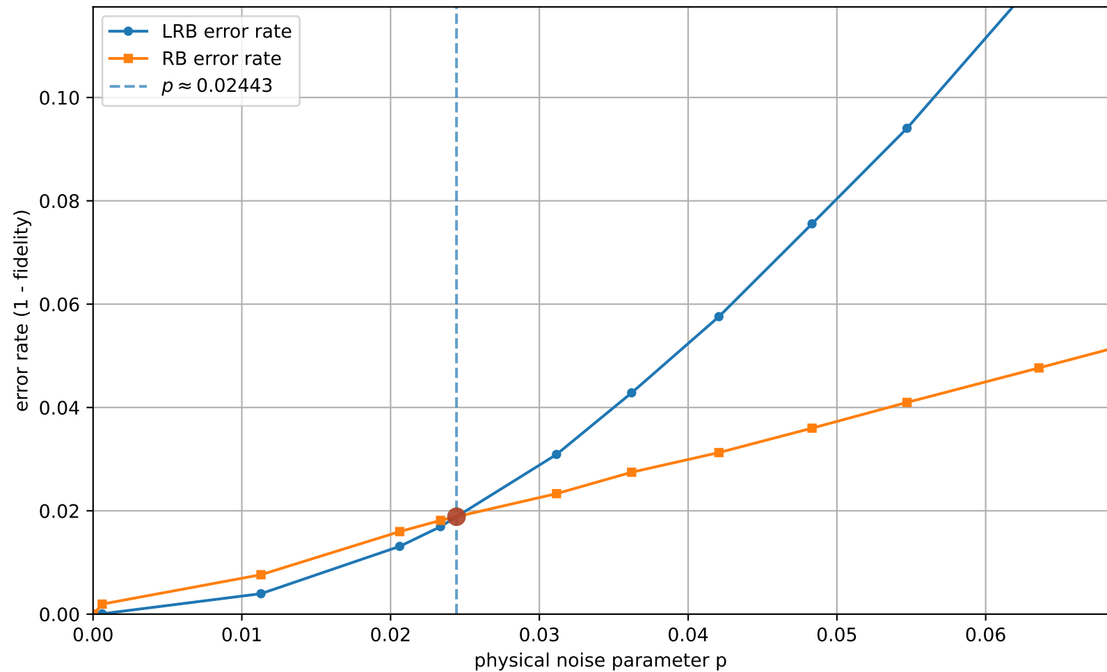
LRB vs RB (uniform interval check = 8, q=3, [[3, 1, 2]]_3 ): error rates vs p
