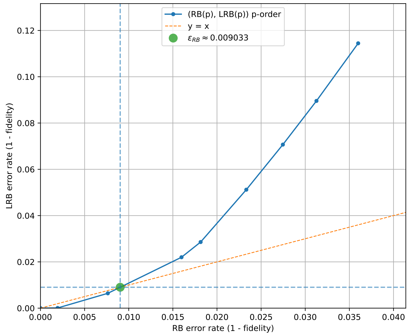
LRB vs RB (uniform interval check = 15, q=3 , [[3, 1, 2]]_3 )
