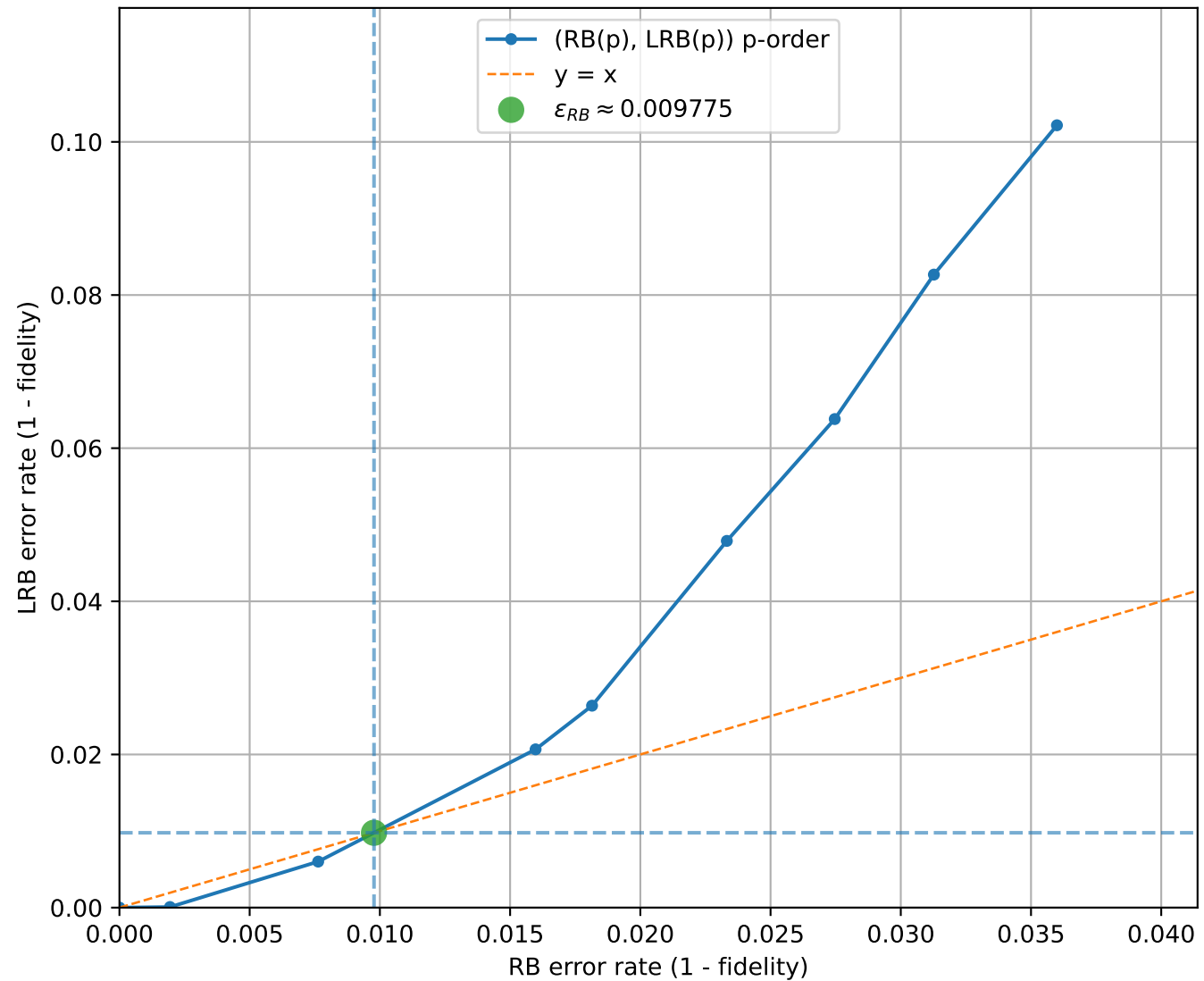
LRB vs RB (uniform interval check = 14, q=3 , [[3, 1, 2]]_3 )
