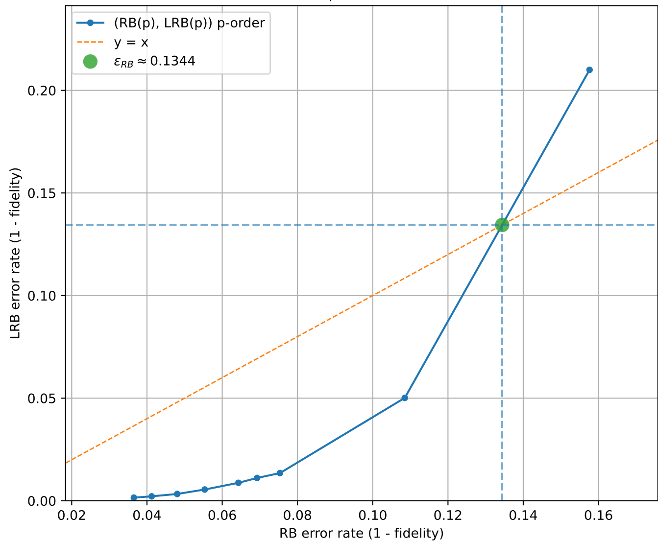
unif=1: LRB vs RB (p-window around threshold)
