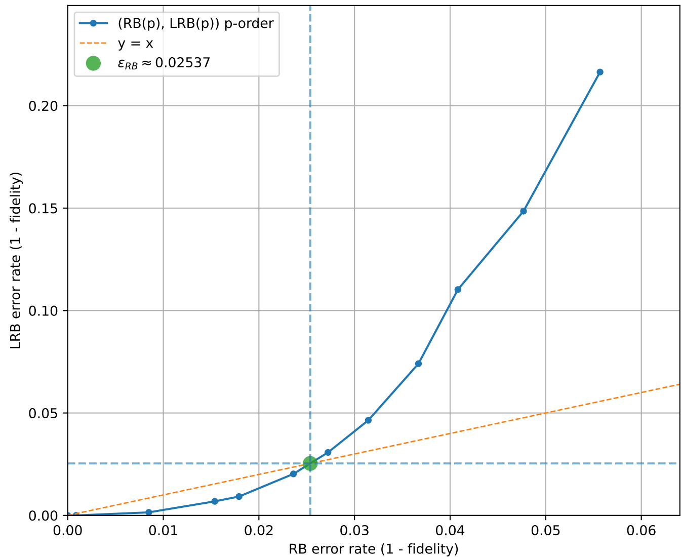
LRB vs RB (uniform interval check = 9, q=3, [[5, 1, 2]]_3 )
