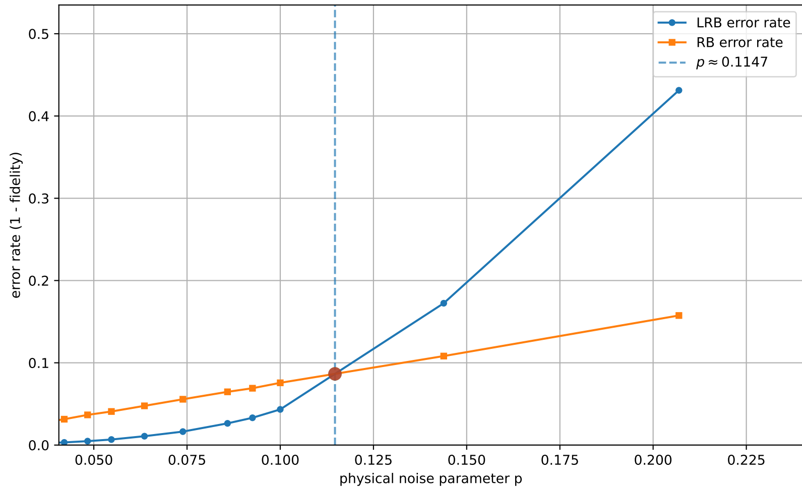
LRB vs RB (uniform interval check = 2, q=3 , [[5, 1, 2]]_3 ): error rates vs p
