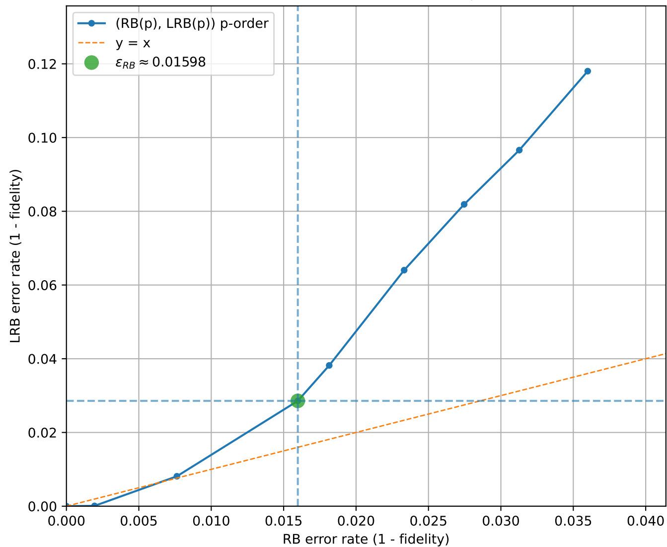
LRB vs RB (uniform interval check = 20, q=3 , [[3, 1, 2]]_3 )
