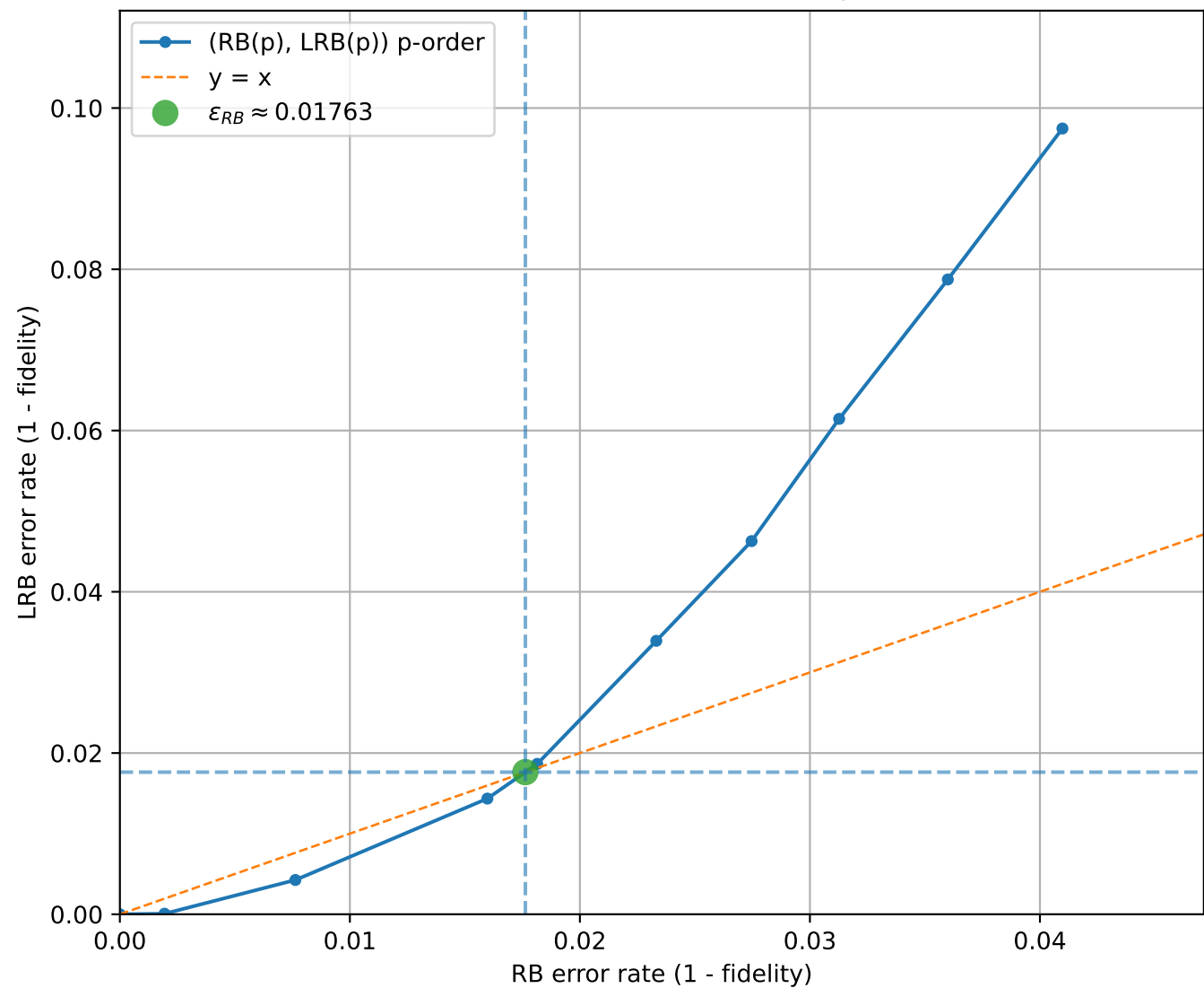
LRB vs RB (uniform interval check = 9, q=3, [[3, 1, 2]]_3 )
