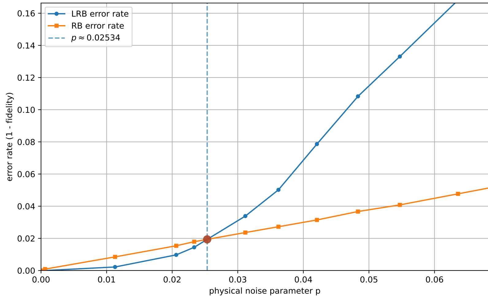
LRB vs RB (uniform interval check = 14, q=3 , [[5, 1, 2]]_3 ): error rates vs p
