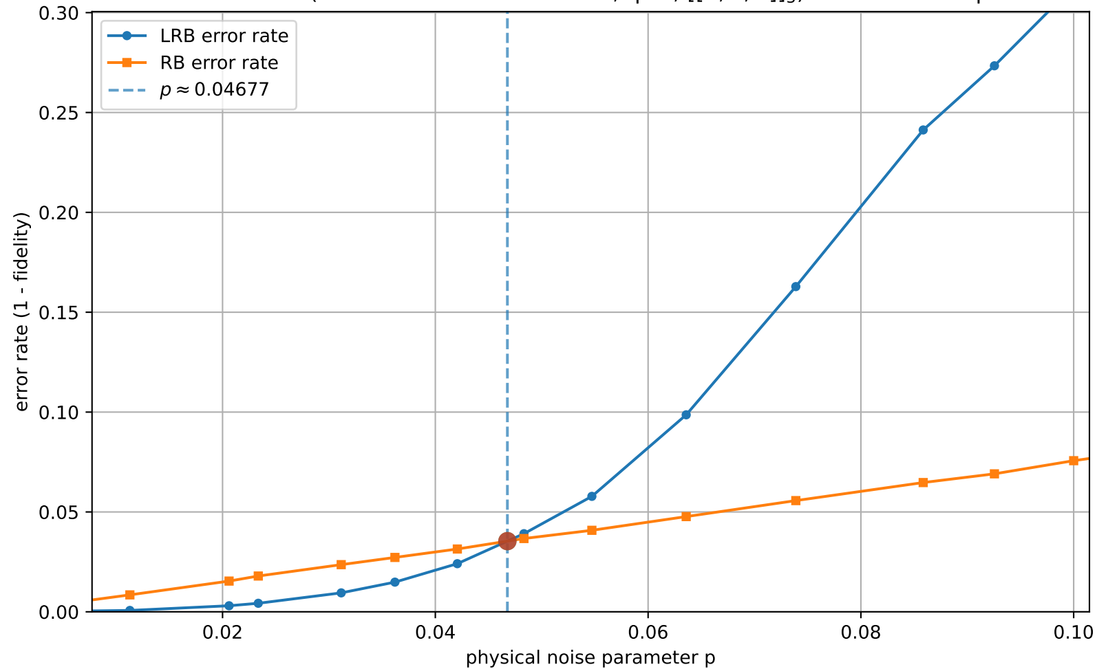
LRB vs RB (uniform interval check = 5, q=3 , [[5, 1, 2]]_3 ): error rates vs p
