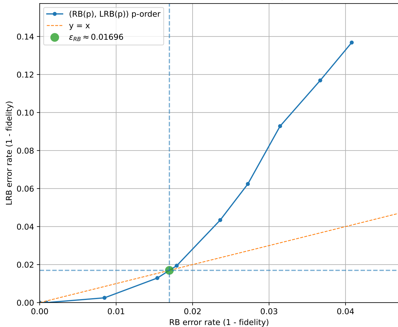
LRB vs RB (uniform interval check = 17, q=3 , [[5, 1, 2]]_3 )
