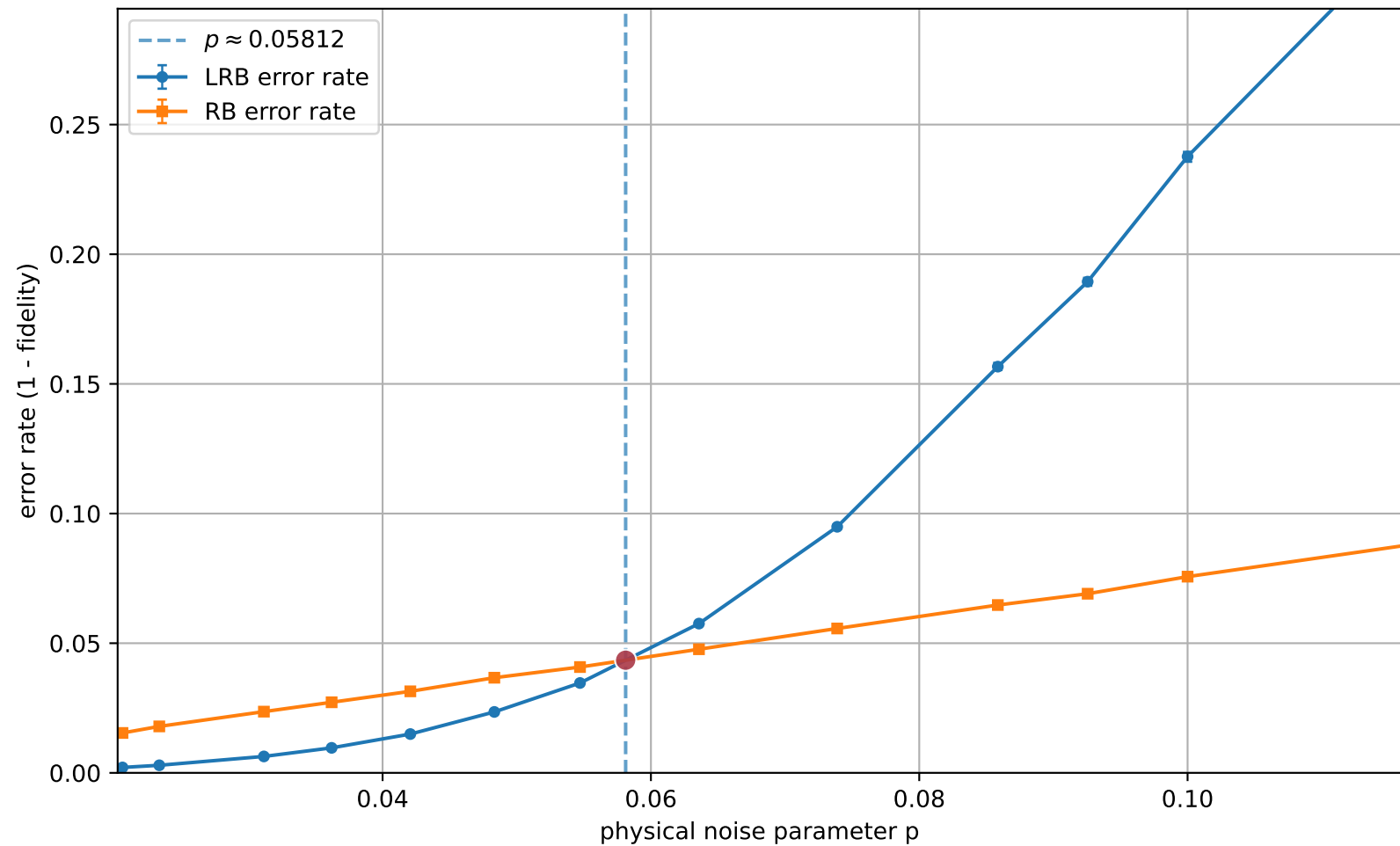
LRB vs RB (uniform interval check = 4, q=3 , [[5, 1, 2]]_3 ): error rates vs p
