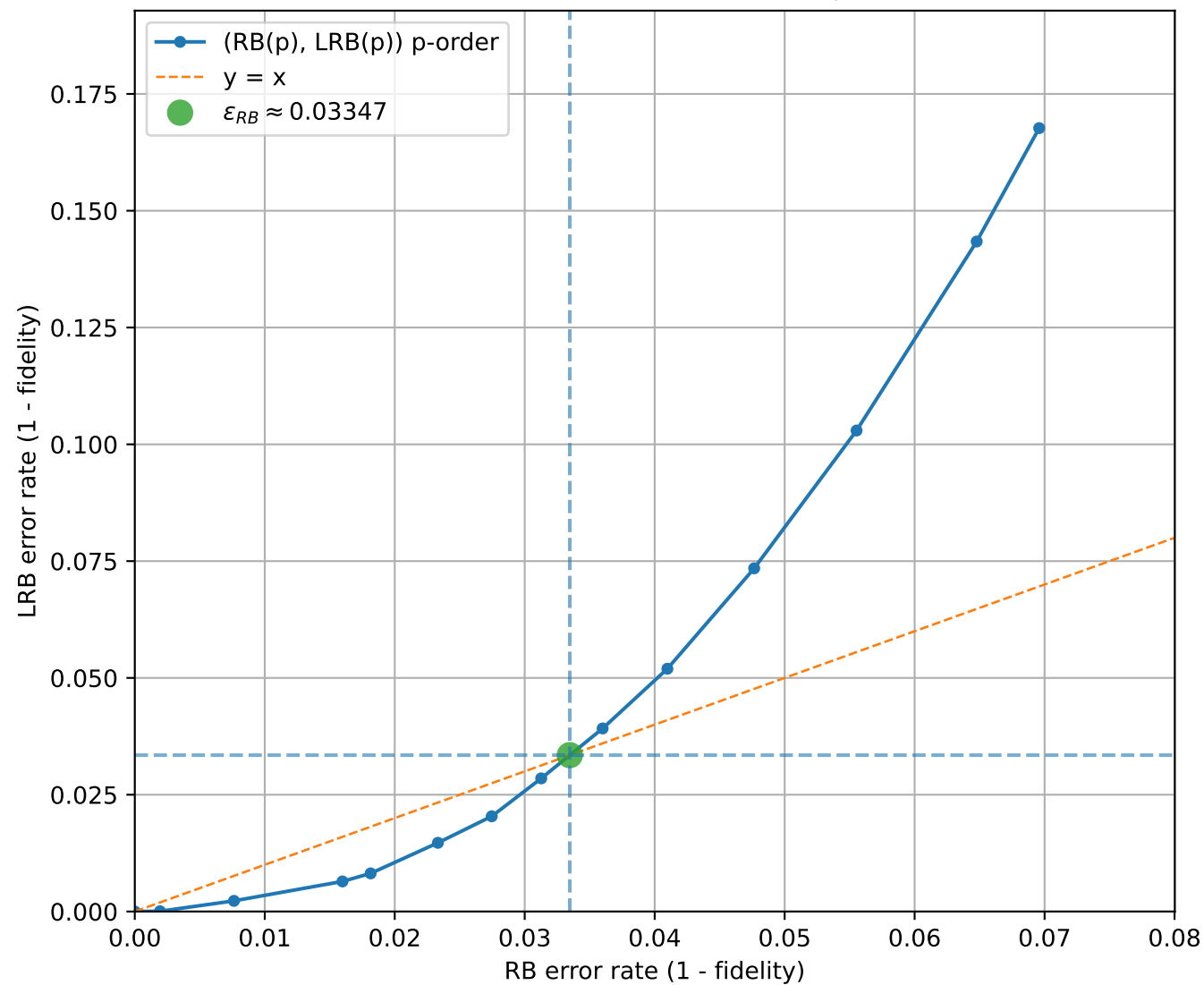
LRB vs RB (uniform interval check = 4, q=3, [[3, 1, 2]]_3 )
