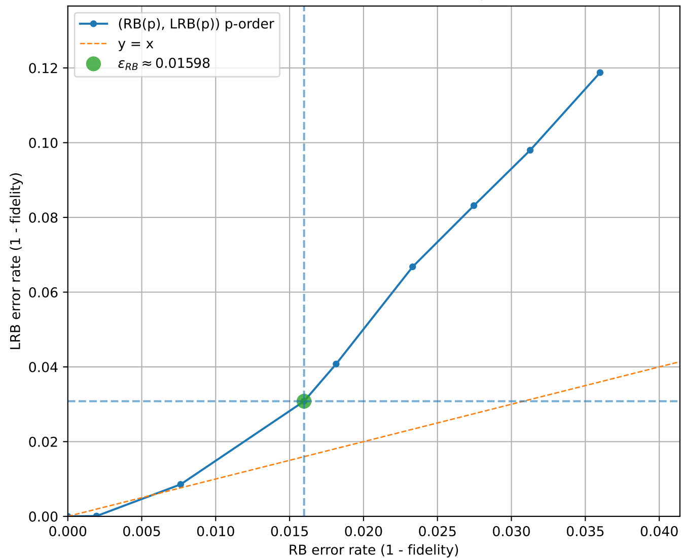
LRB vs RB (uniform interval check = 21, q=3 , [[3, 1, 2]]_3 )
