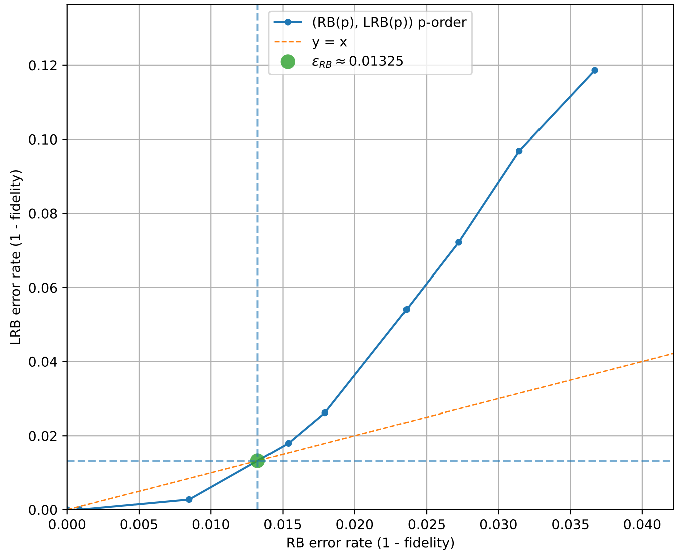
LRB vs RB (uniform interval check = 19, q=3 , [[5, 1, 2]]_3 )
