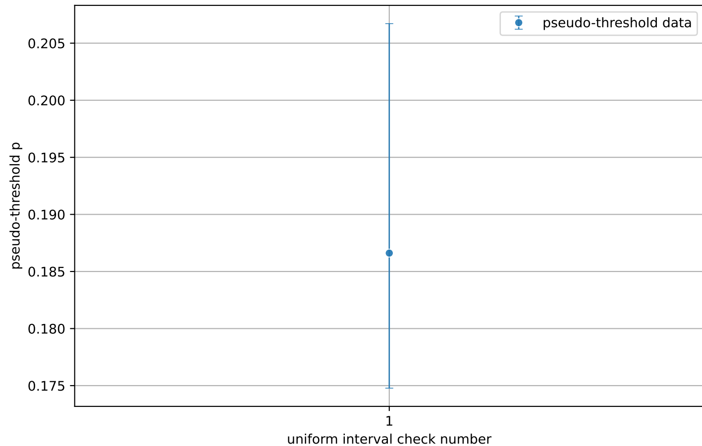
Pseudo-threshold vs uniform interval check ( q=3 , [[5, 1, 2]]_3 )
