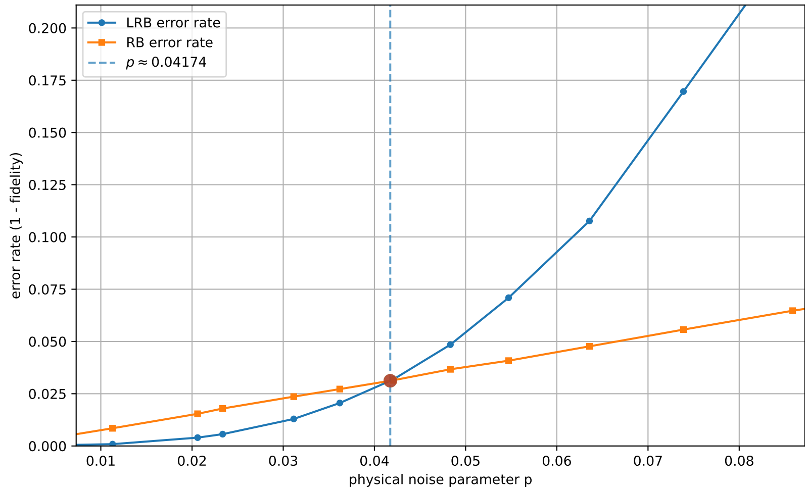
LRB vs RB (uniform interval check = 6, q=3 , [[5, 1, 2]]_3 ): error rates vs p
