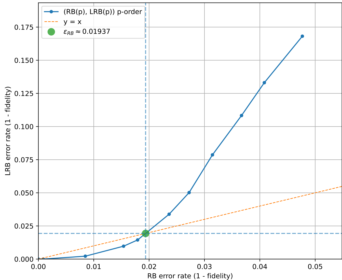
LRB vs RB (uniform interval check = 14, q=3 , [[5, 1, 2]]_3 )
