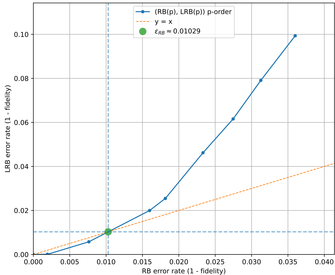
LRB vs RB (uniform interval check = 13, q=3 , [[3, 1, 2]]_3 )
