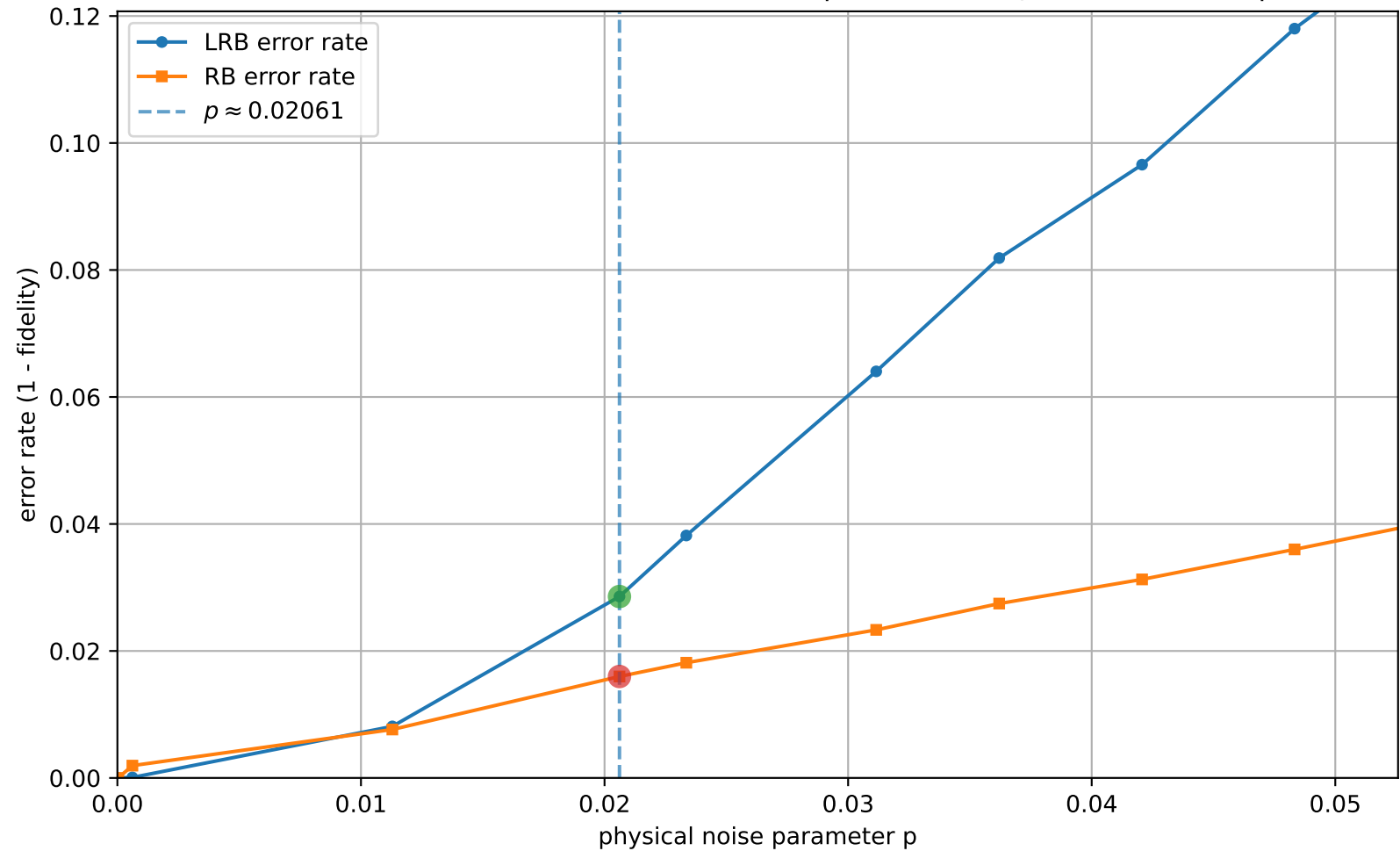
LRB vs RB (uniform interval check = 20, q=3, [[3, 1, 2]]_3 ): error rates vs p
