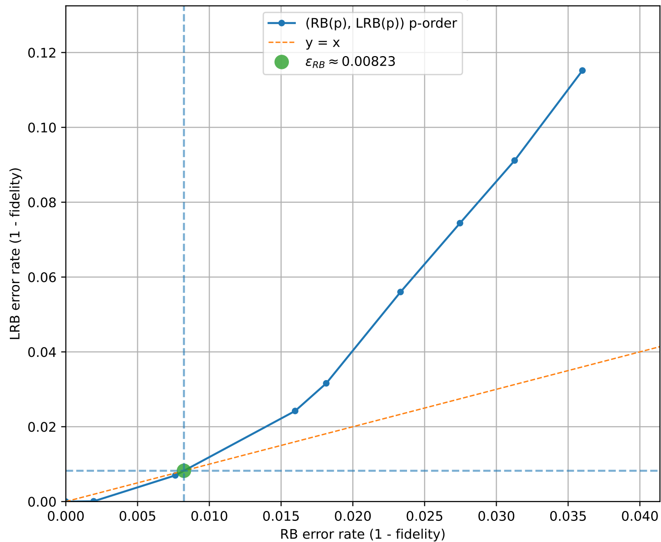
LRB vs RB (uniform interval check = 17, q=3 , [[3, 1, 2]]_3 )
