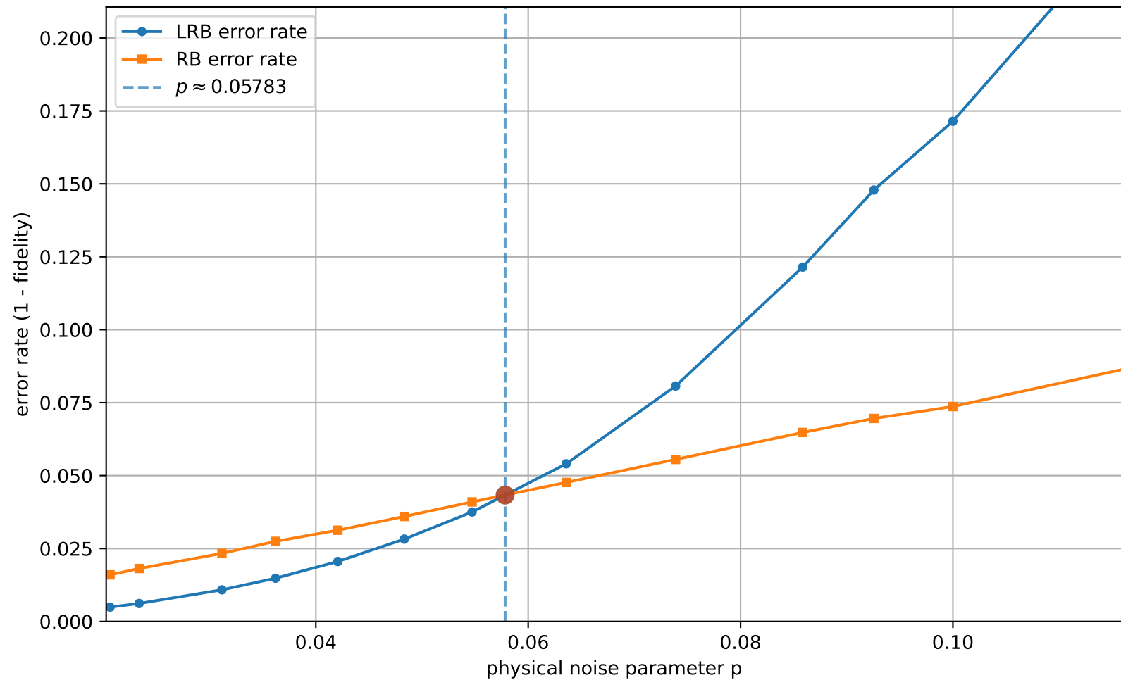
LRB vs RB (uniform interval check = 3, q=3 , [[3, 1, 2]]_3 ): error rates vs p
