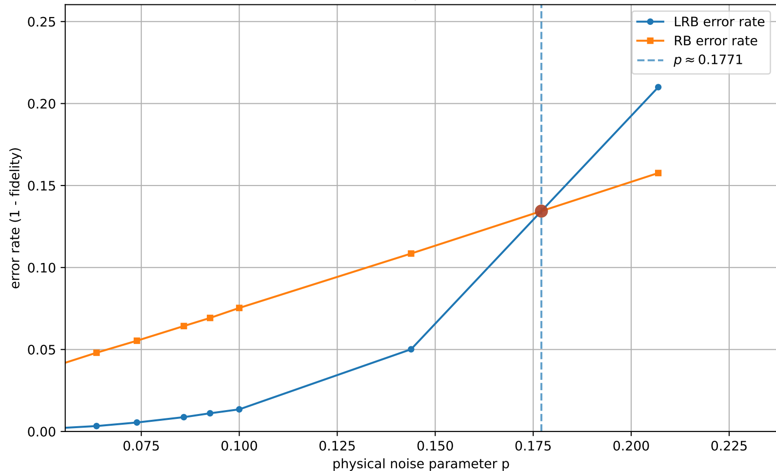
unif=1: error rates vs p (zoom near threshold)
