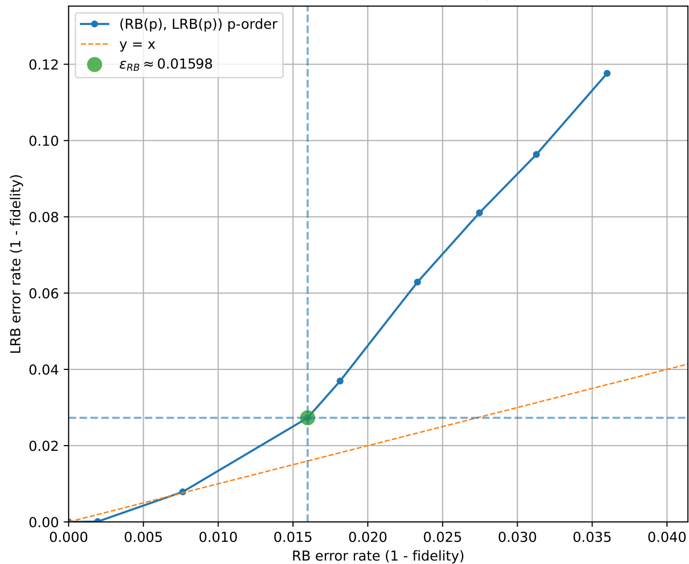
LRB vs RB (uniform interval check = 19, q=3 , [[3, 1, 2]]_3 )
