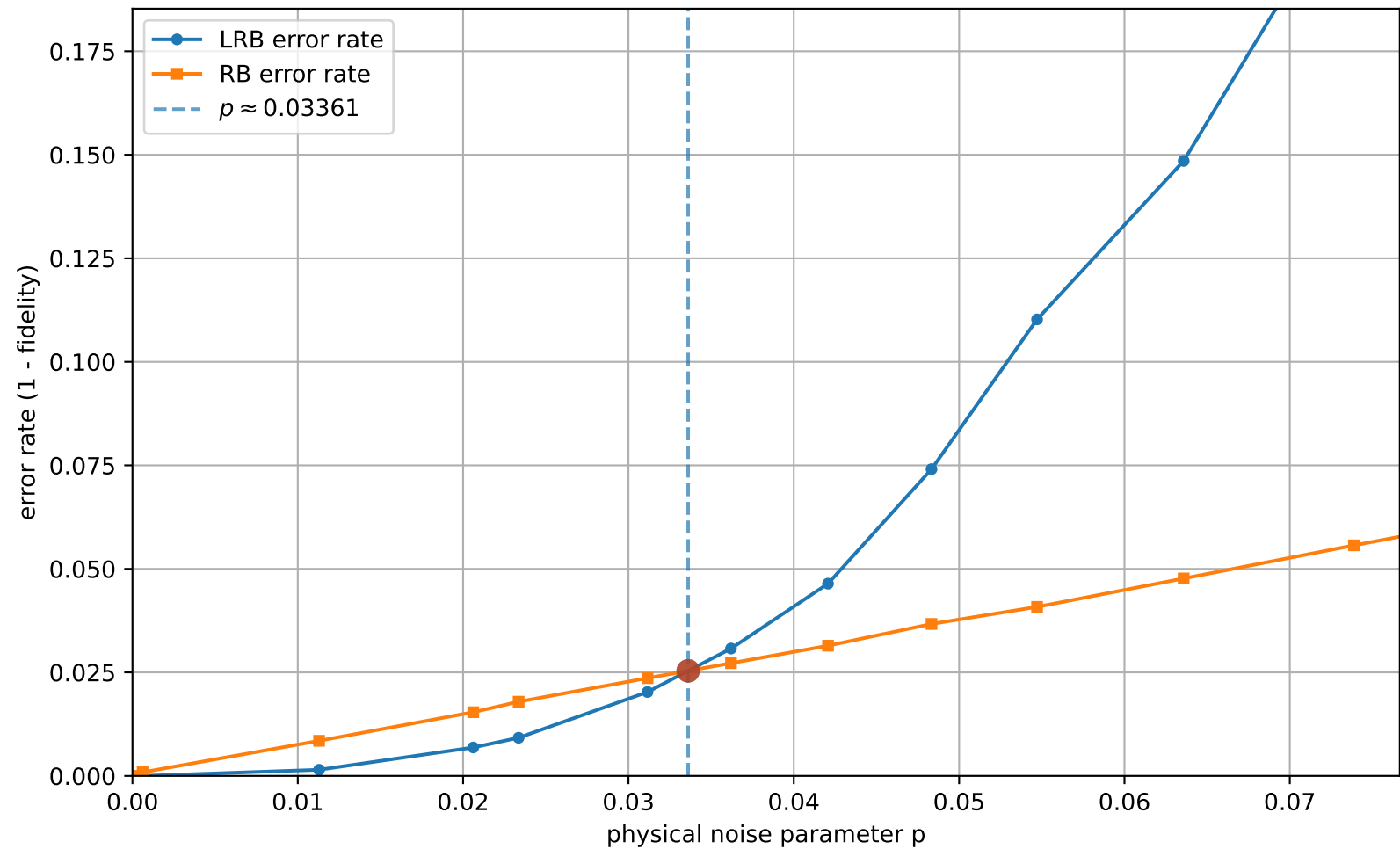
LRB vs RB (uniform interval check = 9, q=3, [[5, 1, 2]]_3 ): error rates vs p
