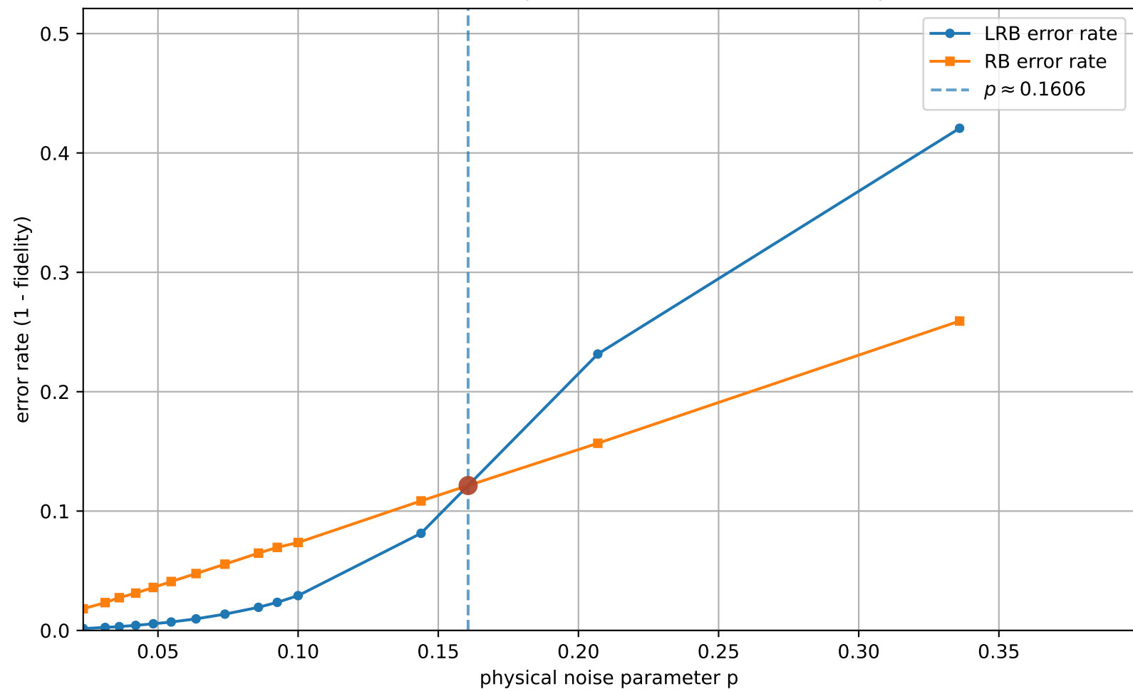
LRB vs RB (uniform interval check = 1, q=3 , [[3, 1, 2]]_3 ): error rates vs p (zoom near threshold)
