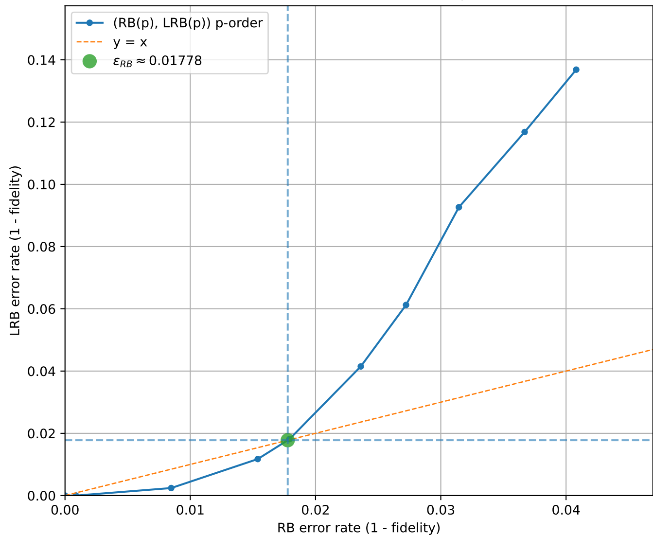
LRB vs RB (uniform interval check = 16, q=3 , [[5, 1, 2]]_3 )
