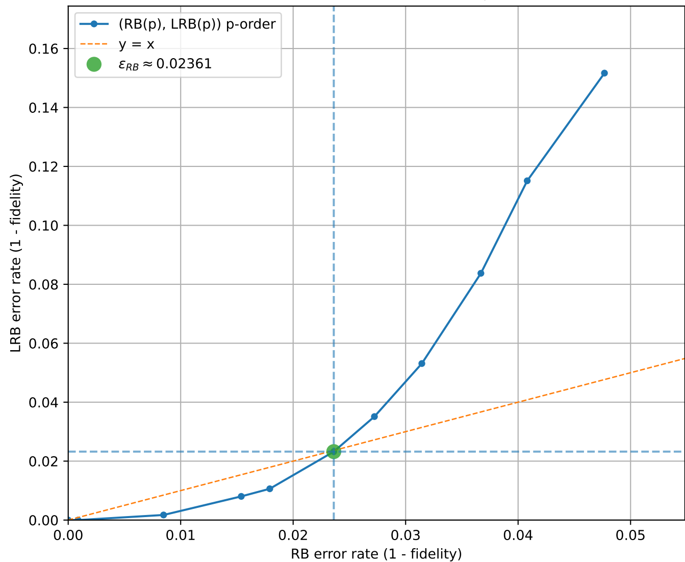
LRB vs RB (uniform interval check = 10, q=3 , [[5, 1, 2]]_3 )
