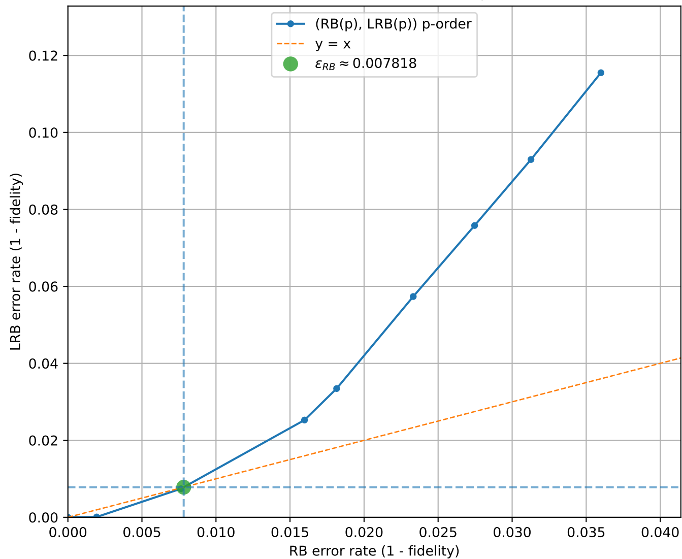
LRB vs RB (uniform interval check = 18, q=3 , [[3, 1, 2]]_3 )
