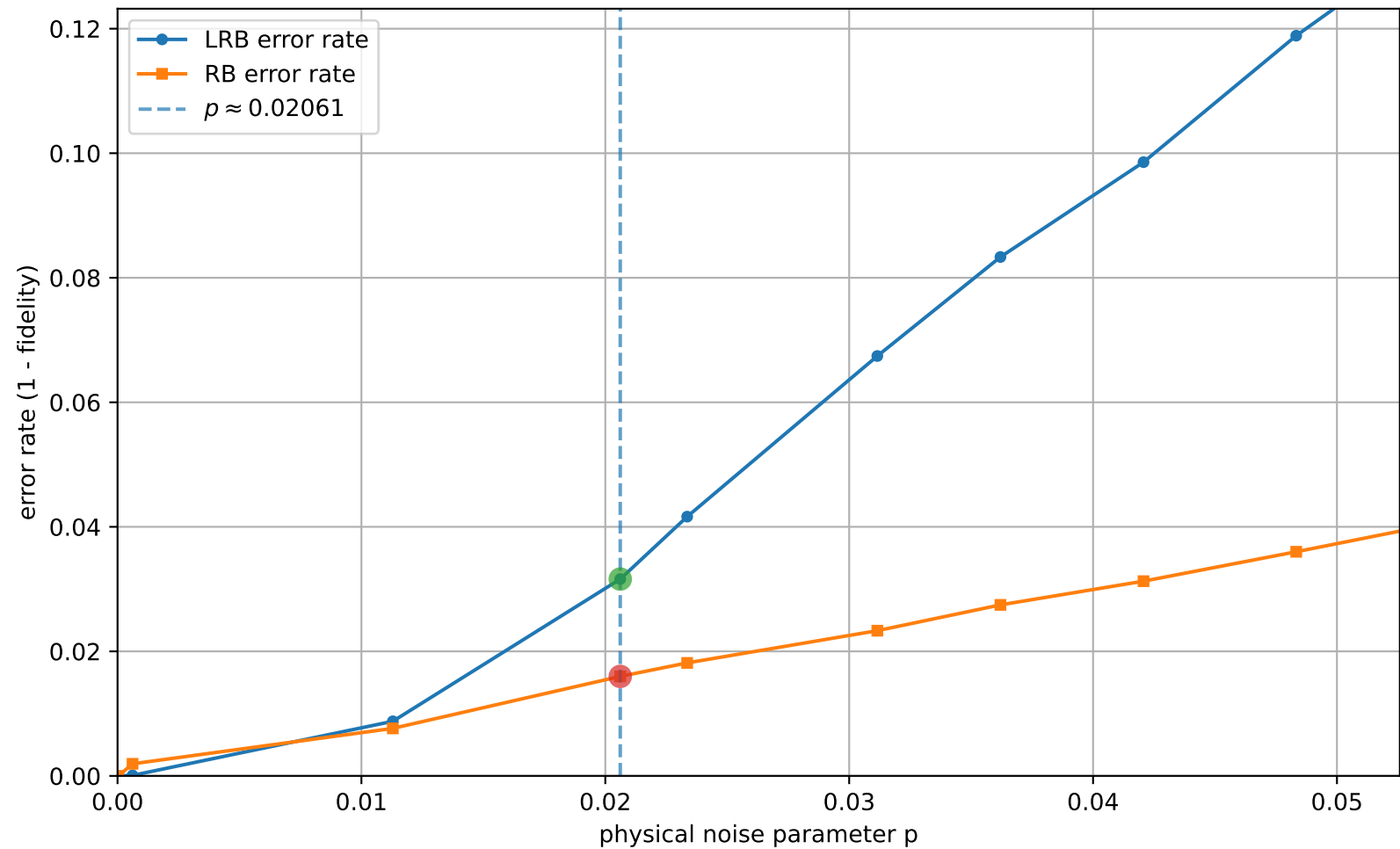
LRB vs RB (uniform interval check = 22, q=3, [[3, 1, 2]]_3 ): error rates vs p
