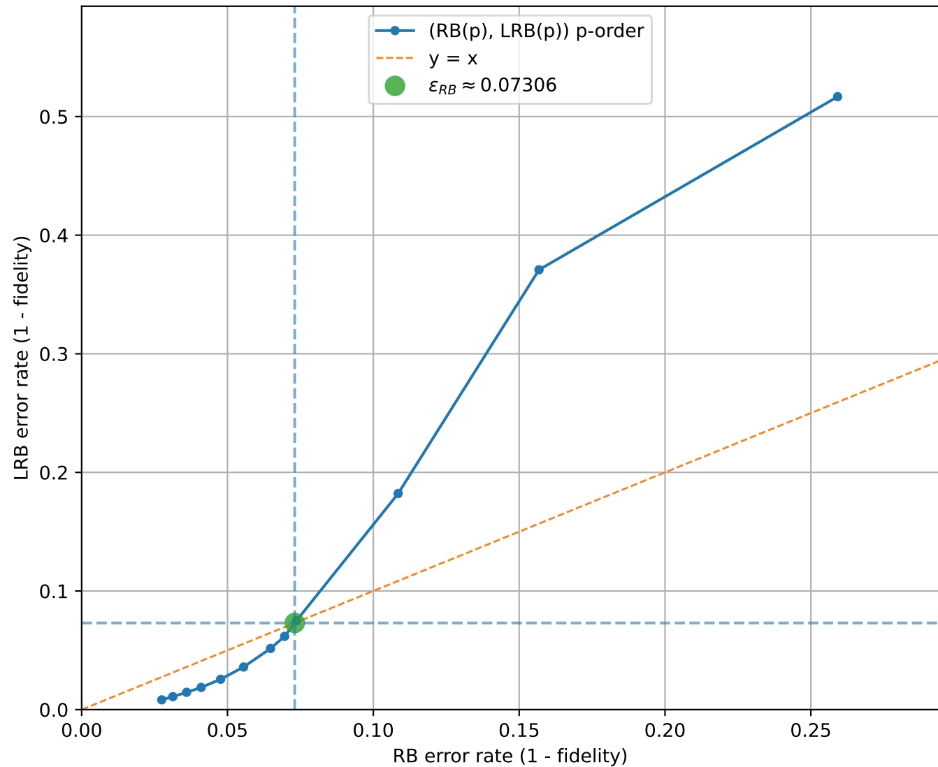
LRB vs RB (uniform interval check = 2, q=3 , [[3, 1, 2]]_3 ): p-window around threshold
