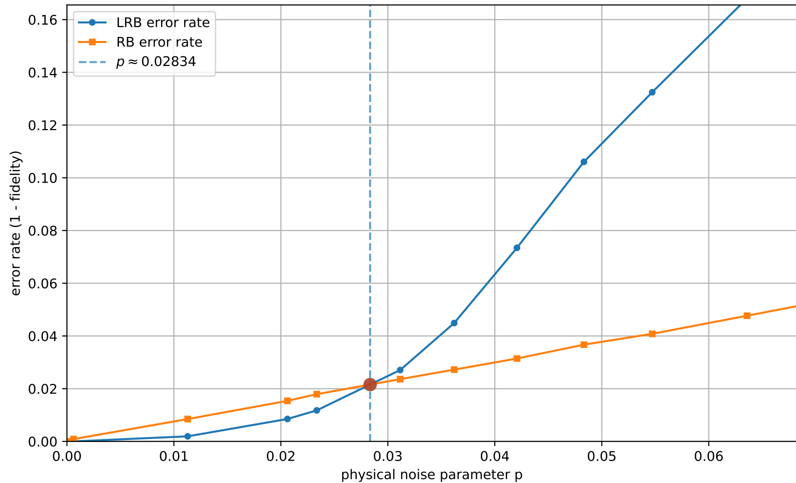
LRB vs RB (uniform interval check = 11, q=3, [[5, 1, 2]]_3 ): error rates vs p
