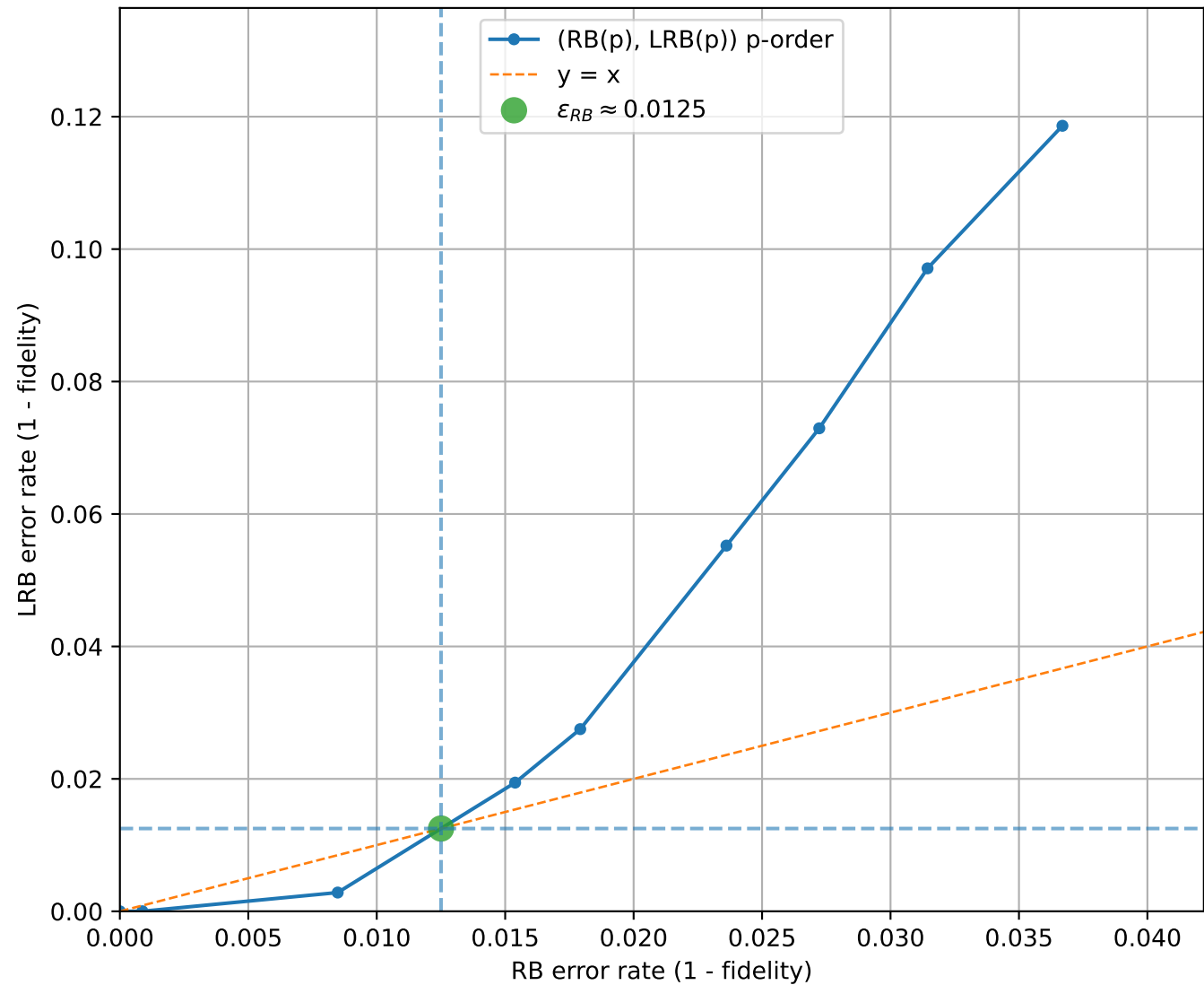
LRB vs RB (uniform interval check = 20, q=3 , [[5, 1, 2]]_3 )
