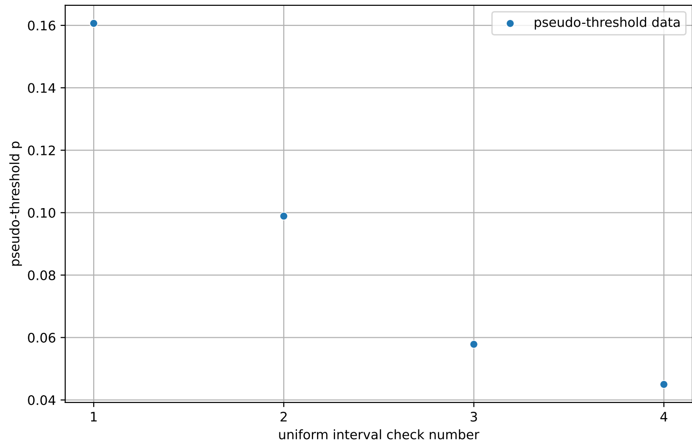
Pseudo-threshold vs uniform interval check (q=3, [[3, 1, 2]]_3 )
