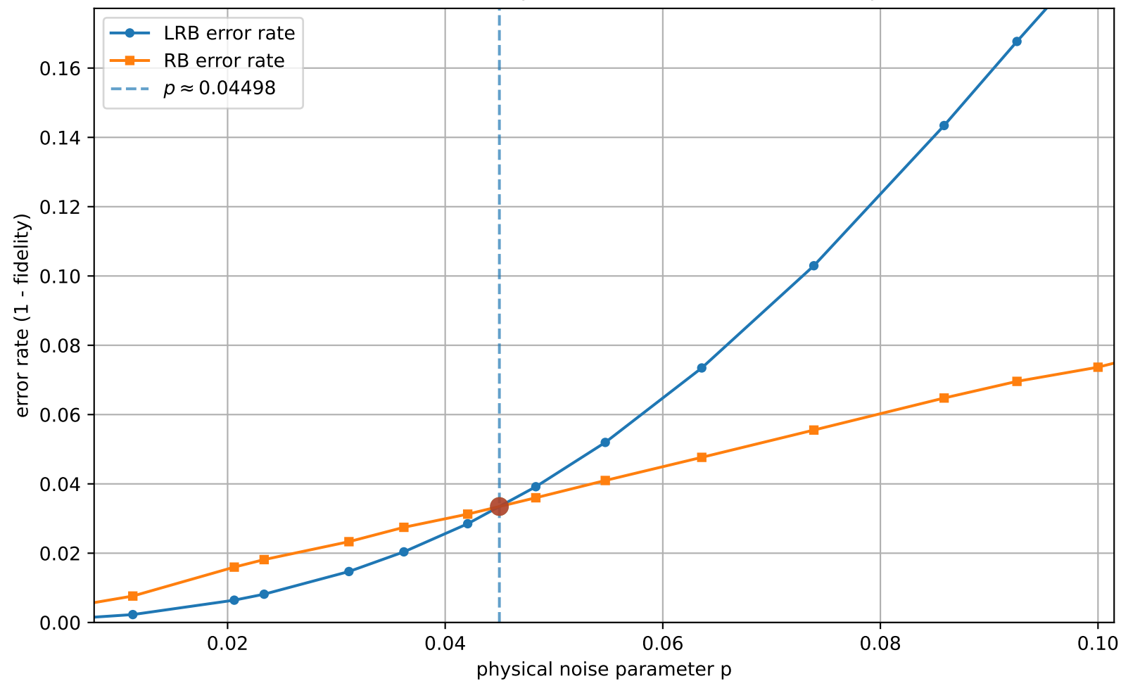
LRB vs RB (uniform interval check = 4, q=3 , [[3, 1, 2]]_3 ): error rates vs p (zoom near threshold)
