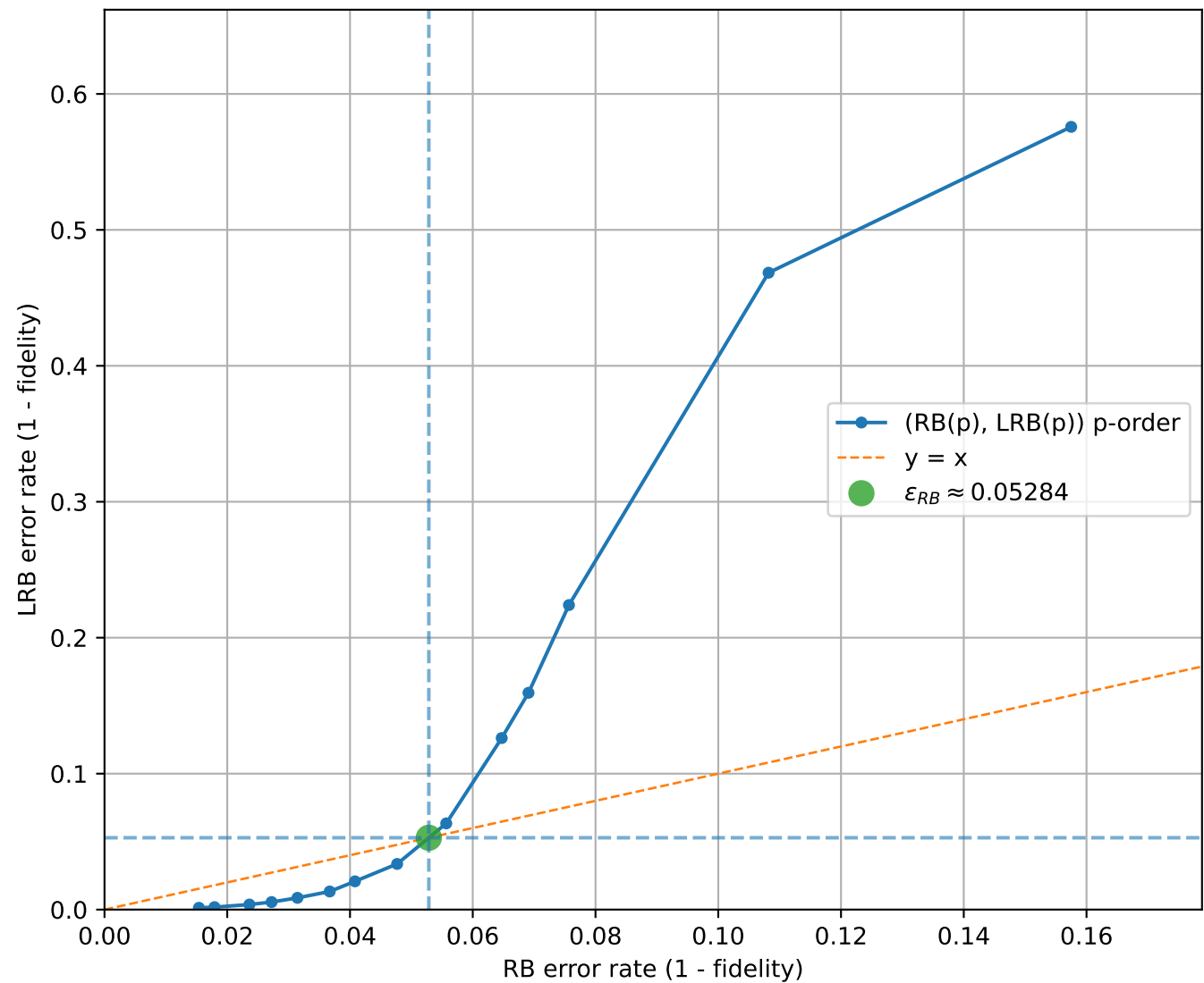
LRB vs RB (uniform interval check = 3, q=3 , [[5, 1, 2]]_3 )
