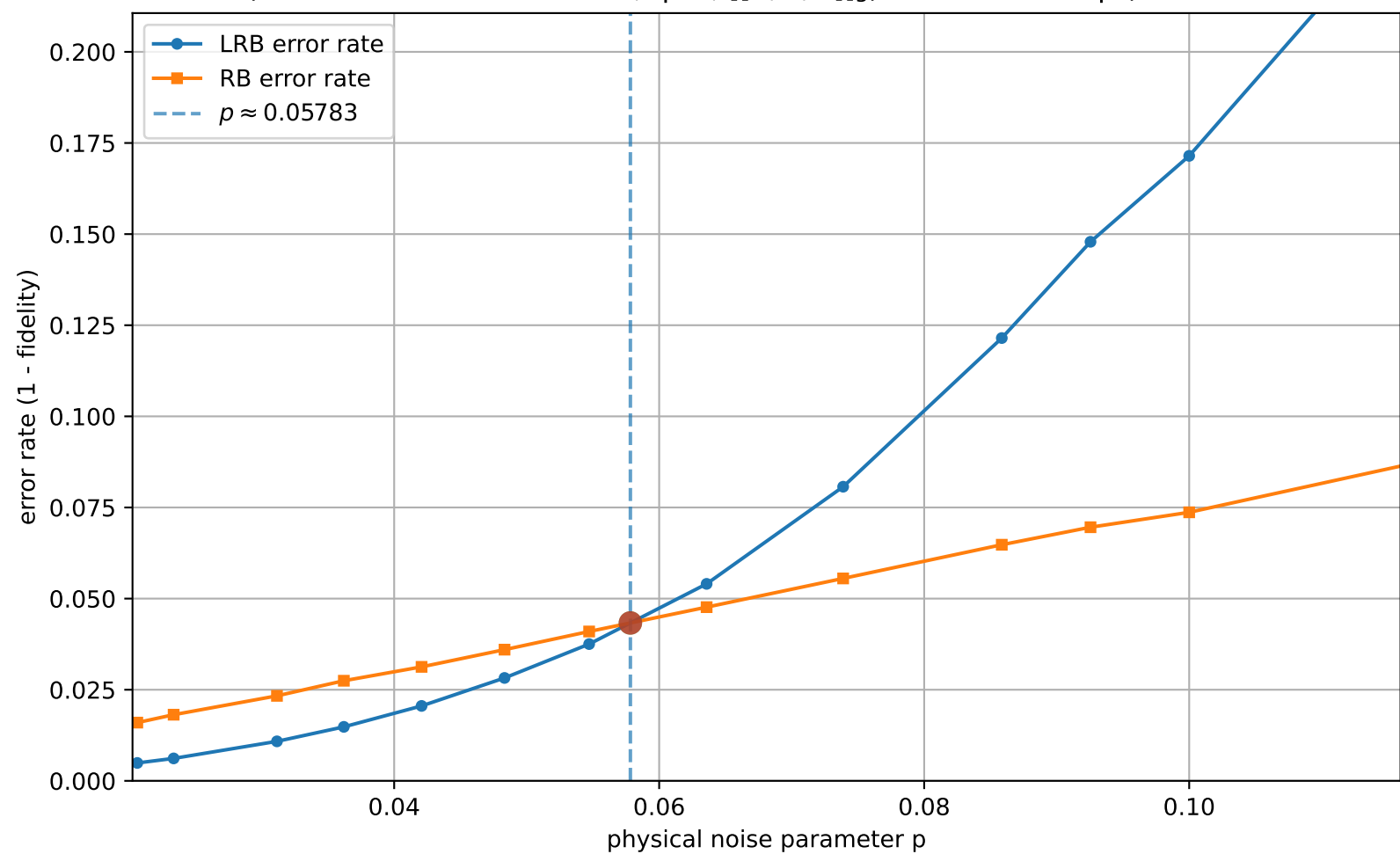
LRB vs RB (uniform interval check = 3, q=3 , [[3, 1, 2]]_3 ): error rates vs p (zoom near threshold)
