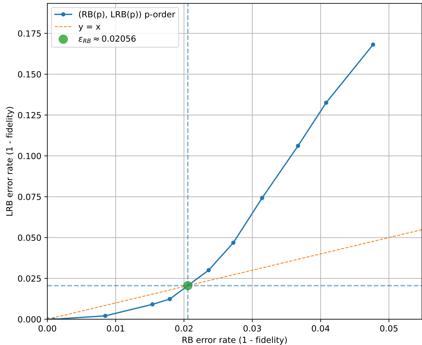
LRB vs RB (uniform interval check = 12, q=3 , [[5, 1, 2]]_3 )
