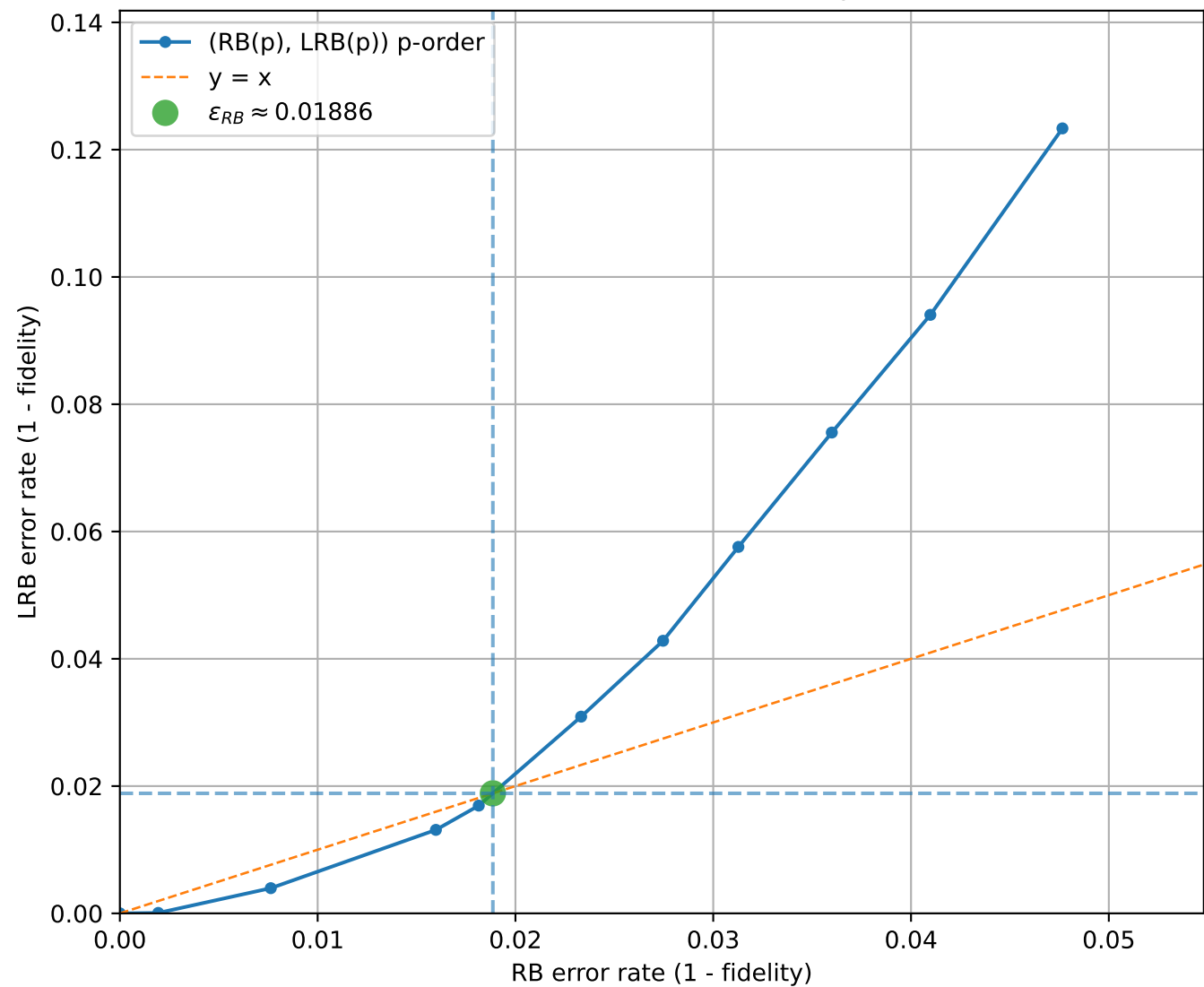
LRB vs RB (uniform interval check = 8, q=3 , [[3, 1, 2]]_3 )
