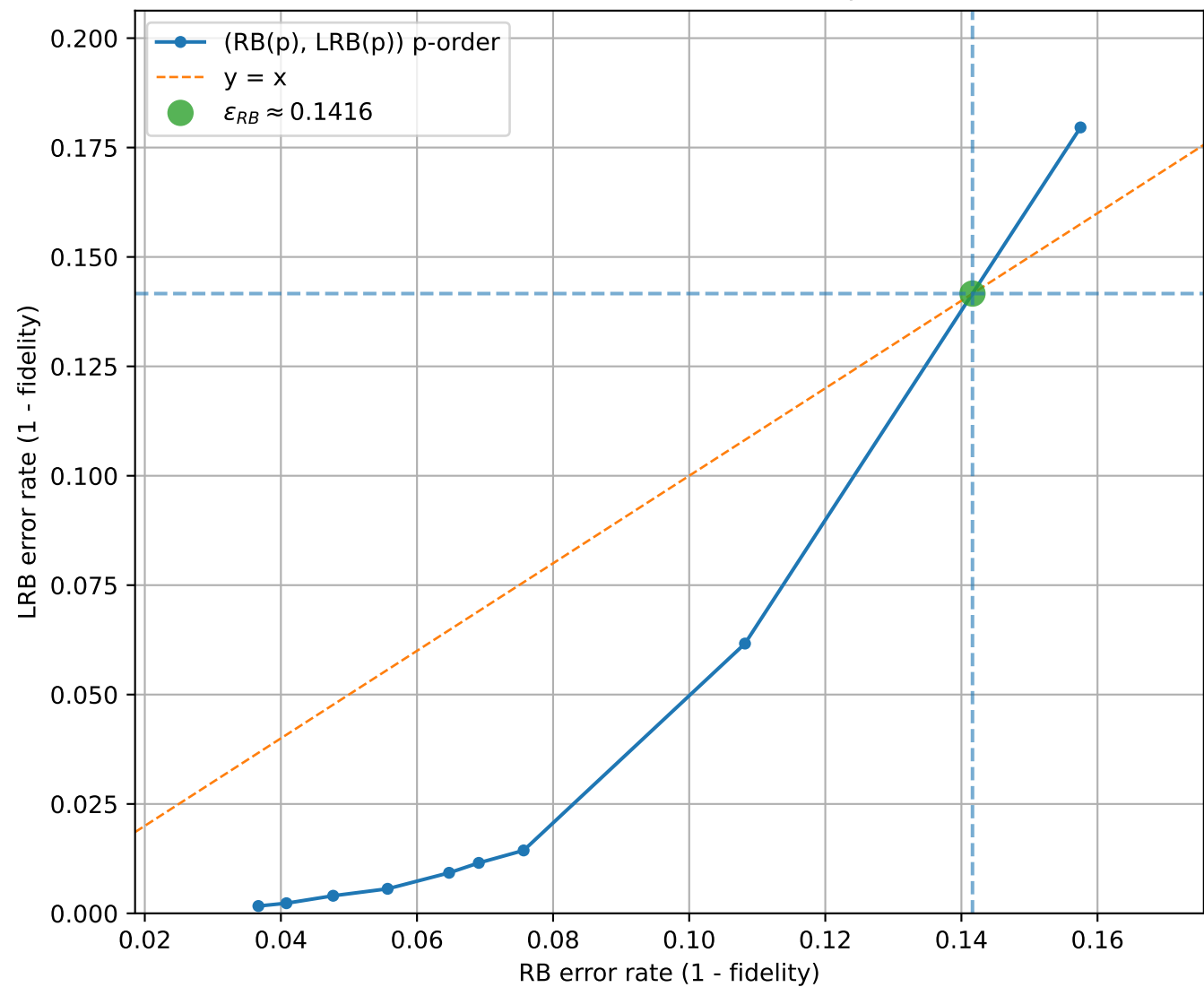
LRB vs RB (uniform interval check = 1, q=3 , [[5, 1, 2]]_3 )
