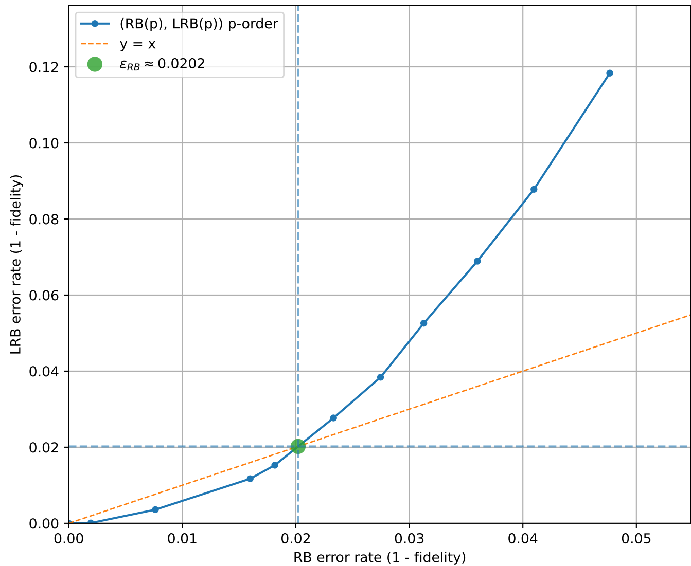
LRB vs RB (uniform interval check = 7, q=3, [[3, 1, 2]]_3 )
