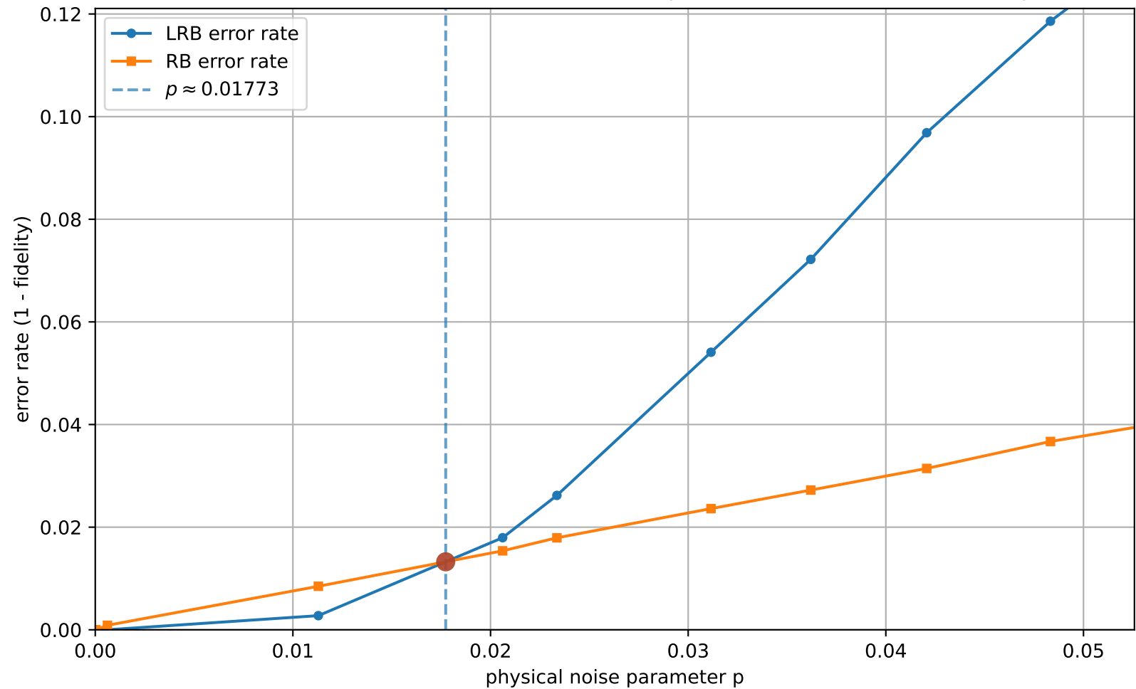
LRB vs RB (uniform interval check = 19, q=3 , [[5, 1, 2]]_3 ): error rates vs p
