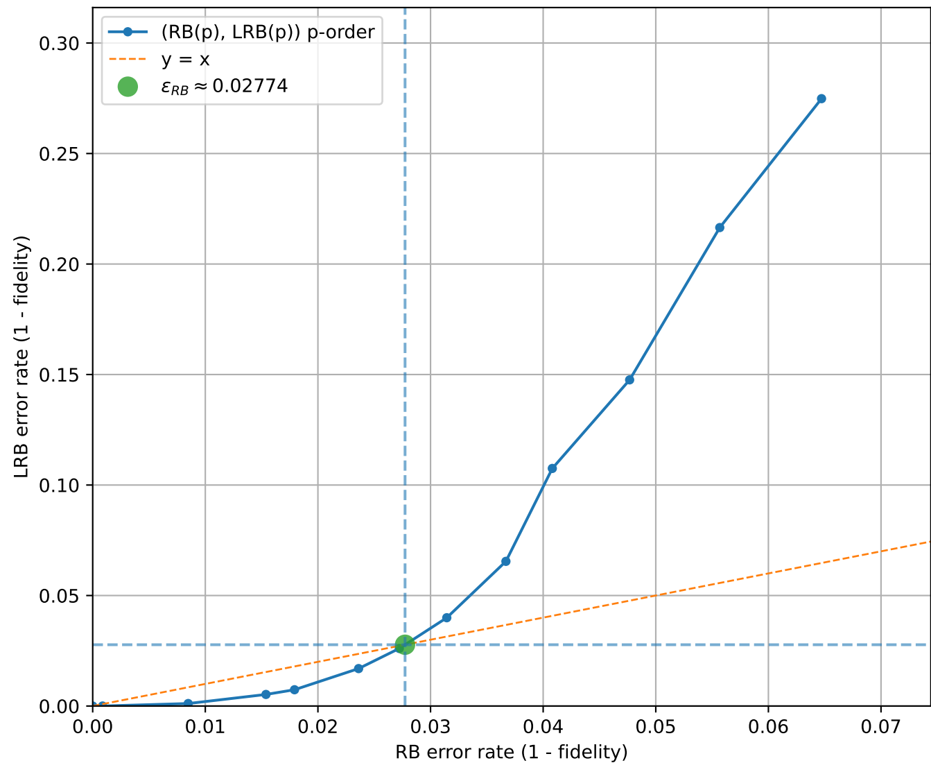
LRB vs RB (uniform interval check = 7, q=3, [[5, 1, 2]]_3 )
