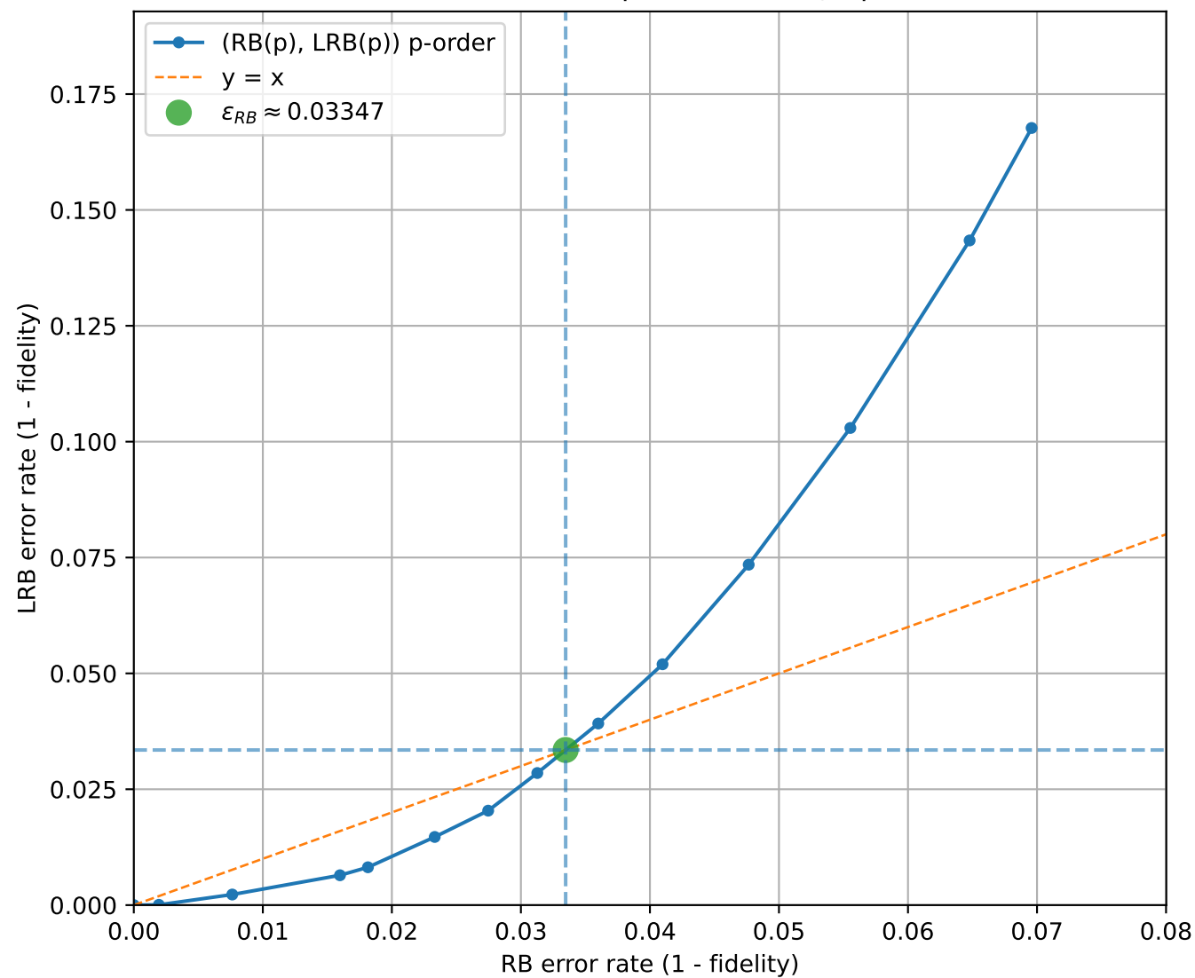
LRB vs RB (uniform interval check = 4, q=3 , [[3, 1, 2]]_3 ): p-window around threshold
