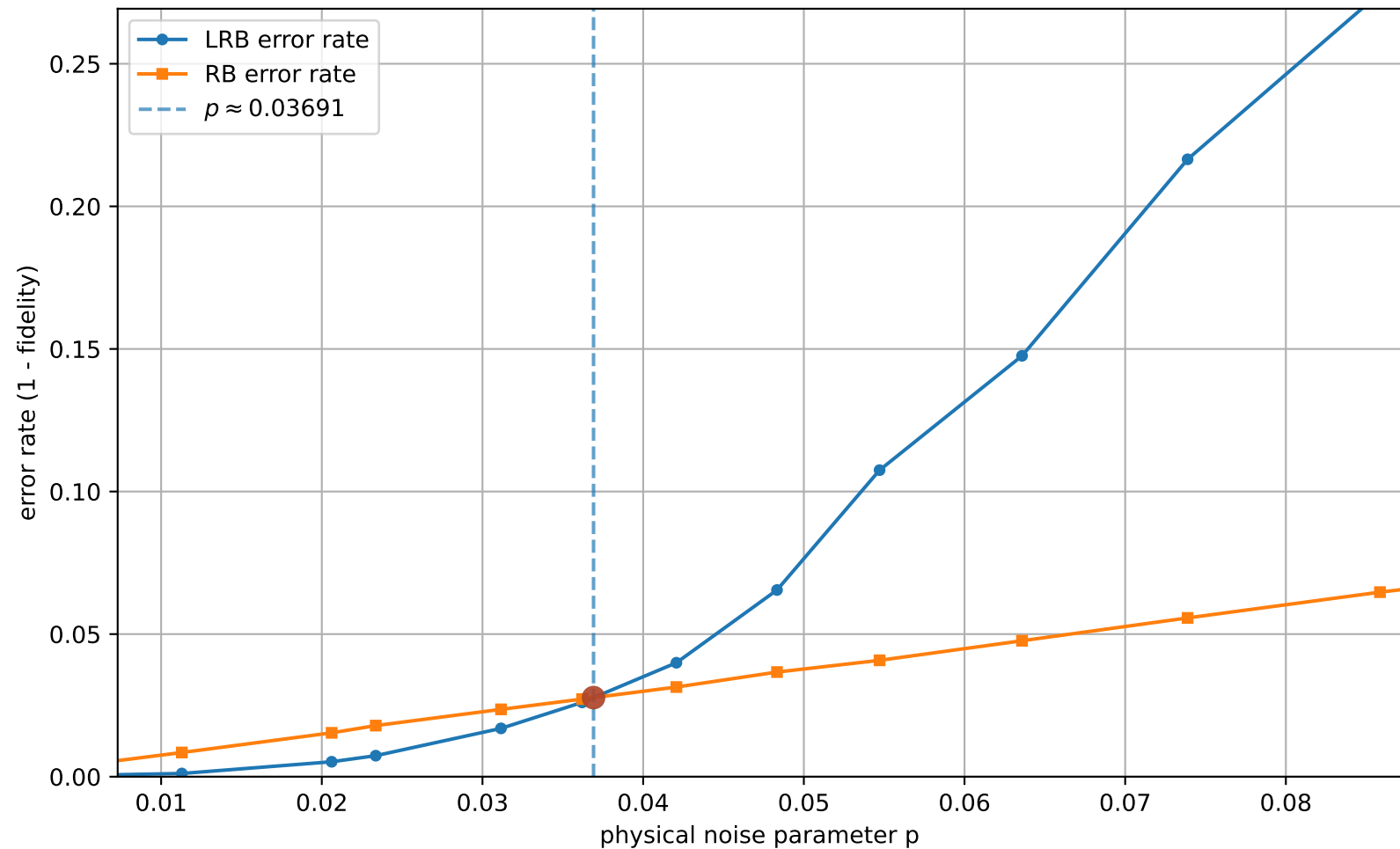
LRB vs RB (uniform interval check = 7, q=3 , [[5, 1, 2]]_3 ): error rates vs p
