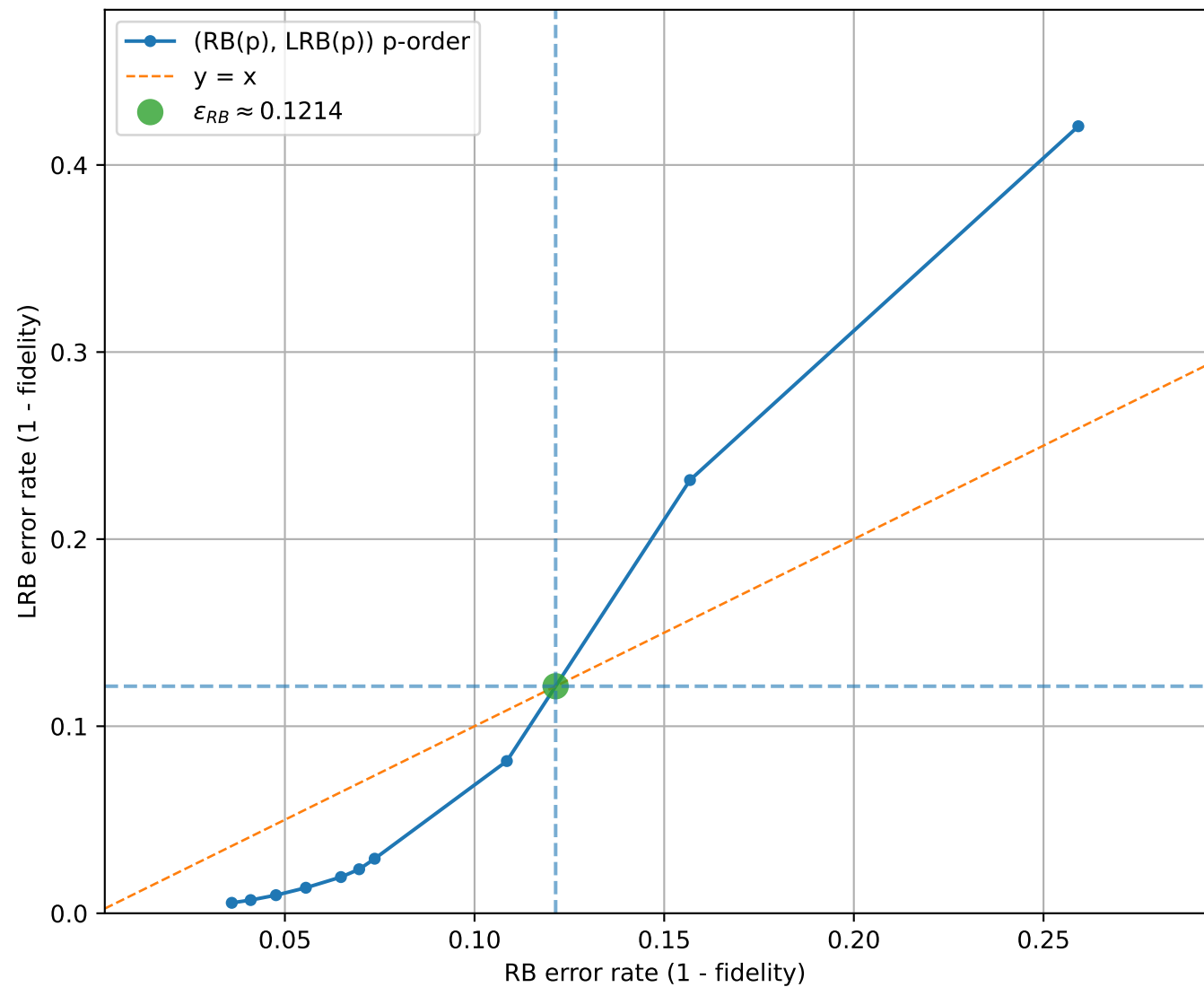
LRB vs RB (uniform interval check = 1, q=3 , [[3, 1, 2]]_3 ): p-window around threshold
