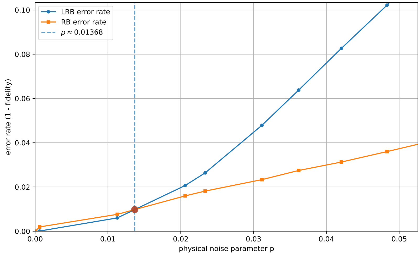
LRB vs RB (uniform interval check = 14, q=3, [[3, 1, 2]]_3 ): error rates vs p
