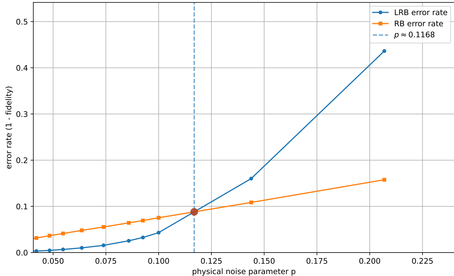
unif=2: error rates vs p (zoom near threshold)
