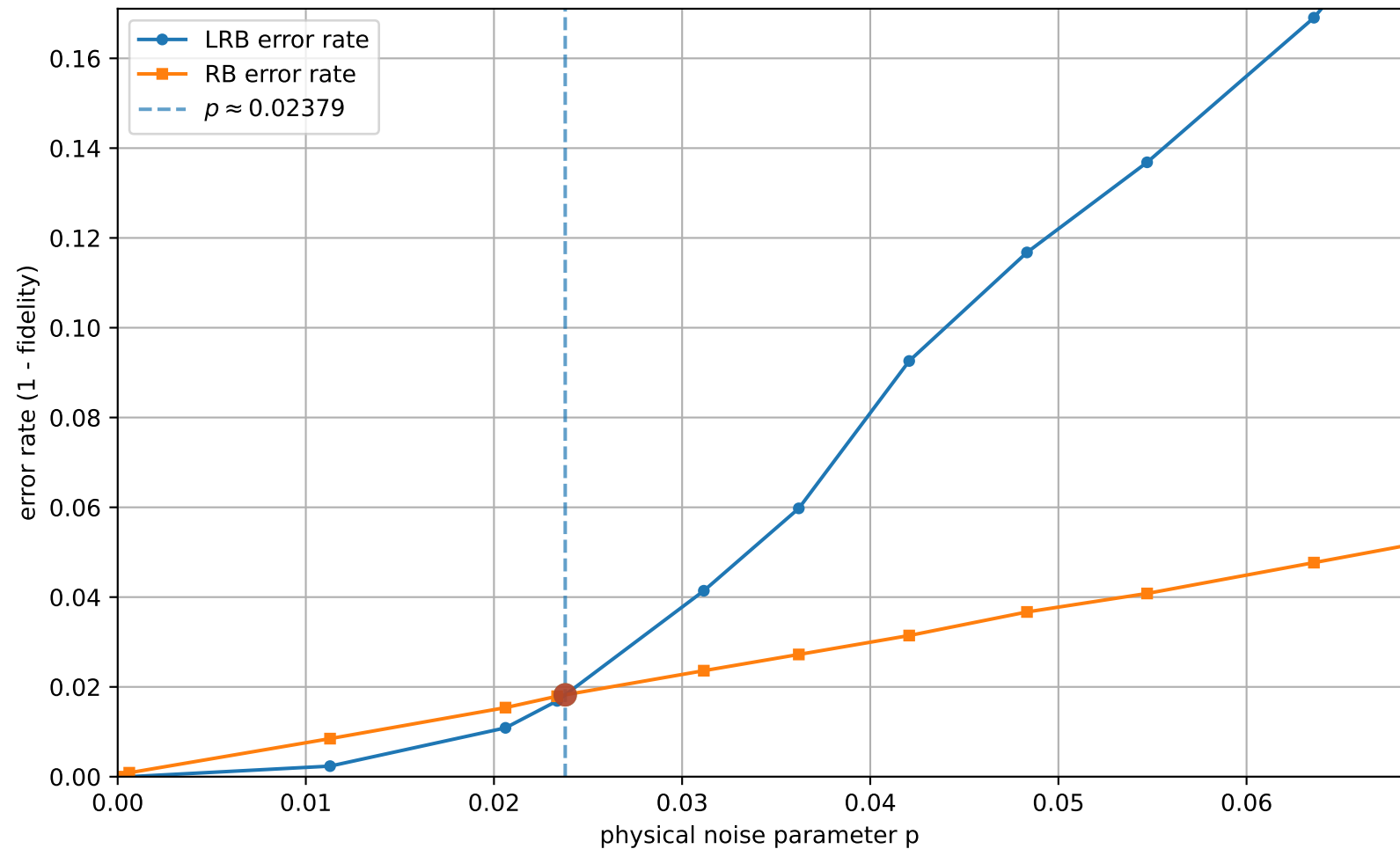
LRB vs RB (uniform interval check = 15, q=3 , [[5, 1, 2]]_3 ): error rates vs p
