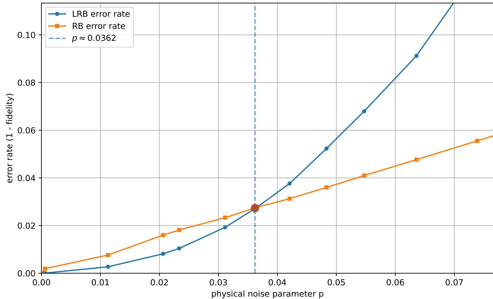
LRB vs RB (uniform interval check = 5, q=3, [[3, 1, 2]]_3 ): error rates vs p
