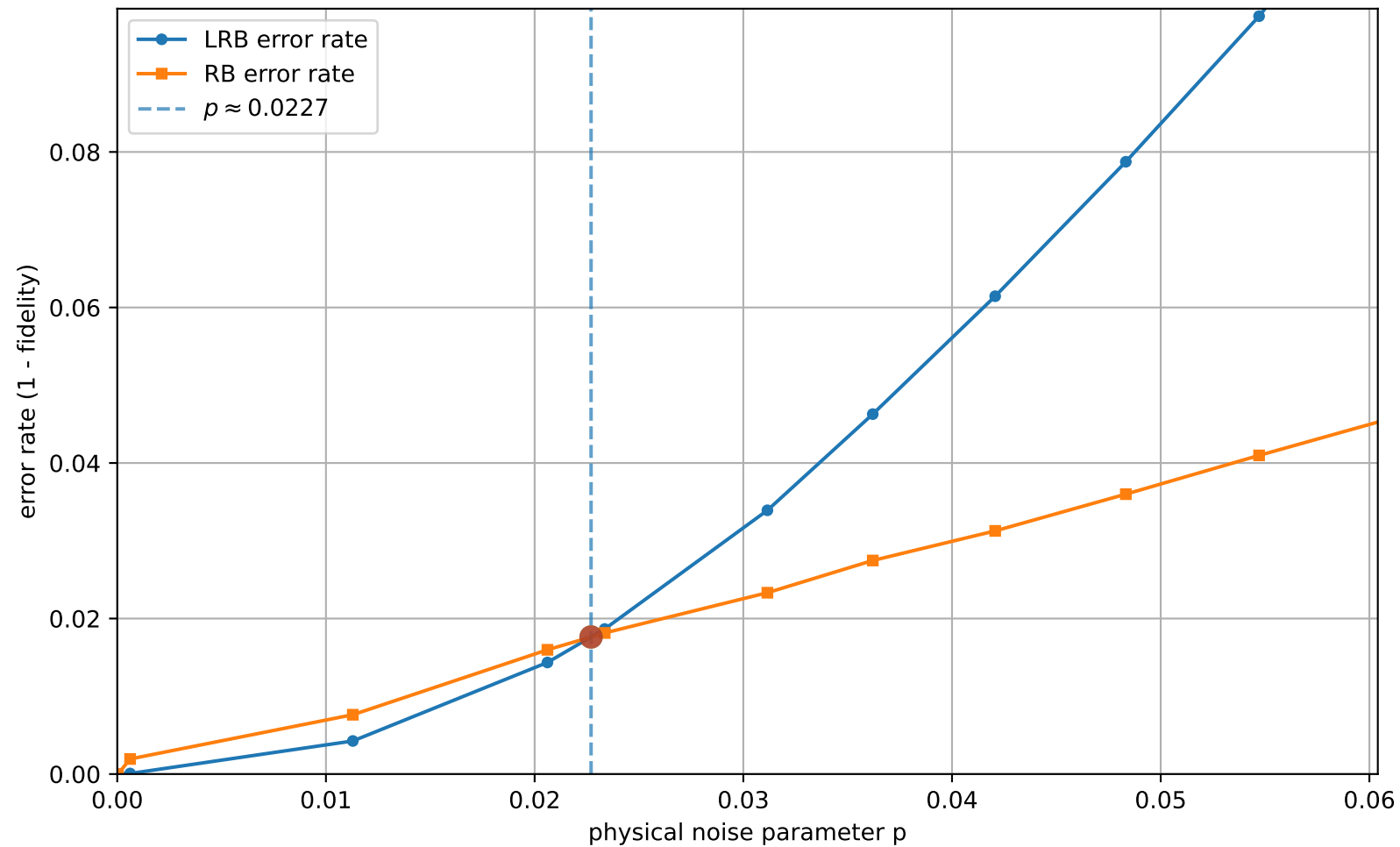
LRB vs RB (uniform interval check = 9, q=3 , [[3, 1, 2]]_3 ): error rates vs p
