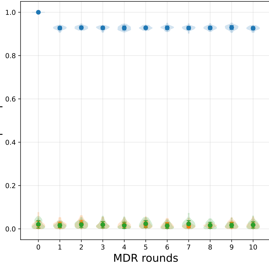
Unbiased Depolarizing Noise
