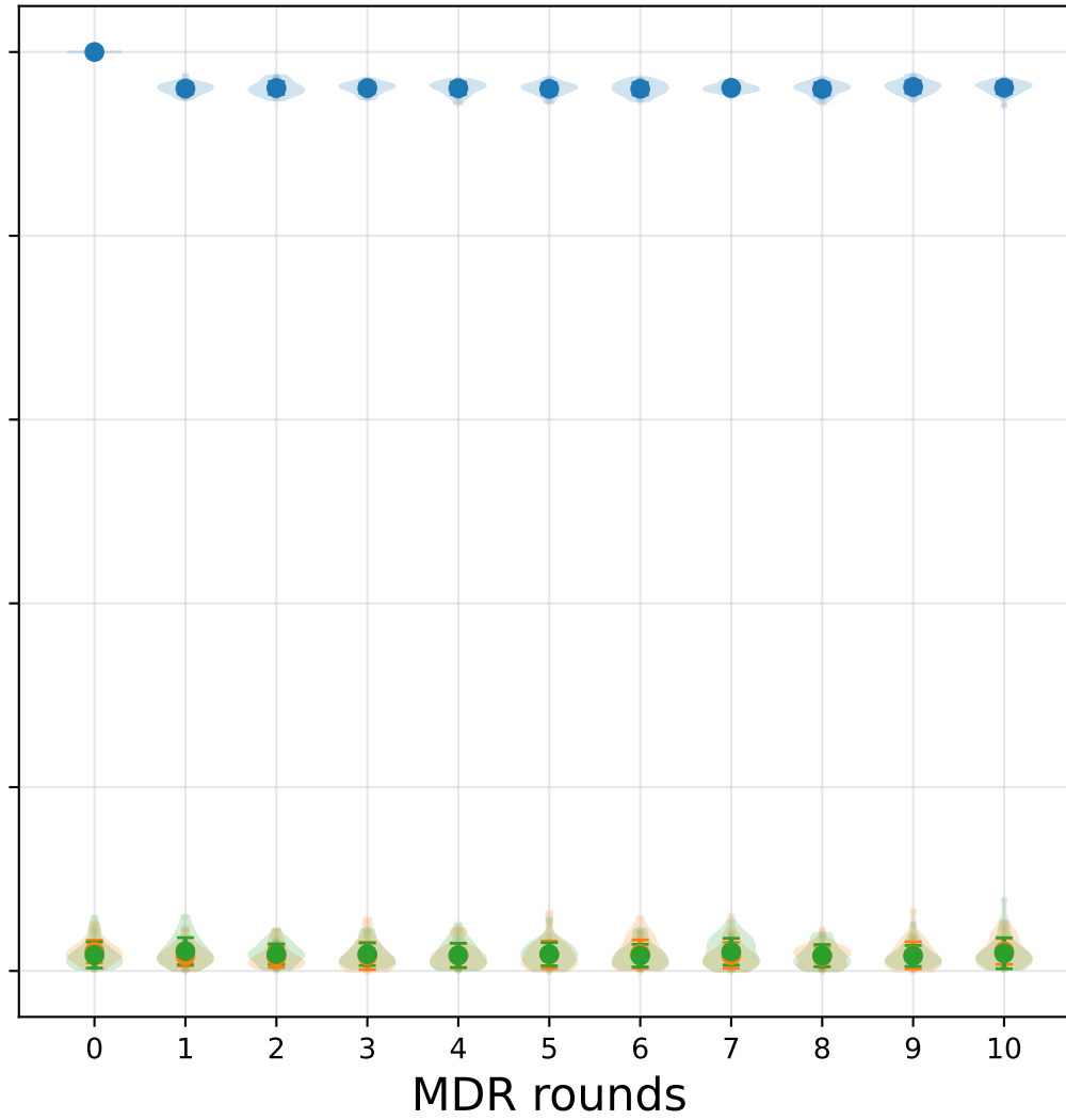
Z Type Noise
