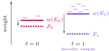
(c) Free-energy comparison
