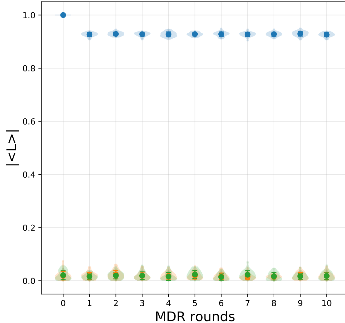
Unbiased Depolarizing Noise
