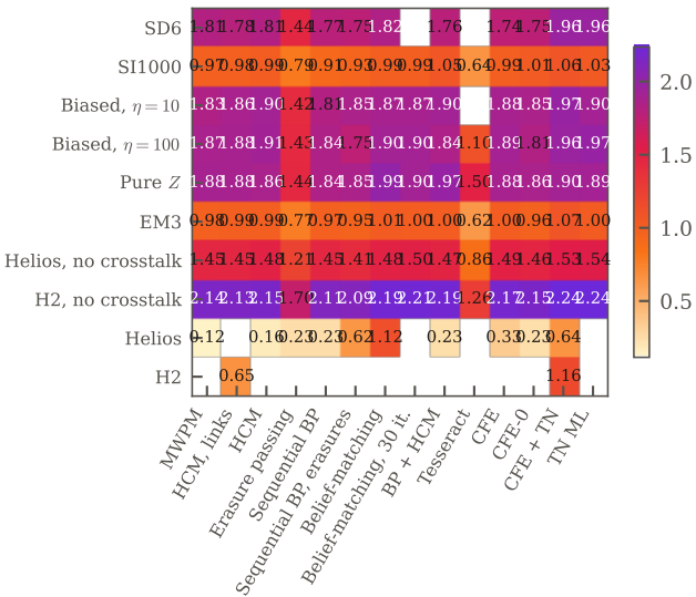
r = 1 , threshold (%)
