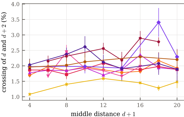
r = 1 , Biased, \eta = 10
