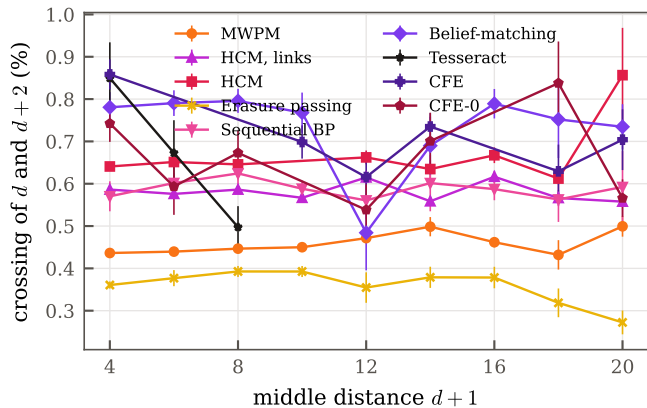
r = d , Biased, \eta = 10
