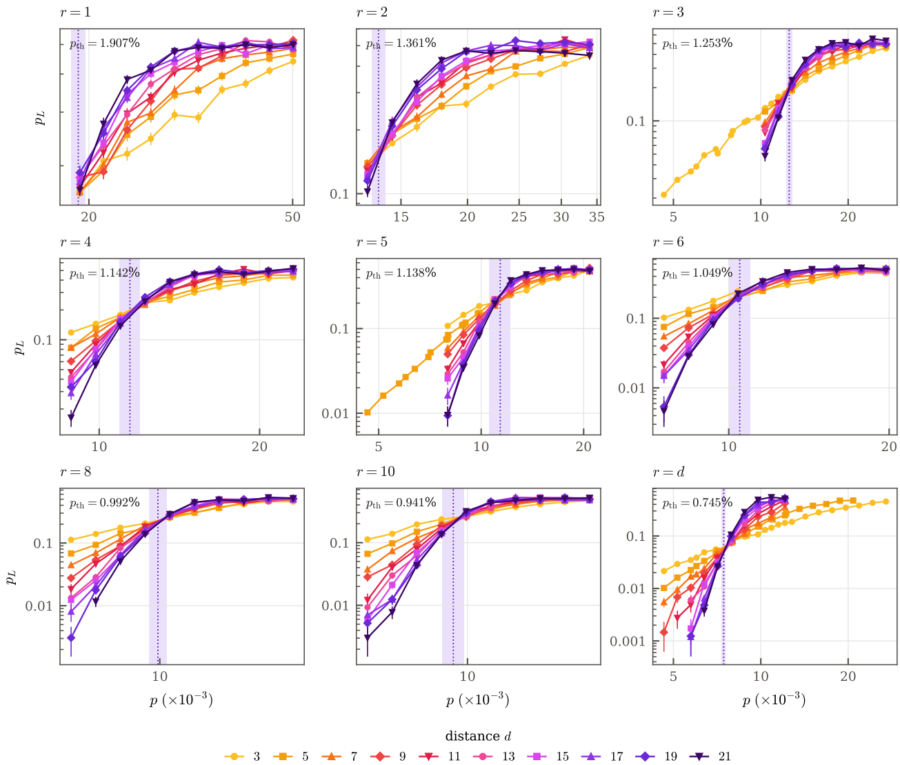
Biased, \eta = 10 , Belief-matching
