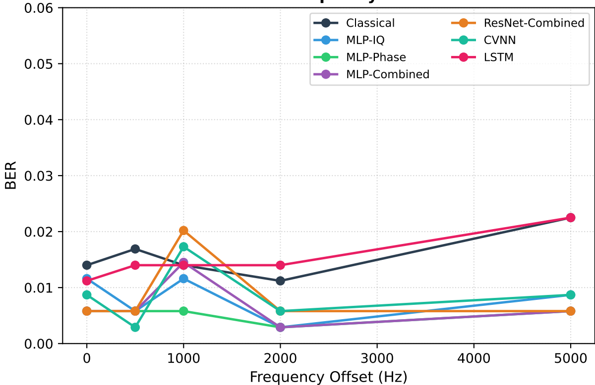
BER vs Frequency Offset
