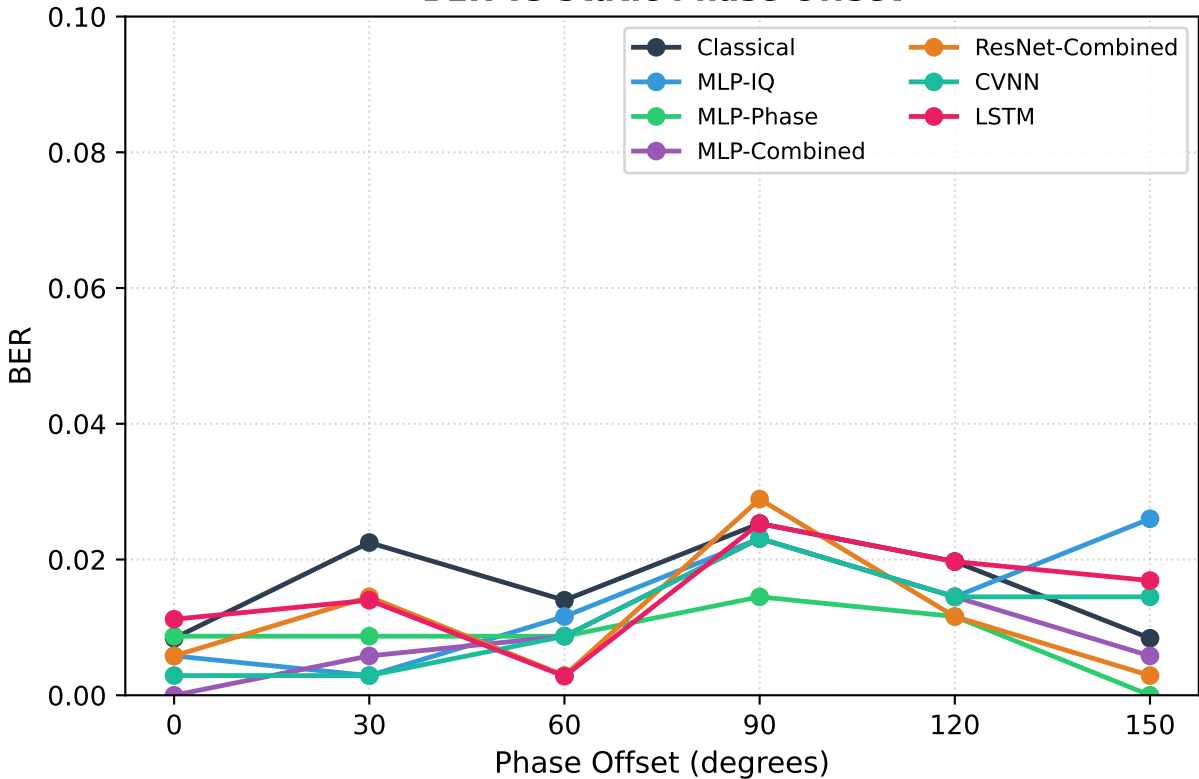
BER vs Static Phase Offset
