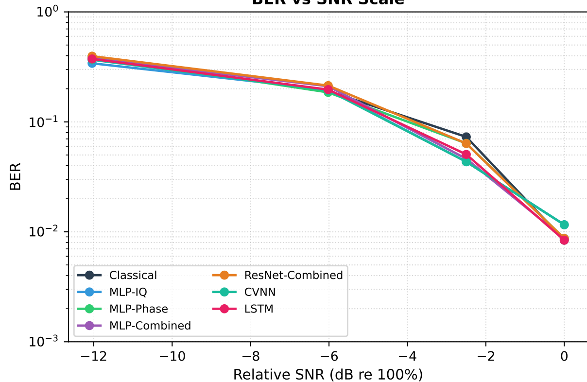
BER vs SNR Scale
