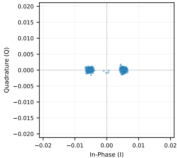
Freq offset 5 kHz
