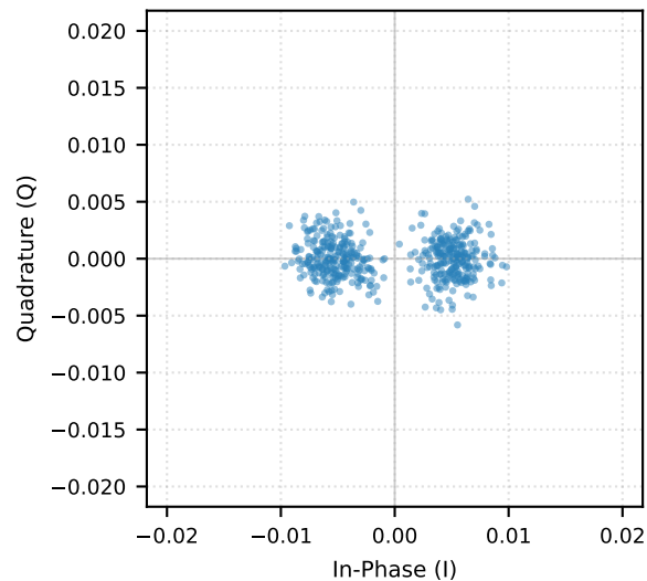
IQ imbalance \alpha=0.7
