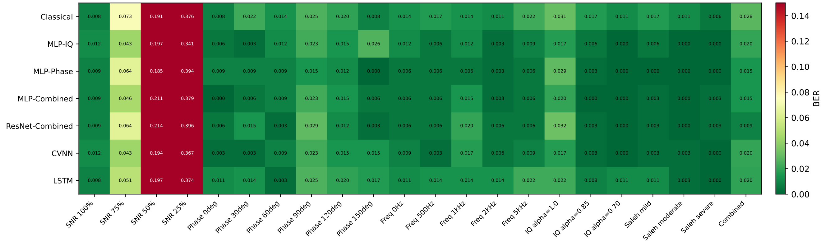
BER Heatmap — Green = Low Error, Red = High Error
