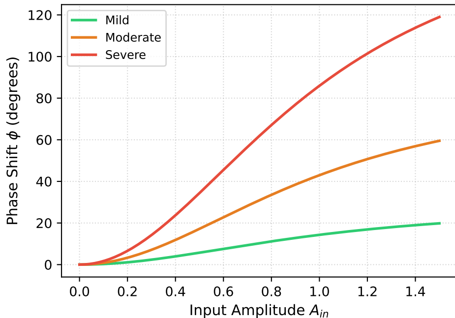
AM-PM Characteristic
