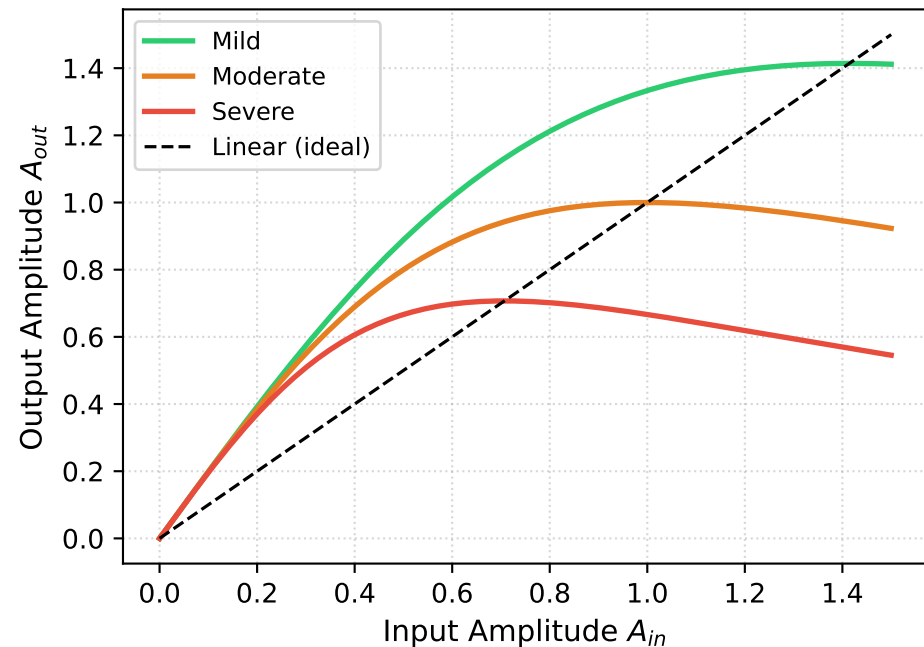
AM-AM Characteristic
