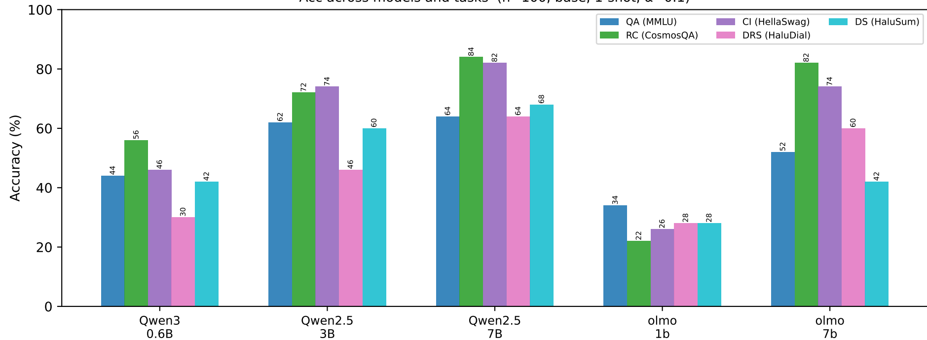
Acc across models and tasks (n=100, base, 1-shot, \alpha=0.1 )
