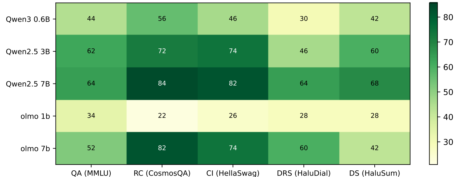
Acc heatmap — models × tasks (n=100, base, 1-shot, \alpha=0.1 )
