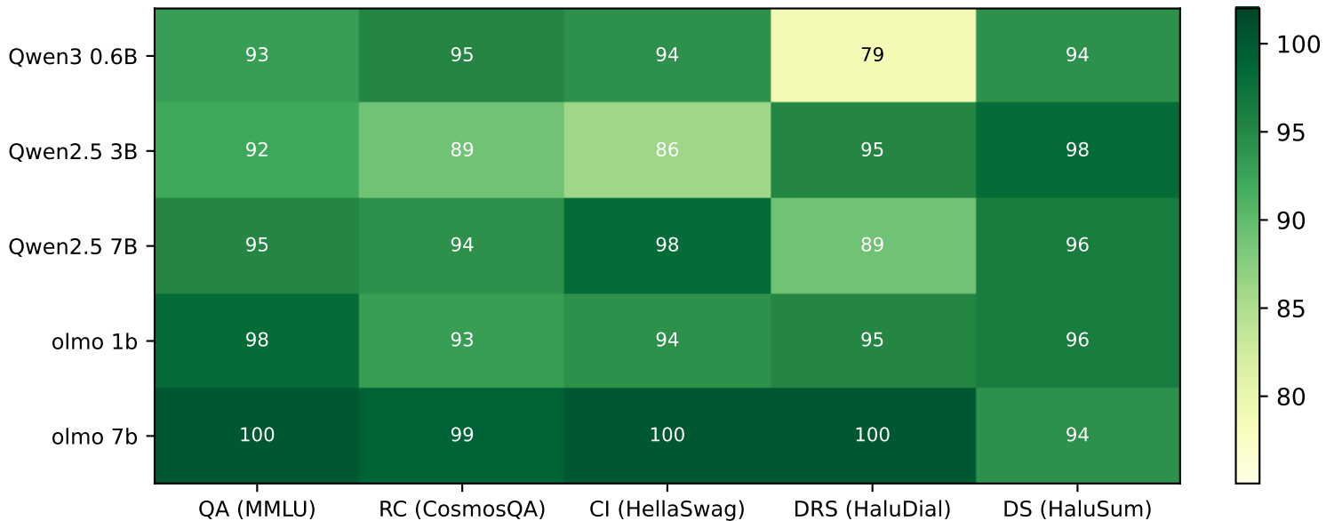
CR heatmap — models × tasks (n=100, base, 1-shot, \alpha=0.1 )
