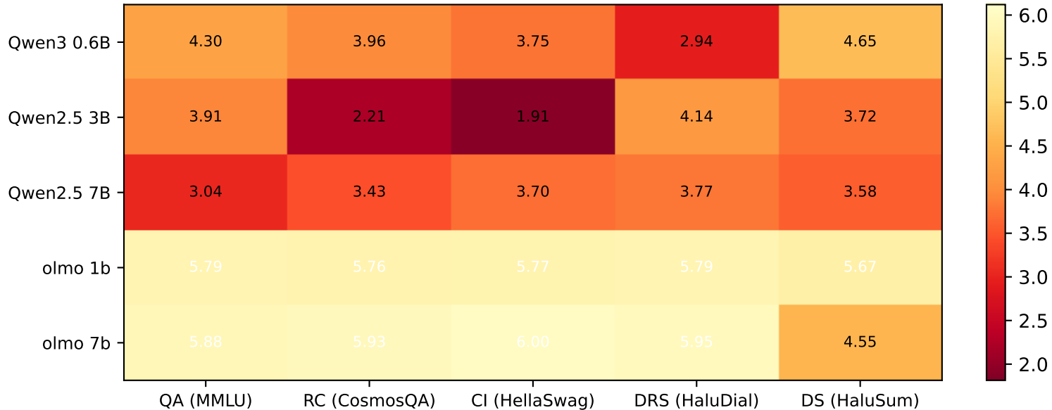
SS heatmap — models × tasks (n=100, base, 1-shot, \alpha=0.1 )
