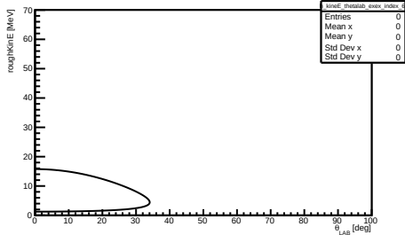
h_kineE_thetalab_exex_z_600--700
